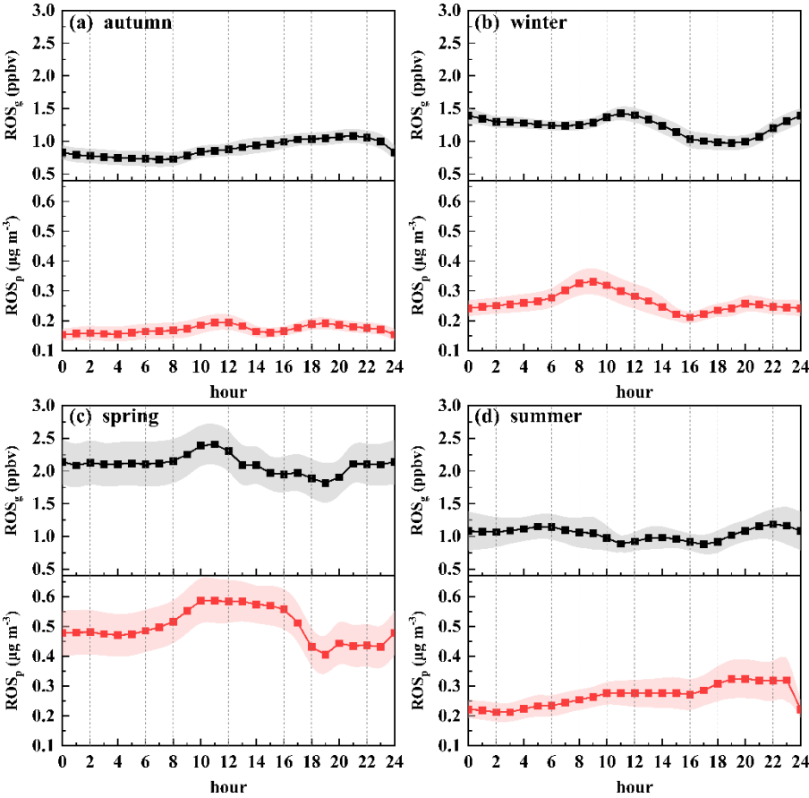
505 Figure 7. Seasonal diurnal profiles of \text{ROS}_g and \text{ROS}_p in clean days
