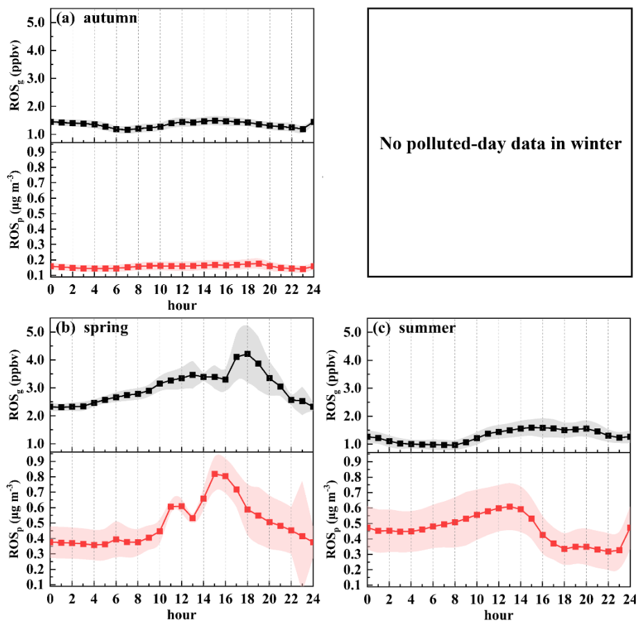
Figure 8. Seasonal diurnal profiles of ROS_g and ROS_p in polluted days
