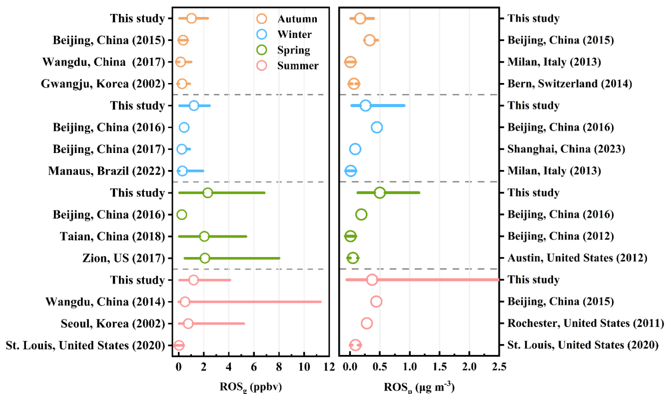
Figure 6. Comparison of seasonal mean ROS g and ROS p concentrations observed in this study with those reported in previous field observations from different regions. Circles denote mean values, and horizontal lines denote the corresponding concentration ranges. All concentrations are expressed as H 2 O 2 equivalents; literature data were converted to ppbv for ROS g and μg m -3 for ROS p where applicable. Detailed data sources are summarized in Table S3.
