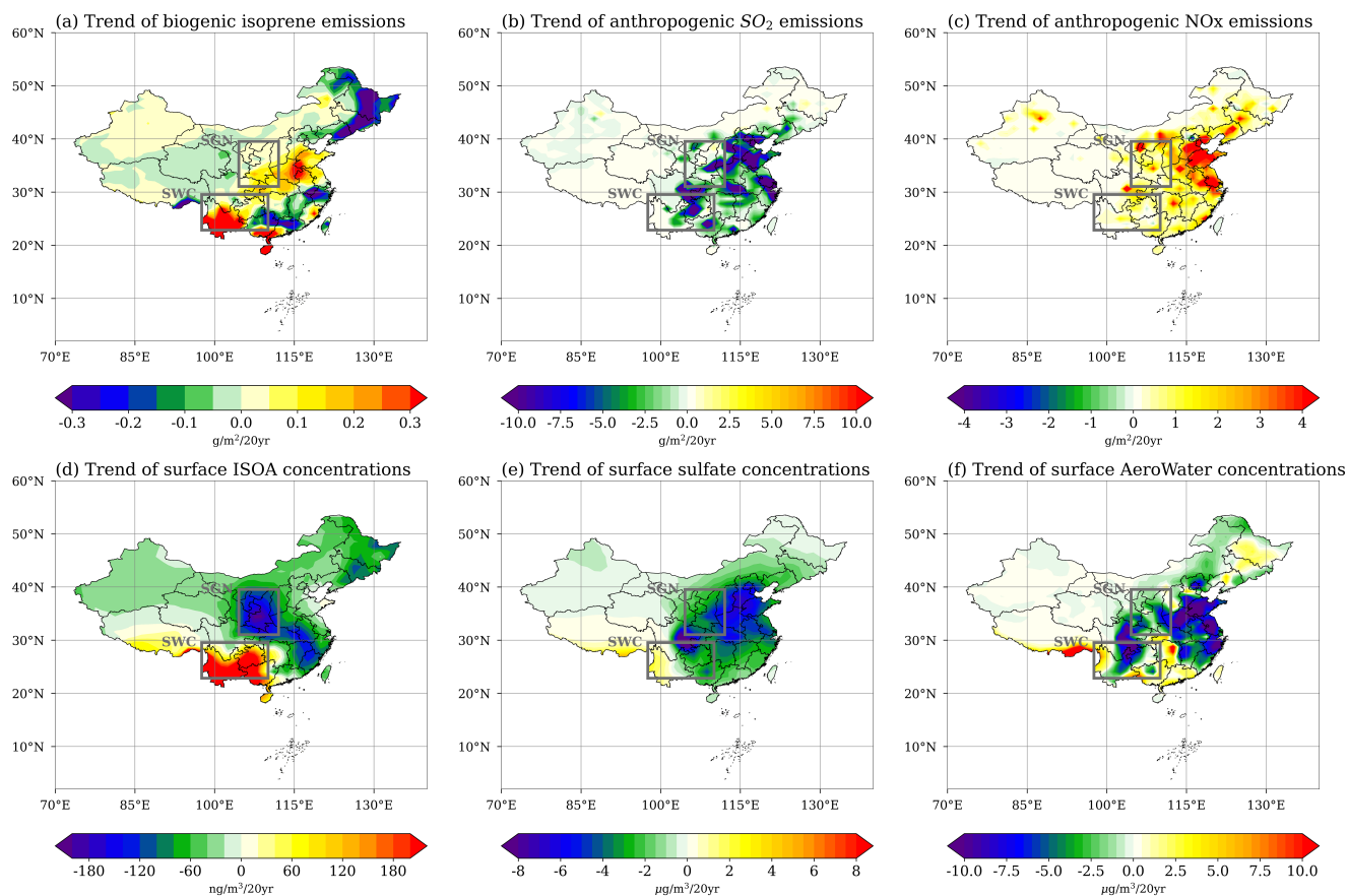
Figure 6: Long-term trends in annual mean surface concentrations of biogenic isoprene emissions (a; unit: \text{g m}^{-2} per 20 years), anthropogenic sulfur dioxide (SO 2 ) emissions (b; unit: \text{g m}^{-2} per 20 years), and anthropogenic nitrogen oxides (NO x ) emissions (c; unit: \text{g m}^{-2} per 20 years), and of surface isoprene-derived secondary organic aerosol (ISOA) concentrations (d; \text{ng m}^{-3} per 20 years), surface sulfate concentrations (e; \mu\text{g m}^{-3} per 20 years), and surface aerosol liquid water (AeroWater) concentrations (f; \mu\text{g m}^{-3} per 20 years), in China from 2000 to 2019. The two boxed regions denote Southwest China (SWC) and the Shaanxi-Gansu-Ningxia region (SGN), respectively.
