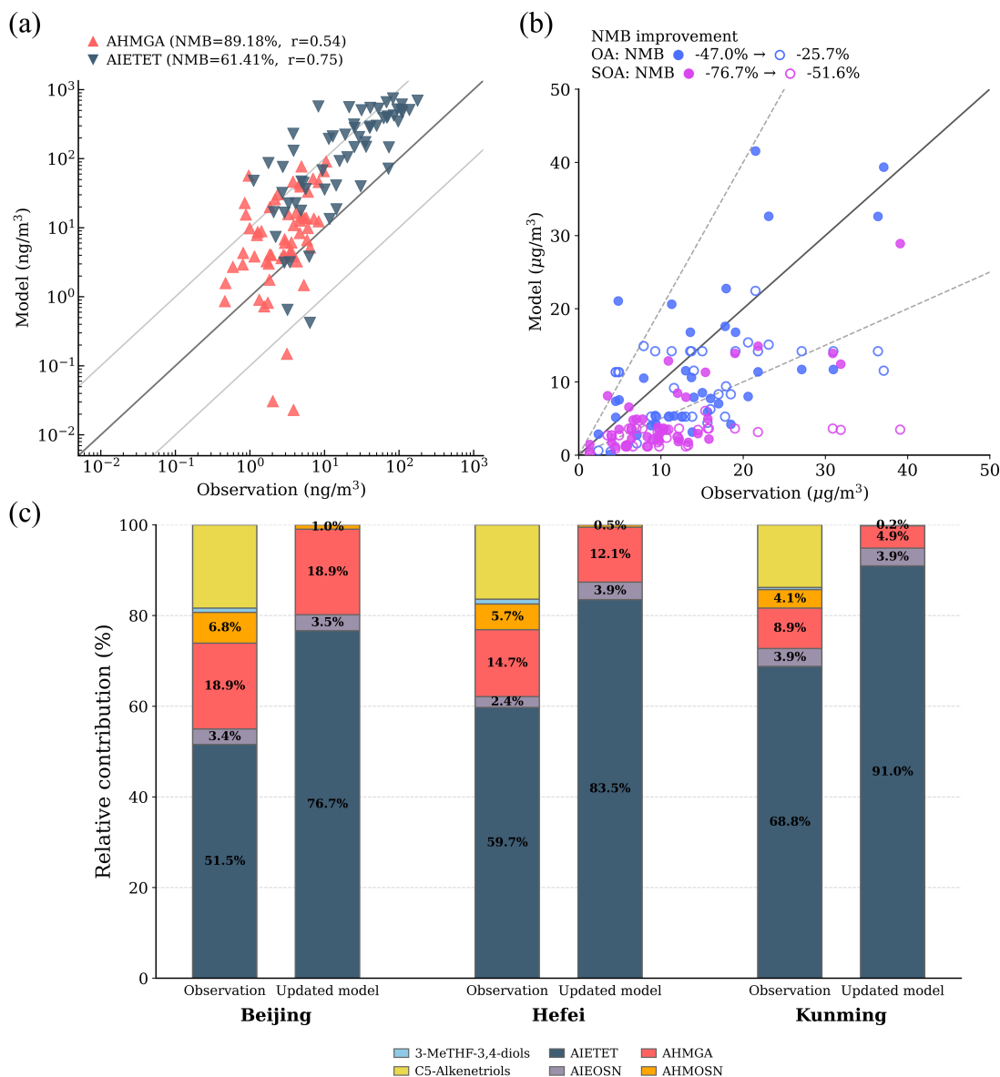
Figure 2: (a) Evaluation of simulated 2-methyltetrols (AIETET) and 2-methylglyceric acid (AHMGA) concentrations against ground-based observations from Ding et al. (2016) ( \text{ng m}^{-3} ). Statistical metrics were calculated using monthly means in log space. The dark gray solid line denotes the 1:1 line, and the light gray solid lines denote the factor-of-10 range. (b) Evaluation of simulated organic aerosol (OA) and secondary organic aerosol (SOA) concentrations before and after the mechanism update against ground-based observations compiled from Miao et al. (2021) and Chen et al. (2024a) ( \mu\text{g m}^{-3} ). Filled circles represent simulations before the update, while open circles represent simulations after the update. Blue and magenta markers denote OA and SOA, respectively. The inset annotation summarizes the changes in normalized mean bias (NMB) from the original to the updated simulation. The dark gray solid line denotes the 1:1 line, and the light gray dashed lines denote the factor-of-two range. (c) Comparison of ISOA product composition between ground-based observations adapted from Zhang et al. (2022) and the updated model simulation in this study. The grouped stacked bars show the relative contribution of each ISOA product to total measured or simulated ISOA at Beijing, Hefei, and Kunming. For each city, the left bar represents the observed composition and the right bar represents the updated model.
