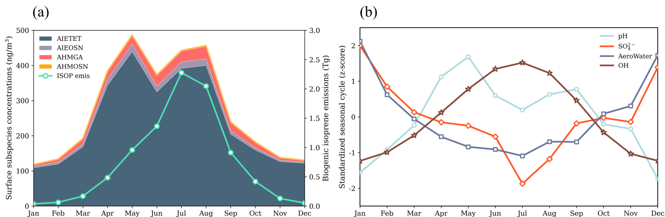
Figure 4: (a) Monthly variations of surface isoprene-derived secondary organic aerosol (ISOA) subspecies (left y axis; unit: ng m -3 ) and biogenic isoprene emissions (ISOP emis; right y axis; unit: Tg) in China, based on the climatological monthly means averaged over the five simulation years (2000, 2006, 2012, 2016, and 2019). (b) Standardized monthly variations of background chemical and aerosol variables relevant to ISOA formation, including surface aerosol pH, surface sulfate (SO 4 2- ) concentrations, surface aerosol liquid water (AeroWater) concentrations, and surface hydroxyl radical (OH) concentrations in China, based on the climatological monthly means averaged over the five simulation years.
