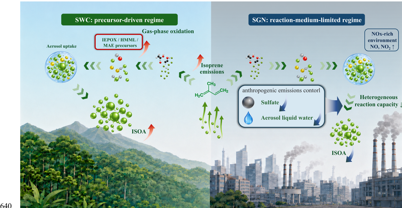
Figure 9. Schematic illustration of contrasting regional controls on surface isoprene-derived secondary organic aerosol (ISOA) formation in Southwest China (SWC; left) and the Shaanxi-Gansu-Ningxia region (SGN; right). The background scenes and selected graphical elements were created with the assistance of OpenAI's image-generation tools in ChatGPT (OpenAI, 2026).
