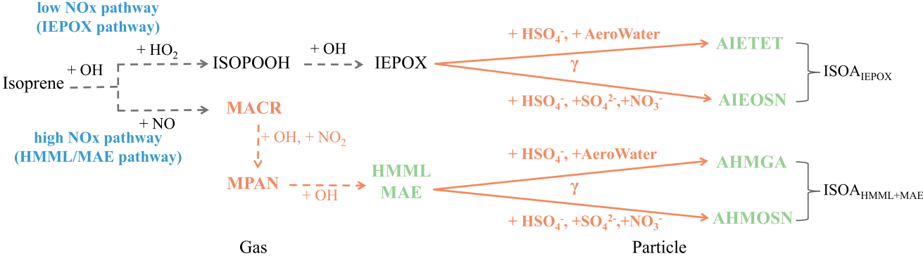
Figure 1: Schematic of the explicit isoprene-derived secondary organic aerosol (ISOA) formation mechanism implemented in CAM6-Chem in this study. Dashed arrows indicate gas-phase reactions, whereas solid arrows indicate particle-phase heterogeneous uptake and product-formation reactions. Species explicitly represented as updated ISOA precursors or product classes in this mechanism are shown in green, and the explicitly represented ISOA formation pathways are shown in orange. AeroWater denotes aerosol liquid water. AIIETET denotes IEPOX-derived 2-methyltetrols, AIIOSN denotes IEPOX-derived organosulfate/organonitrate products, AHMGA denotes HMML/MAE-derived 2-methylglyceric acid, and AHMOSN denotes HMML/MAE-derived organosulfate/organonitrate products.
