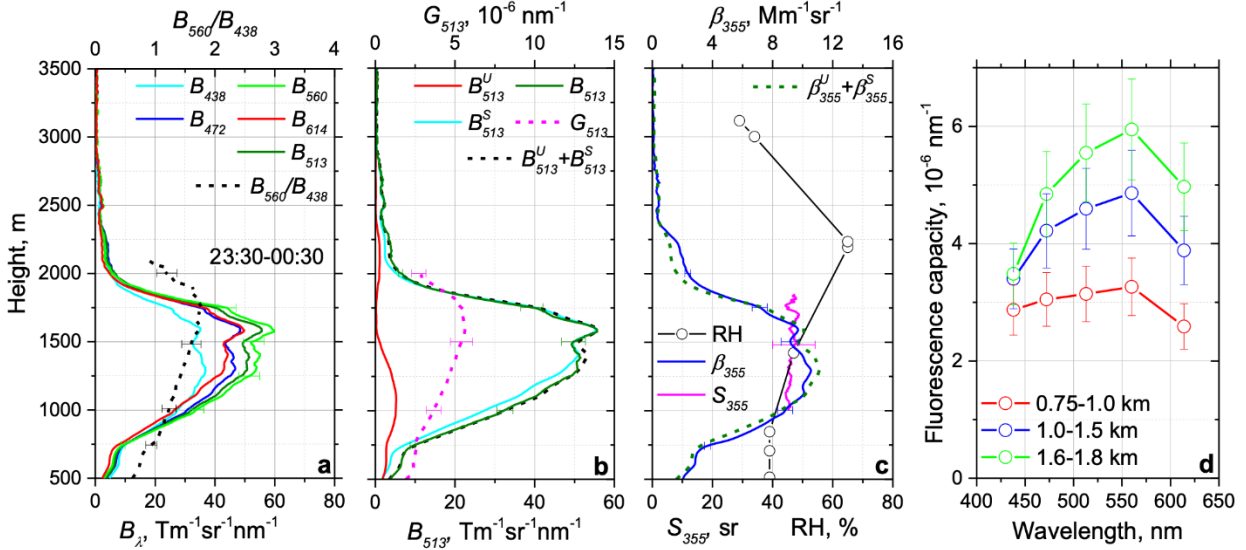
300 Figure 10: Similar to Fig.5, but for 25-26 September 2024 for the period 23:30-00:30 UTC. RH profile was obtained from the Global Data Assimilation System (GDAS).
