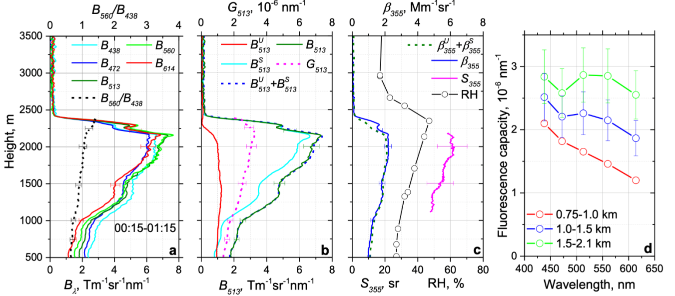
Figure 13: Similar to Fig.5, but for 2 October 2024 for the period 00:15-01:15 UTC. RH profile was obtained from the GDAS.
