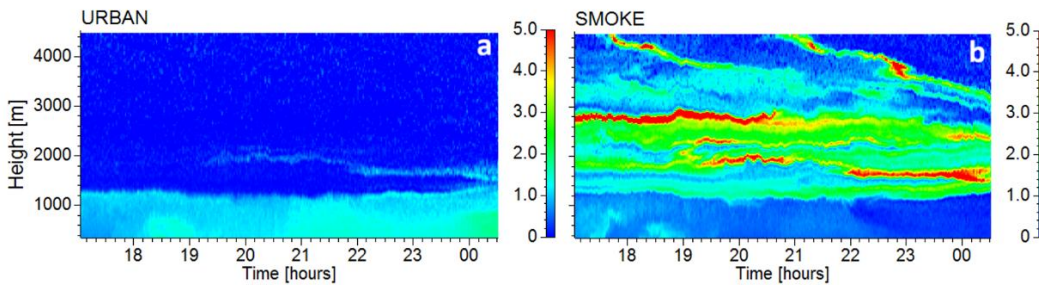
Figure 4: Spatio-temporal distributions of the fluorescence backscattering coefficients (in \text{Tm}^{-1}\text{sr}^{-1}\text{nm}^{-1} ) attributed to (a) urban, B_{513}^U , and (b) smoke, B_{513}^S , particles on 26-27 September 2023.
