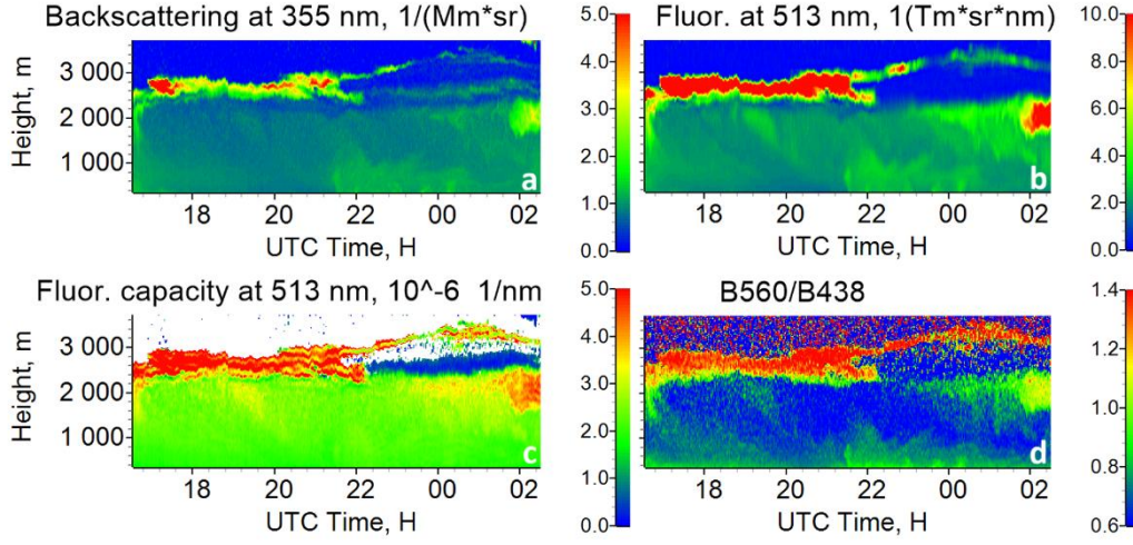
355 Figure 14: Similar to Fig.3, but for the night of 3-4 October, 2024.
