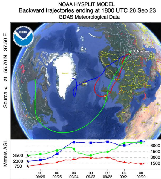
Figure 2: The HYSPLIT six-day backward trajectories for the air mass over Moscow at altitudes 750 m, 2000 m, and 3500 m on 26 September 2023 at 18:00 UTC.
