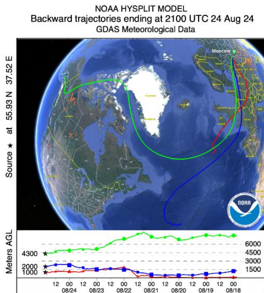
Figure 18: The HYSPLIT seven-day backward trajectories for the air mass over Moscow at altitudes 1000 m, 2000 m, and 4300 m on 24 August 2024 at 21:00 UTC.
