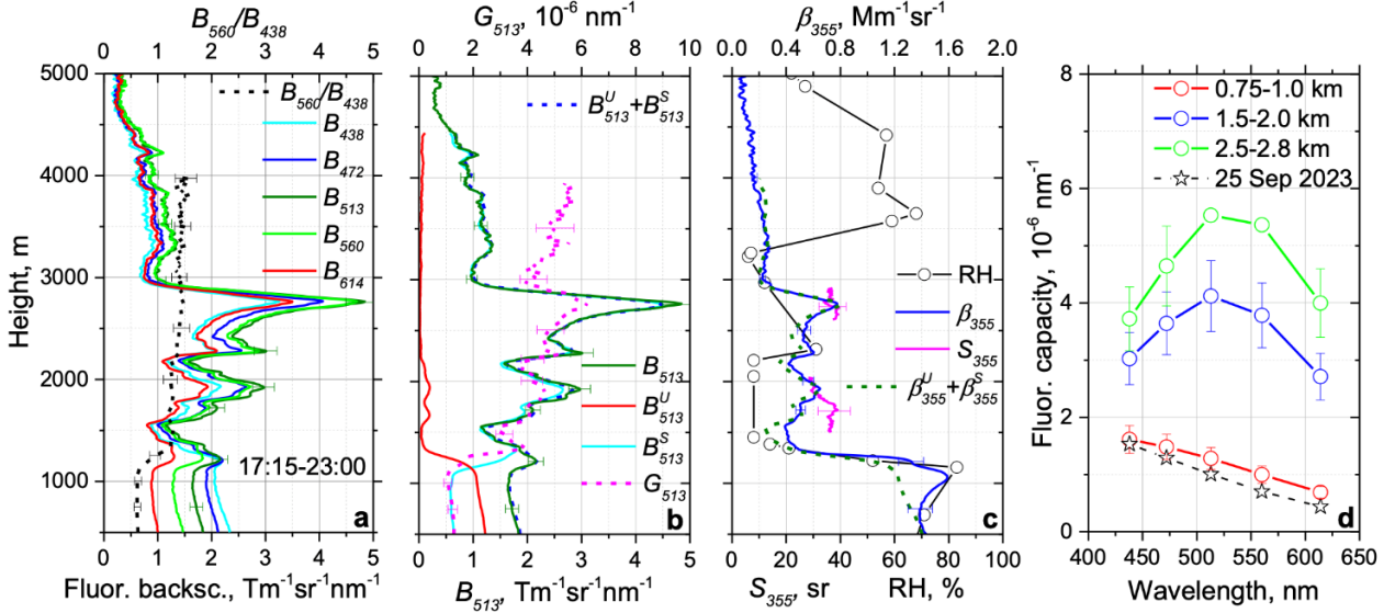
Figure 5. Vertical profiles of particle parameters measured from 17:15 to 23:00 UTC on 26 September 2023. (a) The fluorescence backscattering coefficients, B_\lambda , and the spectral ratio B_{560}/B_{438} . (b) The fluorescence backscattering coefficients attributed to urban, B_{513}^U , and smoke, B_{513}^S , particles, the total measured B_{513} , the reconstructed sum B_{513}^U + B_{513}^S , and the fluorescence capacity, G_{513} . (c) The aerosol backscattering coefficient \beta_{355} , the lidar ratio, S_{355} , and the reconstructed sum of backscattering coefficients, \beta_{355}^U + \beta_{355}^S , attributed to urban and smoke particles. Open symbols show the radiosonde-measured relative humidity, RH. (d) Spectral dependence of fluorescence capacity for different height ranges. The spectrum from 25 September 2023 (0.75–1.0 km), when smoke was absent in the PBL, is shown with stars for reference.
