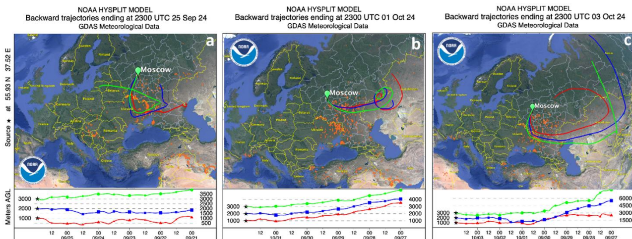
Figure 7: The HYSPLIT five-day backward trajectories for the air mass over Moscow at altitudes 1000 m, 2000 m, and 3000 m at 23:00 UTC on (a) 25 September, (b) 1 October and (c) 3 October 2024.
