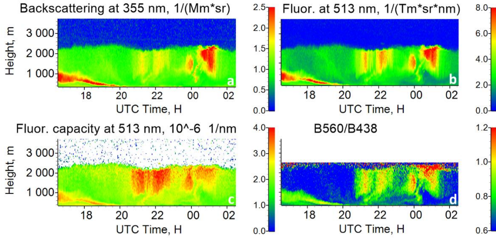
320 Figure 11: Similar to Fig.3, but for the night of 1-2 October 2024.
