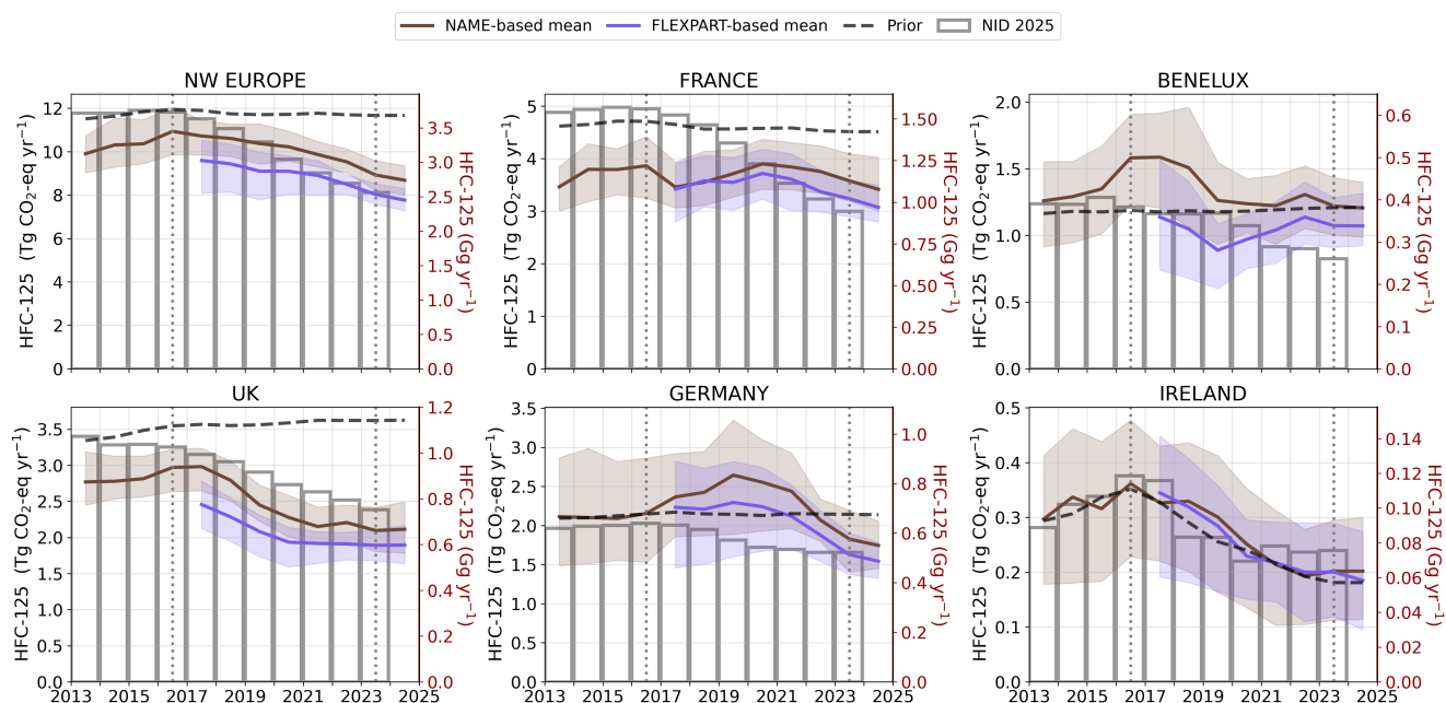
Figure 3. Annual HFC-125 emissions for north-western Europe and its subregions (France, Benelux=Belgium-Netherlands-Luxembourg, UK, Germany, Ireland) from 2013 to 2024. Left y-axes show emissions in Tg CO 2 -eq yr -1 , while right y-axes show emissions in Gg yr -1 . Atmospheric inversion estimates are shown as the NAME-based mean (brown) and FLEXPART-based mean (purple), each representing the average of the InTEM, ELRIS, and RHIME inversion systems, with uncertainty ranges defined by the minimum and maximum of the 15.9 % and 84.1 % percentile, respectively, across the three models. Both means have been smoothed using a three-year moving average. The black dashed line indicates the prior emissions, and national inventory emissions submitted to the UNFCCC (2025 submission; NID 2025) are shown as grey outlined bars. The vertical dotted lines in 2016 and 2023 serve as visual guides for the discussion.
