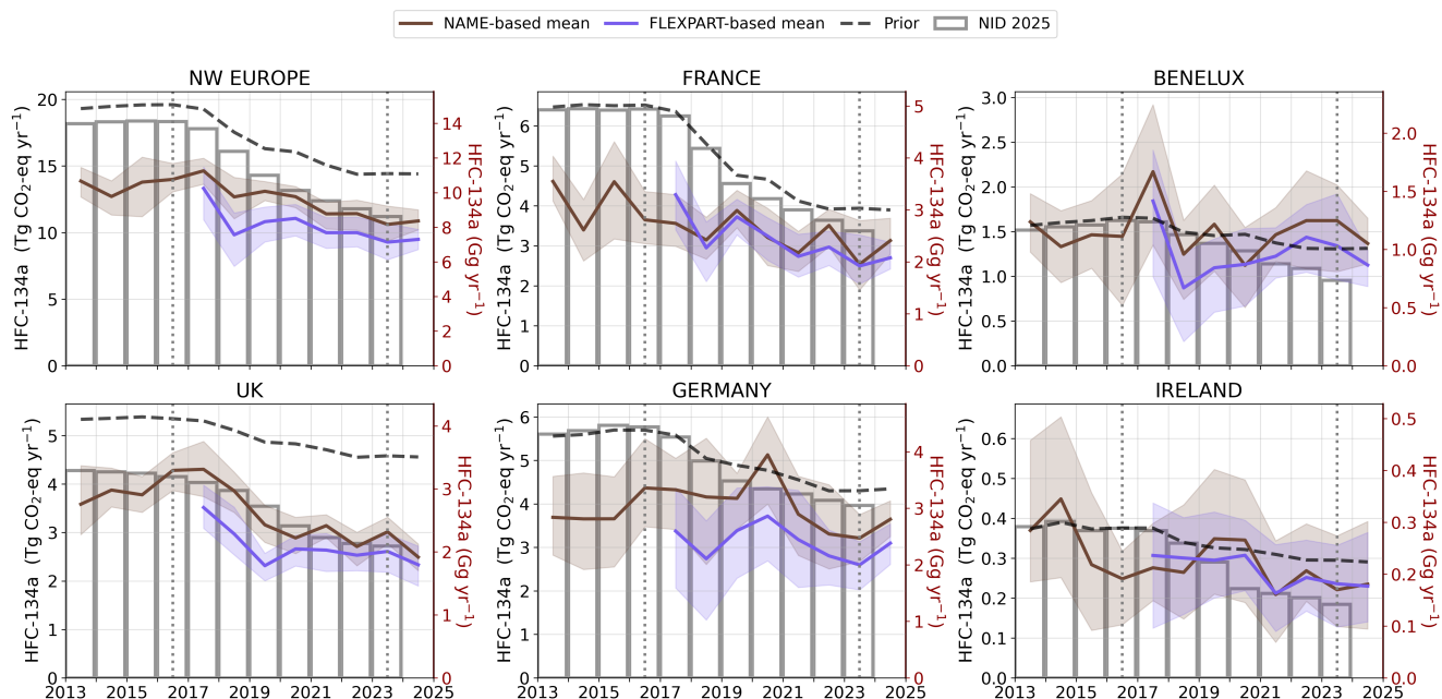
Figure A1. Annual HFC-134a emissions for north-western Europe and its subregions (France, Benelux=Belgium-Netherlands-Luxembourg, UK, Germany, Ireland) from 2013 to 2024. Atmospheric inversion estimates are shown as the NAME-based mean (brown) and FLEXPART-based mean (purple), each representing the average of the InTEM, ELRIS, and RHIME inversion systems from Figure A2, with uncertainty ranges defined by the minimum and maximum of the 15.9% and 84.1% percentile, respectively, across the three models. Compared to Figure 1, no smoothing has been applied to the means. The black dashed line indicates the prior emissions, and national inventory emissions submitted to the UNFCCC (2025 submission; NID 2025) are shown as grey outlined bars. The vertical dotted lines in 2016 and 2023 serve as visual guides for the discussion.
