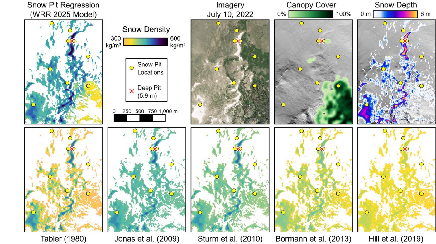
Figure 9. Snow density maps in the region surrounding the Burrow Flat nivation hollow study site (location also shown in Figs. 1, 4, and 5). All of the maps are based on empirical relationships with the lidar-derived snow depth at 3 m resolution in addition to
