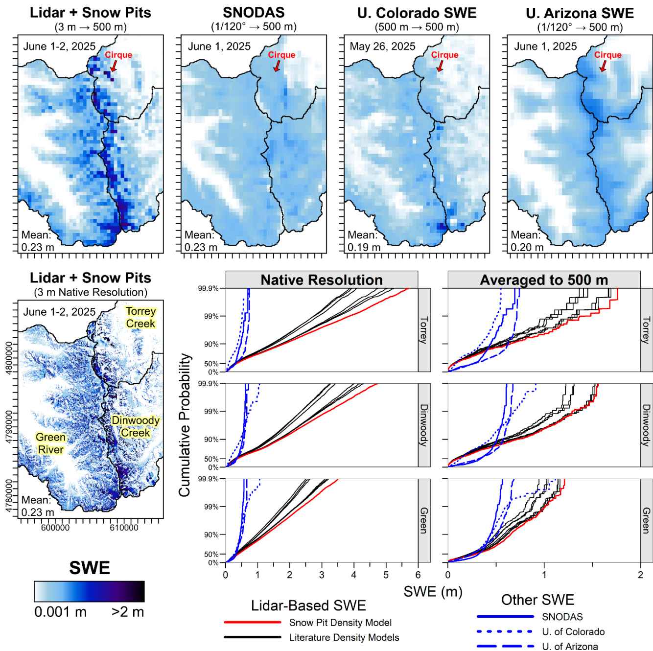
830 Figure 11. Comparison of gridded SWE datasets in the northern WRR study area. Inset plots show the cumulative distribution 831 function of spatial SWE variability within each map (note logarithmically transformed scale on vertical axis). All datasets are 832 averaged to the same 500 m resolution for consistency (upper panels), though the lidar-based dataset is also shown at the native 3 833 m resolution for comparison. Regardless of the density model assumptions, the lidar-based SWE map exhibits more spatial 834 heterogeneity than the other datasets, which drastically underestimate the magnitude and spatial extent of deep snow zones. 835 Nevertheless, density model assumptions can also substantially alter the cumulative SWE distribution.
