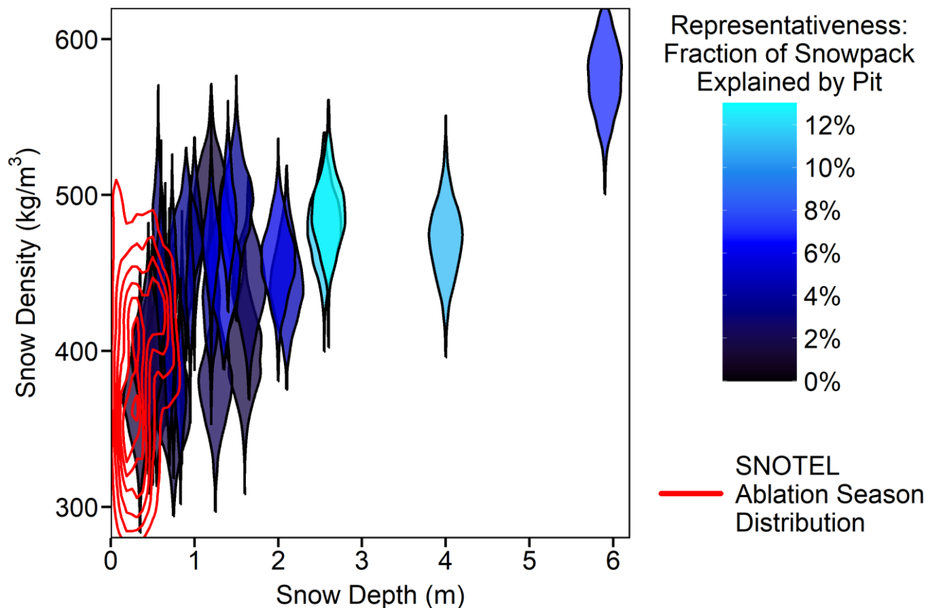
1070 Figure 13: Representativeness of snow pit locations compared to the distribution of SNOTEL data from Wyoming during the 2025 1075 ablation season (beginning from peak SWE at each of 88 SNOTEL locations). Each of the blue violin distributions represents the uncertainty of the Bayesian regression model with respect to a particular snow pit. Lighter blue colors indicate that a particular snow pit is more representative of the WRR lidar-surveyed snowpack as defined in Sect. 2.2.1. The red lines indicate contours of the probability density function (PDF) for the distribution of daily SNOTEL observations of snow depth and density (N = 3676). Note that the SNOTEL observations are exclusively clustered in the least-representative region (shallow snow depth), whereas the most-representative snow pits are between 2 and 4 m deep.
