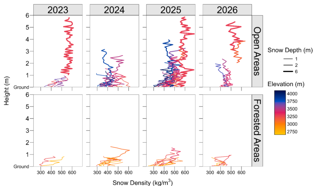
Figure 2. Vertical snow density profiles from 78 snow pits across four years. The sampling resolution is 10 cm vertically. Note the non-representativeness of forested areas with respect to both snow depth and density. Similar patterns of heterogeneity are apparent across years, and the scale of this variability depends on the unique history of accumulation and densification processes occurring each year.
