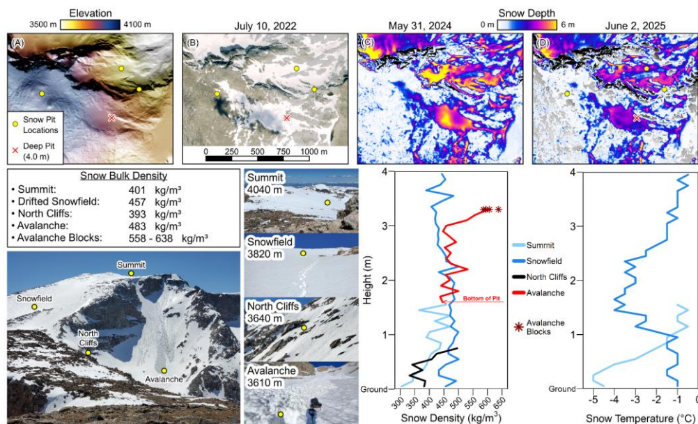
605 Figure 6. Snow depth maps, density / temperature profiles, and photos of four snow pits in the Downs Mountain environs.
