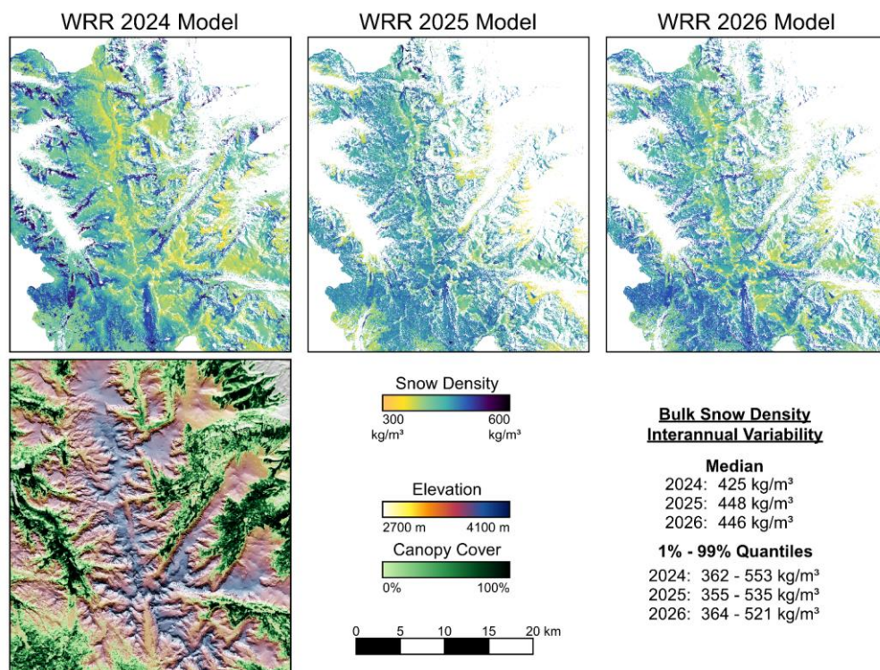
795 Figure 10. Comparison of snow density maps in the northern WRR estimated using airborne lidar depth maps and annual Bayesian regression models (Table 1). Snow density maps and statistics are masked to only include areas with lidar-based snow depth > 0.2 m. Although the broad patterns of density heterogeneity are consistent, snowpack settings such as high elevations, deep drifts, and forested areas exhibit differing levels of sensitivity each year.
