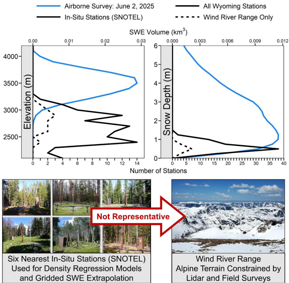
Figure 12: Comparison of elevation and snow depth distribution of the northern WRR snowpack at the time of our June 2, 2025, airborne lidar survey. Note the dual axes on the plots: the top axis shows the volume of SWE (from lidar and snow pit density regression), and the bottom axis shows the number of SNOTEL stations within respective elevation or snow depth bands. The reported SNOTEL snow depth is the maximum depth observed at each site in water year 2025 (most SNOTEL sites were snow-free at the time of our lidar survey). The SNOTEL photos are USA Natural Resource Conservation Service (NRCS) stock photos (Public Domain). The alpine photo (by the authors) is from May 31, 2025, (nearly contemporaneous with the lidar survey), looking west into the Green River headwaters from Downs Mountain (Fig. 1).
