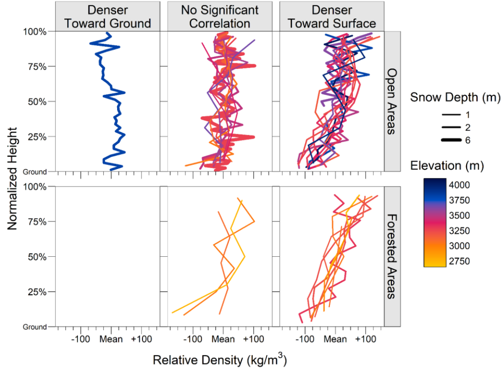
485 Figure 3. Vertical density trends relative to the bulk density of each snow pit (only considering the 36 snow pits from 2025). Most snow pits have trends toward denser snow near the surface or no trend, and only one location has a trend toward denser snow near the ground. The threshold for trend significance is p < 0.05 using Pearson's product-moment correlation test.
