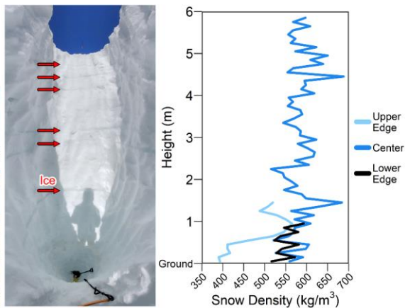
Figure 4. Snow depth profiles (longitudinal) and snow density profiles (vertical) from the Burrow Flat nivation hollow. Note that the longitudinal surface profile has the same horizontal and vertical scales. The human figure near the center snow pit (in the longitudinal profile) has an approximate height of 1.8 m (6 feet), and human figures are also visible in the overview photograph near the center snow pit. The deviation in the 2025 snow depth profile is the result of our partially refilled center snow pit excavation. Major ice layers are indicated in the closeup photograph with red arrows, but there are also many thin ice layers near the surface that are not indicated.
