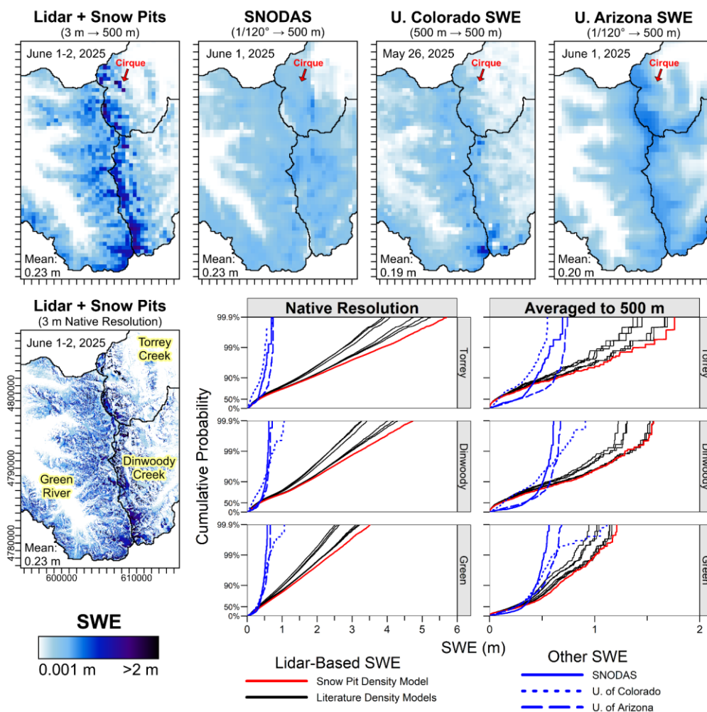
Figure 4011. Comparison of gridded SWE datasets in the northern WRR study area. Inset plots show the cumulative distribution function of spatial SWE variability within each map (note logarithmically transformed scale on vertical axis). All datasets are averaged to the same 500 m resolution for consistency (upper panels), though the lidar-based dataset is also shown at the native 3 m resolution for comparison. Regardless of the density model assumptions, the lidar-based SWE map exhibits more spatial heterogeneity than the other datasets, which drastically underestimate the magnitude and spatial extent of deep snow zones. Nevertheless, density model assumptions can also substantially alter the cumulative SWE distribution.
