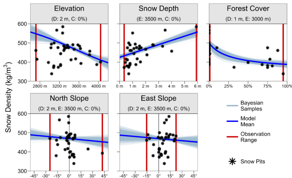
Figure 7. Evaluation of the 2026 WRR statistical snow density model with respect to individual variables. (Eq. 1, Table 1). In each panel, all other variables are held constant, and the snow density response is predicted with respect to a single variable (e.g., for elevation, the snow depth is held constant at 2 m with 0% forest cover). D = snow depth, C = forest cover, E = elevation. All topographic slopes are flat except as specified. Snow pit measurements are shown to illustrate the range of variability, but since each snow pit corresponds to a unique combination of all five predictors, the snow pit points are not expected to fit the univariate sensitivity tests shown here.
