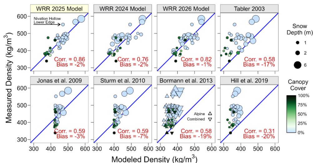
Figure 8. Comparison of measured snow densities with predicted density from various empirical models (Table 1). The WRR 2025 model is directly fit solely to this dataset, and the WRR 2024 model is fit to various WRR observations from previous years 2023-2024 , and the WRR 2026 model is fit to observations from 2023-2026. The other models are based on an array of global observations presented in the literature, and are not necessarily intended for general extrapolation. Correlation and bias for the Bormann et al. (2013) models are reported as averages between the alpine model and the model based on all combined global sites. Note that all of the prior literature models substantially underestimate the highest densities, and most models neglect the density contrast between snow in forested and open areas.
