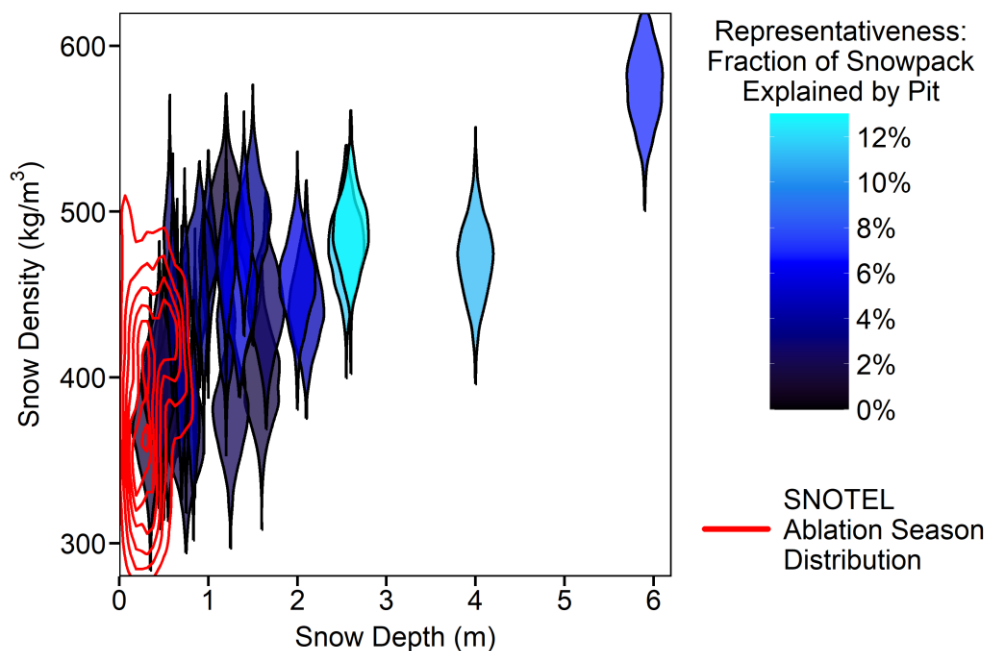
Figure 4213: Representativeness of snow pit locations compared to the distribution of SNOTEL data from Wyoming during the 2025 ablation season (beginning from peak SWE at each of 88 SNOTEL locations). Each of the blue violin distributions represents the uncertainty of the Bayesian regression model with respect to a particular snow pit. Lighter blue colors indicate that a particular snow pit is more representative of the WRR lidar-surveyed snowpack as defined in Sect. 2.2.1. The red lines indicate contours of the probability density function (PDF) for the distribution of daily SNOTEL observations of snow depth and density ( N = 3676 ). Note that the SNOTEL observations are exclusively clustered in the least-representative region (shallow snow depth), whereas the most-representative snow pits are between 2 and 4 m deep.
