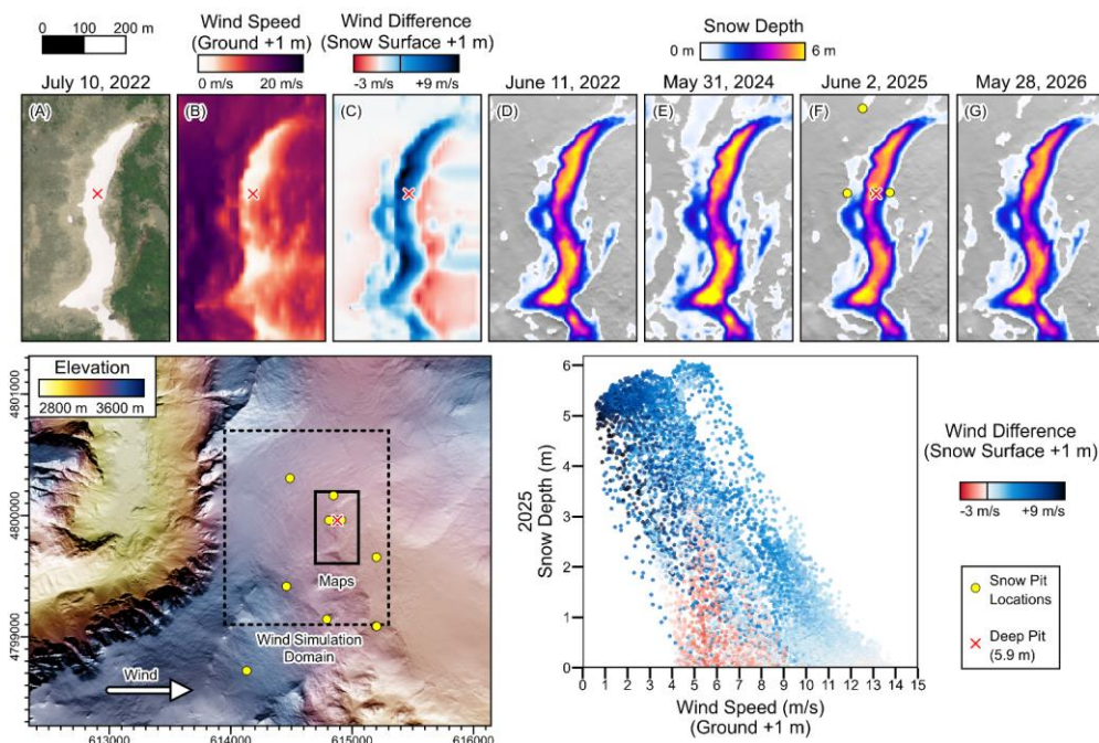
Figure 5. Wind speed simulations and annual snow depth maps associated with the Burrow Flat nivivation hollow.
