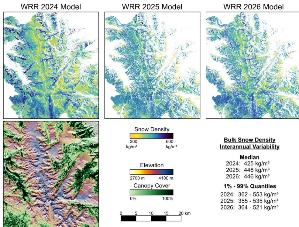
835 Figure 10. Comparison of snow density maps in the northern WRR estimated using airborne lidar depth maps and annual Bayesian regression models (Table 1). Snow density maps and statistics are masked to only include areas with lidar-based snow depth > 0.2 m. Although the broad patterns of density heterogeneity are consistent, snowpack settings such as high elevations, deep drifts, and forested areas exhibit differing levels of sensitivity each year.
