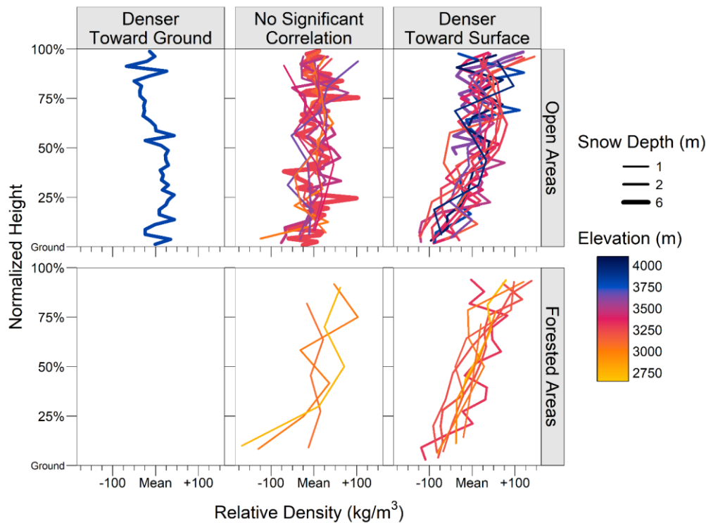
Figure 3. Vertical density trends relative to the mean bulk density of each snow pit. (only considering the 36 snow pits from 2025). Most snow pits have trends toward denser snow near the surface or no trend, and only one location has a trend toward denser snow near the ground. The threshold for trend significance is p < 0.05 using Pearson's product-moment correlation test.
