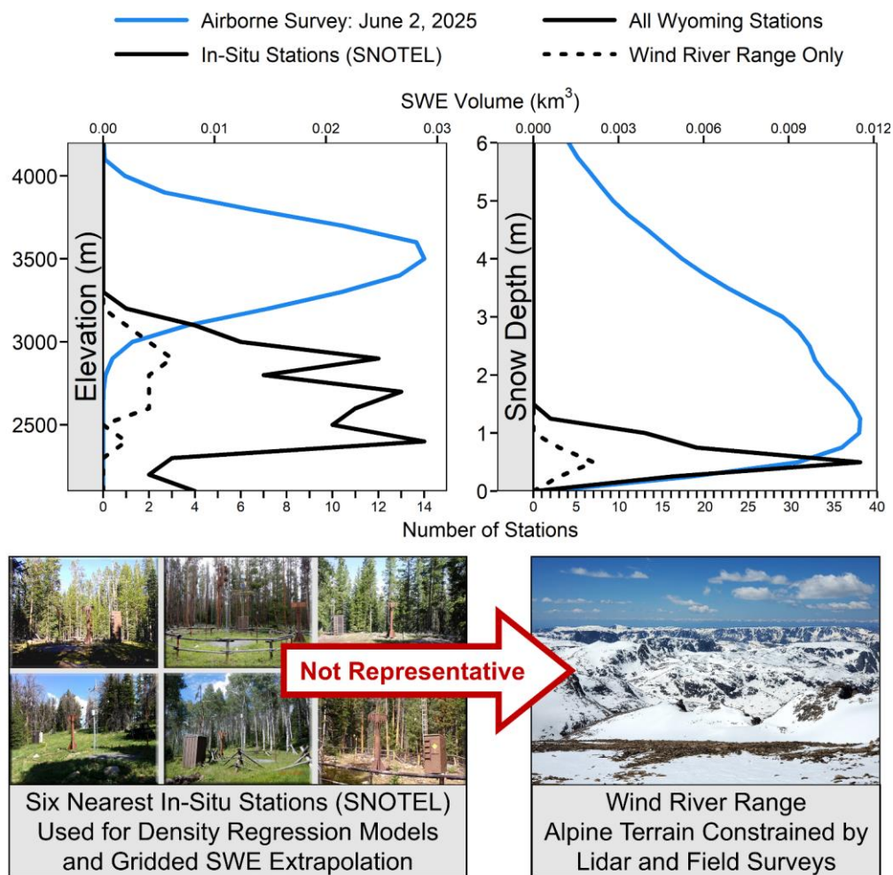
Figure 4-12: Comparison of elevation and snow depth distribution of the northern WRR snowpack at the time of our June 2, 2025, airborne lidar survey. Note the dual axes on the plots: the top axis shows the volume of SWE (from lidar and snow pit density regression), and the bottom axis shows the number of SNOTEL stations within respective elevation or snow depth bands. The reported SNOTEL snow depth is the maximum depth observed at each site in water year 2025 (most SNOTEL sites were snow-free at the time of our lidar survey). The SNOTEL photos are USA Natural Resource Conservation Service (NRCS) stock photos (public domainPublic Domain) . The alpine photo (by the authors) is from May 31, 2025, looking west into the Green River headwaters from Downs Mountain. (Fig. 1) .
