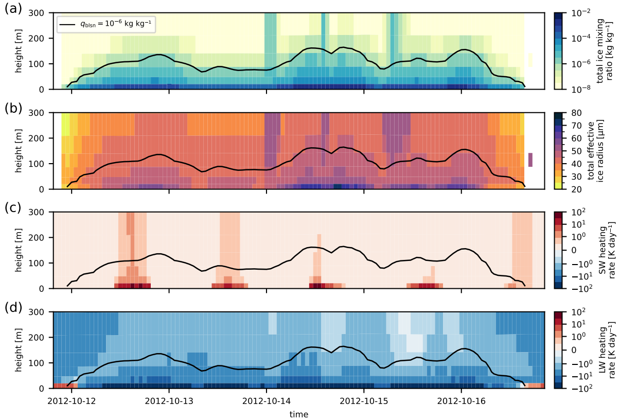
Figure 6. Timeseries of hourly input and output profiles of ecRad-1.4.1 for the integrated grid (IG) experiment during a blowing snow event at S10 from 2012-10-12 until 2012-10-17: a ) total ice mixing ratio (including blowing snow) q_{\text{total, ice}} [ \text{kg kg}^{-1} ], b ) total effective radius of ice particles r_{\text{e}}^{\text{total, ice}} [ \mu\text{m} ], c , d ) net shortwave and longwave heating rates [ \text{K day}^{-1} ]. The black line represents the height at which the blowing snow mixing ratio q_{\text{blsn}} = 10^{-6} \text{ kg kg}^{-1} , indicating the approximate height of the top of the blowing snow layer.
