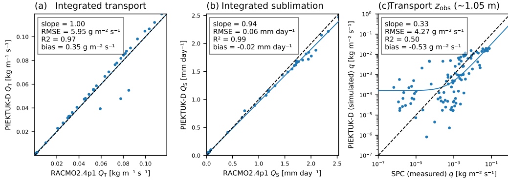
Figure C1. Scatter plots of the measured and simulated horizontal blowing snow transport fluxes and sublimation rates at site S10 from 2012-09-07 until 2012-10-06 for RACMO2.4p1 and the offline PIEKTUK-D model: a), b) vertically integrated horizontal blowing snow transport flux Q_T [ \text{kg m}^{-1} \text{s}^{-1} ] and vertically integrated sublimation rate Q_S [ \text{mm day}^{-1} ] of RACMO2.4p1 and PIEKTUK-D (including blowing snow grid and mean radius bugs), and c) measured and simulated horizontal blowing snow transport fluxes q [ \text{kg m}^{-2} \text{s}^{-1} ] of the SPC and PIEKTUK-D at the observation height above the surface z_{\text{obs}} (without bugs). Dashed lines represent the 1:1 line, solid lines represent the best-fit line, and the colours represent the normalised point density from low (0.0, dark blue) to high (1.0, red).
