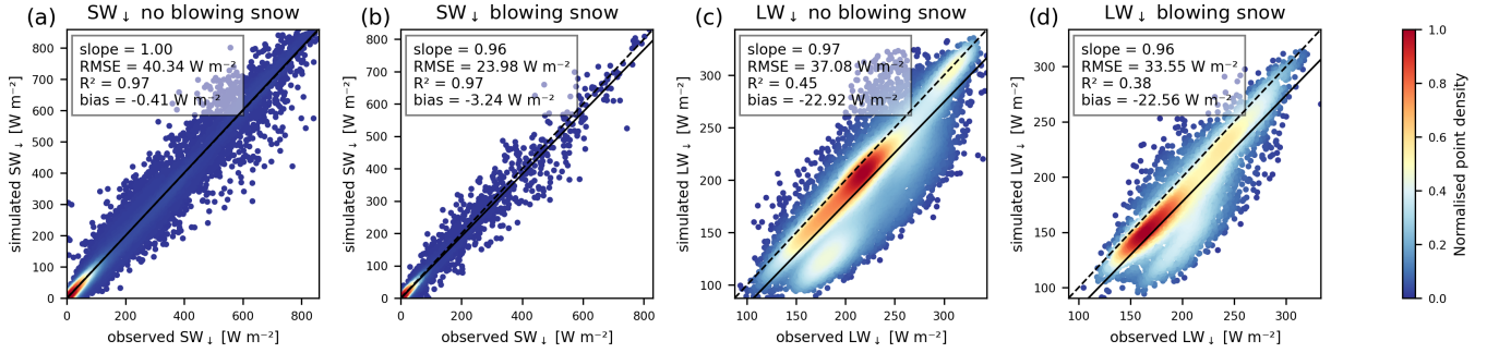
Figure 4. Density scatter plots of the simulated and observed surface radiation fluxes for the baseline experiment at site S10 without ( Q_T < 10^{-3} \text{ kg m}^{-1} \text{ s}^{-1} ) and with blowing snow ( Q_T > 10^{-3} \text{ kg m}^{-1} \text{ s}^{-1} ) between 2010 and 2016: a, b ) downwelling surface shortwave radiation flux \text{SW}_\downarrow without and with blowing snow [ \text{W m}^{-2} ], c, d ) downwelling surface longwave radiation flux \text{LW}_\downarrow without and with blowing snow [ \text{W m}^{-2} ]. Dashed lines represent the 1:1 line, solid lines represent the linear regression line, and the colours represent the normalised point density from low (0.0, dark blue) to high (1.0, red).
