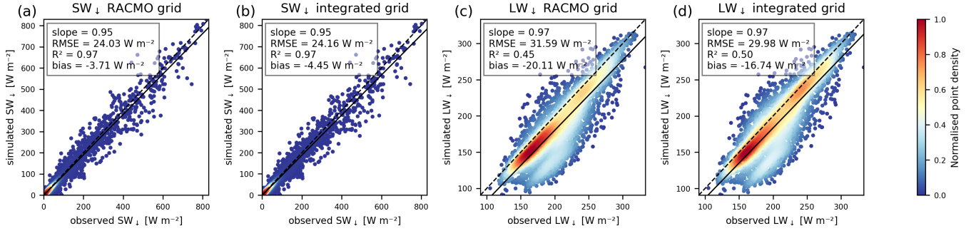
Figure 7. Density scatter plots of the simulated and observed surface radiation fluxes at site S10 during blowing snow events ( Q_T > 10^{-3} \text{ kg m}^{-1} \text{ s}^{-1} ) between 2010 and 2016 for the RACMO grid (RG) and integrated grid (IG) experiments: a, b ) downwelling surface shortwave radiation flux SW_{\downarrow} of the RG and IG experiments [ \text{W m}^{-2} ], c, d ) downwelling surface longwave radiation flux LW_{\downarrow} from the RG and IG experiments [ \text{W m}^{-2} ]. Dashed lines represent the 1:1 line, solid lines represent the linear regression line, and the colours represent the normalised point density from low (0.0, dark blue) to high (1.0, red).
