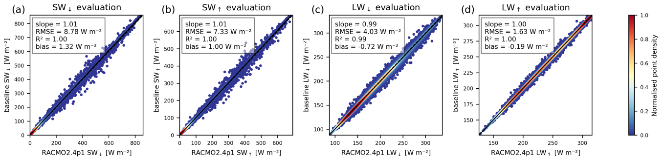
Figure D1. Density scatter plots of the simulated surface radiation fluxes at site S10 for RACMO2.4p1 and the offline baseline model: a) downwelling surface shortwave radiation flux SW_{\downarrow} [ W m^{-2} ], b) upwelling surface shortwave radiation flux SW_{\uparrow} [ W m^{-2} ], c) downwelling surface longwave radiation flux LW_{\downarrow} [ W m^{-2} ], and d) upwelling surface longwave radiation flux LW_{\uparrow} [ W m^{-2} ]. Dashed lines represent the 1:1 line, solid lines represent the best-fit line, and the colours represent the normalised point density from low (0.0, dark blue) to high (1.0, red).
