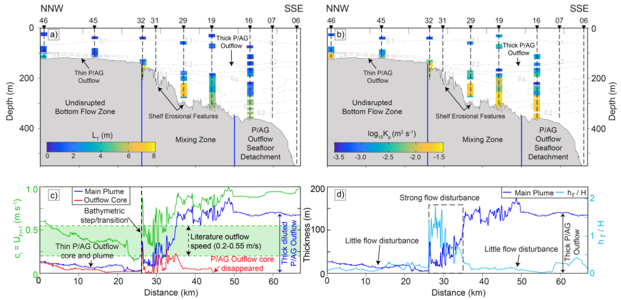
Figure 3: An NNW-SSE CTD transect (along the hydrographically inferred P/AG plume corridor; the white line in Fig. 1a) showing CTD- and bathymetric-derived proxies. The parameters include Thorpe scale (a) and the diapycnal diffusivity (based on Thorpe scales) proxy (b) plotted for the accepted overturns only, as well as the along-transect thickness of the P/AG outflow core and main plume and the CTD-derived critical velocity, c_i (c), and the roughness-to-plume thickness ratio h_r/H plotted with the plume thickness along the transect (d). a and b are superimposed by P/AGw f contours.
