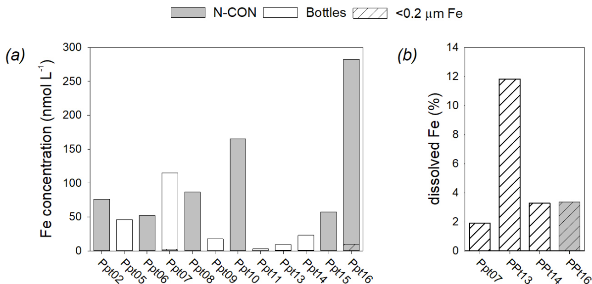
350 Figure 3: Iron concentration and solubility in GN01 precipitation samples. (a) Total dissolvable and dissolved Fe concentrations in precipitation samples collected by N-CON sampler and cut-off bottles, with dissolved Fe contributions to four samples indicated by hatching. (b) Percent of total dissolvable Fe in the dissolved fraction at the time of sample recovery for four samples where a subsample was filtered.
