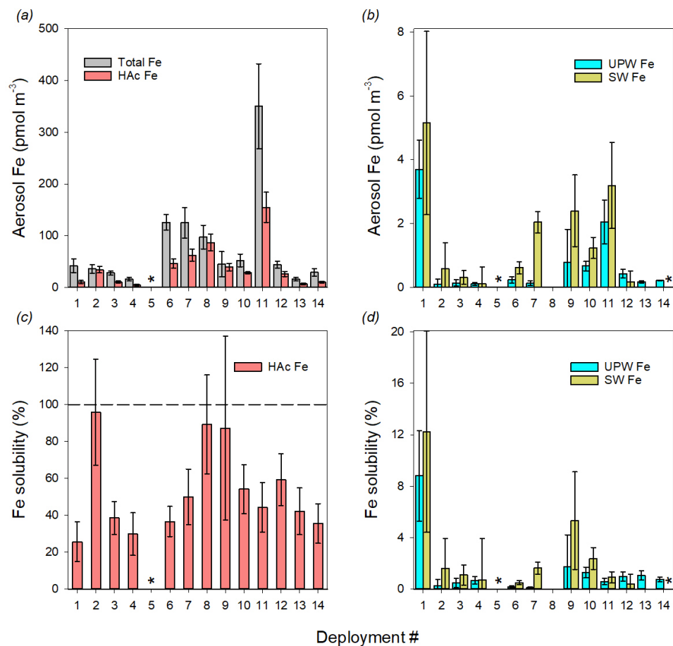
225 Figure 2: Aerosol Fe concentrations and Fe fractional solubility in GN01 aerosols, where fractional solubility is the ratio of soluble to total Fe, expressed as a percentage. (a) concentrations of total Fe and HAc-soluble Fe, (b) concentrations of UPW-soluble and SW-soluble Fe, (c) fractional solubility of Fe in the HAc leach, (d) fractional solubility of Fe in the UPW and SW leaches. Asterisks indicate no data (Aer05, SW leach of Aer14). Values for Aer08 (UPW and SW leaches) and Aer13 (SW leach only) were less than 230 average filter blank. Error bars are propagated error as described in the text and include air volume uncertainty for Aer01. Dashed line in (c) marks 100%.
