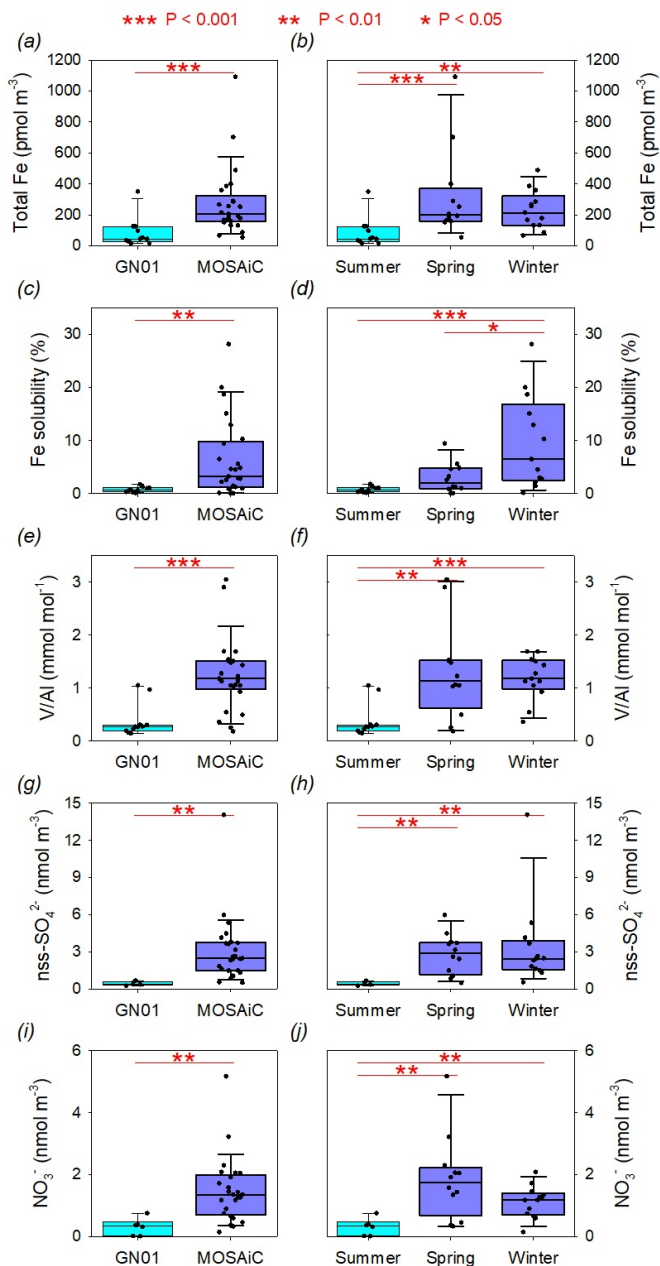
Figure 5: Comparison of aerosol characteristics between GN01 (cyan) and MOSAiC (purple). (a, b) Total aerosol Fe concentration, (c, d) Fe UPW-solubility, (e, f) V/Al molar ratio, (g, h) nss-sulfate concentration, and (i, j) nitrate concentration. Comparisons are made between the two projects (left column) and between seasonal datasets (right column), with MOSAiC data (n = 26) split between winter (deployments 1-13, n = 13) and spring (deployments 14-26, n = 13). GN01 data excludes samples collected south of 70°S (Aer01, Aer14; n = 11, or less where some measurements are below detection). Each box spans 25 th to 75 th percentiles of data and is bisected by the median, with whiskers extending to 10 th and 90 th percentiles. Individual datapoints are superimposed as dots. Red lines indicate statistically significant differences between datasets (Mann-Whitney Rank Sum Test), with level of significance indicated by asterisks.
