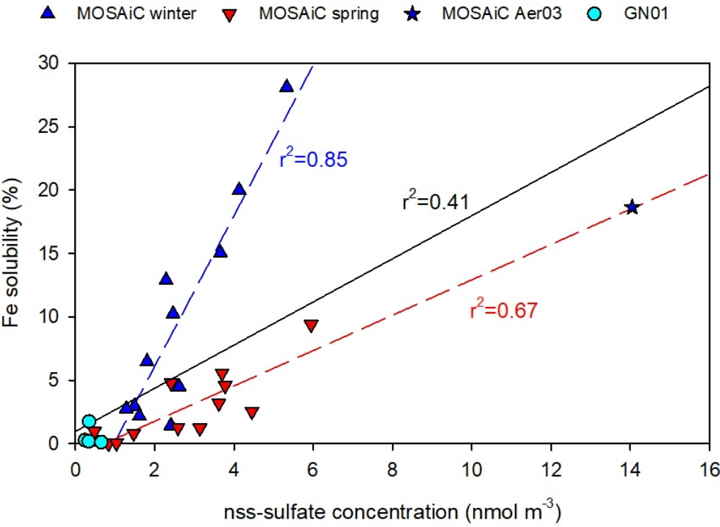
Figure 6: Relationship between aerosol Fe solubility and nss-sulfate concentration. Fe solubility is plotted against nss-sulfate concentration for GN01 (cyan circles), MOSAiC Winter (blue triangles), and MOSAiC Spring (red inverted triangles). Dashed regression lines are included where statistically significant correlations exist for seasonal data (Aer03 excluded from MOSAiC winter data due to unusually high nss-sulfate). Solid black regression line indicates significant correlation for all data.
