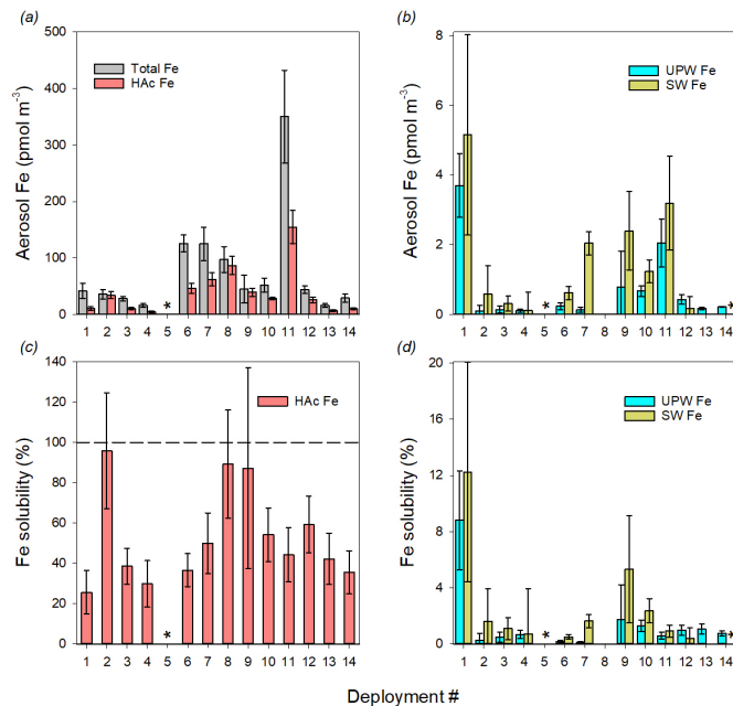
Figure 2: Aerosol Fe concentrations and Fe fractional solubility in GN01 aerosols, where fractional solubility is the ratio of soluble to total Fe, expressed as a percentage. (a) concentrations of total Fe and HAC-soluble Fe, (b) concentrations of UPW-soluble and SW-soluble Fe, (c) fractional solubility of Fe in the HAC leach, (d) fractional solubility of Fe in the UPW and SW leaches. Asterisks indicate no data (Aer05, SW leach of Aer14). Values for Aer08 (UPW and SW leaches) and Aer13 (SW leach only) were less than average filter blank. Error bars are propagated error as described in the text and include air volume uncertainty for Aer01 . Dashed line in (c) marks 100%.
