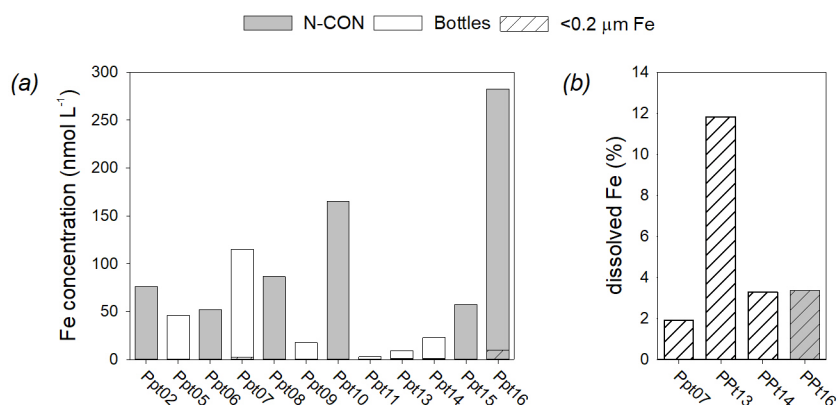
Figure 3: Iron concentration and solubility in GN01 precipitation samples. (a) Total dissolvable and dissolved Fe concentrations in precipitation samples collected by N-CON sampler and cut-off bottles, with dissolved Fe contributions to four samples indicated by hatching. (b) Percent of total dissolvable Fe in the dissolved fraction at the time of sample recovery for four samples where a subsample was filtered.
