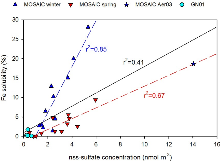
730 Figure 6: Relationship between aerosol Fe solubility and nss-sulfate concentration. Fe solubility is plotted against nss-sulfate concentration for GN01 (cyan circles), MOSAiC Winter (blue triangles), and MOSAiC Spring (red inverted triangles). Dashed regression lines are included where statistically significant correlations exist for seasonal data (Aer03 excluded from MOSAiC winter data due to unusually high nss-sulfate). Solid black regression line indicates significant correlation for all data.
