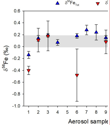
Figure 3: Iron stable isotope (δ 56 Fe) data for GN01 aerosols. Blue triangles are δ 56 Fe for aerosol digests and red inverted triangles are δ 56 Fe for UPW leaches. Error bars represent internal analytical error of δ 56 Fe measurements (2σ). Shaded area represents typical δ 56 Fe values for the upper continental crust (+0.9 ± 1.0 ‰; Gong et al., 2017; Zhang et al., 2025).
