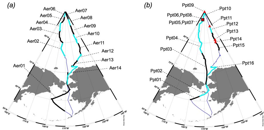
150 Figure 1: Locations of (a) bulk aerosol and (b) precipitation samples collected during GN01. Cruise track is shown by thin blue line with aerosol or N-CON precipitation sample collections overlain in black and light blue on each map. Red triangles in (b) indicate locations of blowing snow samples collected with cutoff bottles, while the black square indicates two N-CON samples (Ppt06, Ppt08) collected close to each other and to cutoff bottle samples Ppt05 and Ppt07. Figure produced using Ocean Data View (Schlitzer, 2025).
