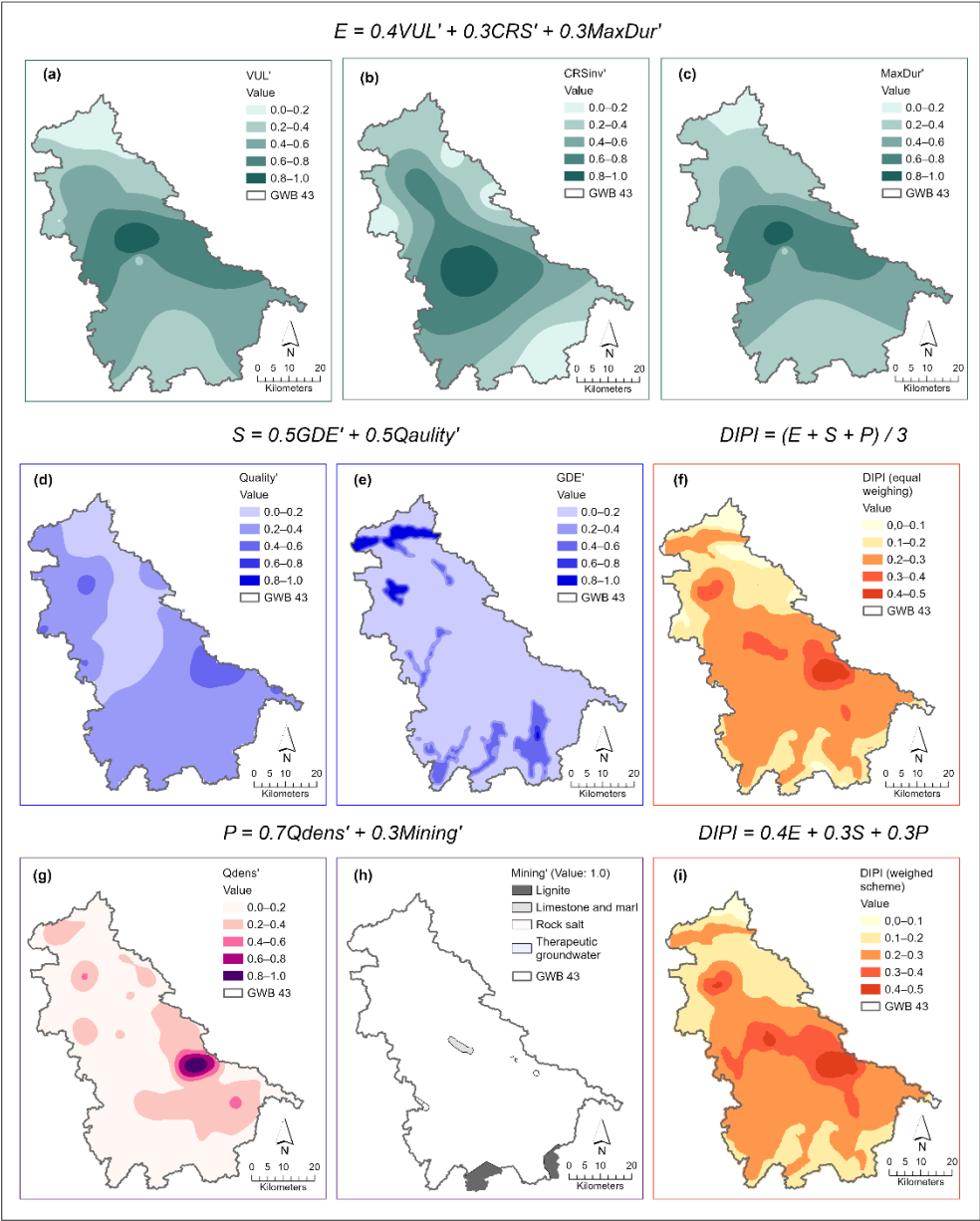
Figure A1: Spatial distribution of normalised DIPI sub-components and comparison of aggregation schemes. Panels (a–c) present the normalised exposure metrics (VUL', CRSinv', MaxDur'), panels (d–e) the sensitivity layers (Quality', GDE'), and panels (g–h) the pressure layers (Qdens', Mining'). Panels (f) and (i) compare the equally weighted and weighted DIPI variants, respectively, illustrating similarities and local differences between the two weighting schemes.
