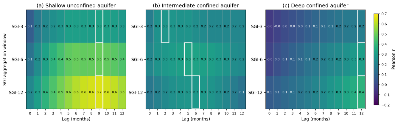
810 Figure B1. Full-period lagged SPI–SGI correlations for the three monitored aquifer systems in GWB 43. Panels show Pearson correlation coefficients between aquifer-group mean SGI and SPI from the meteorological station nearest to the corresponding aquifer-group centroid for (a) the shallow unconfined aquifer, (b) the intermediate confined aquifer, and (c) the deep confined aquifer. Correlations were calculated separately for the 3-, 6-, and 12-month aggregation scales over lags of 0–12 months. White outlines mark the lag associated with the maximum correlation in each row. Positive lags indicate 815 that SGI follows SPI. Maxima occurring at 12 months represent the upper boundary of the tested range and do not exclude longer response delays.
