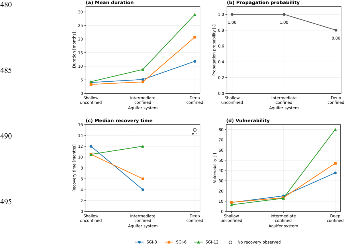
Figure 5. Groundwater drought metrics across the three monitored aquifer systems and aggregation scales. Comparison of (a) mean drought duration, (b) propagation probability from SGI-3 to SGI-12, (c) median recovery time, and (d) vulnerability (VUL) for the shallow unconfined, intermediate confined, and deep confined aquifer systems. Mean duration, recovery time, and vulnerability are shown for SGI-3, SGI-6, and SGI-12. Propagation probability is reported as a single SGI-3-to-SGI-12 value for each aquifer system. Open symbols and “n.r.” indicate that no recovery was observed within the available
