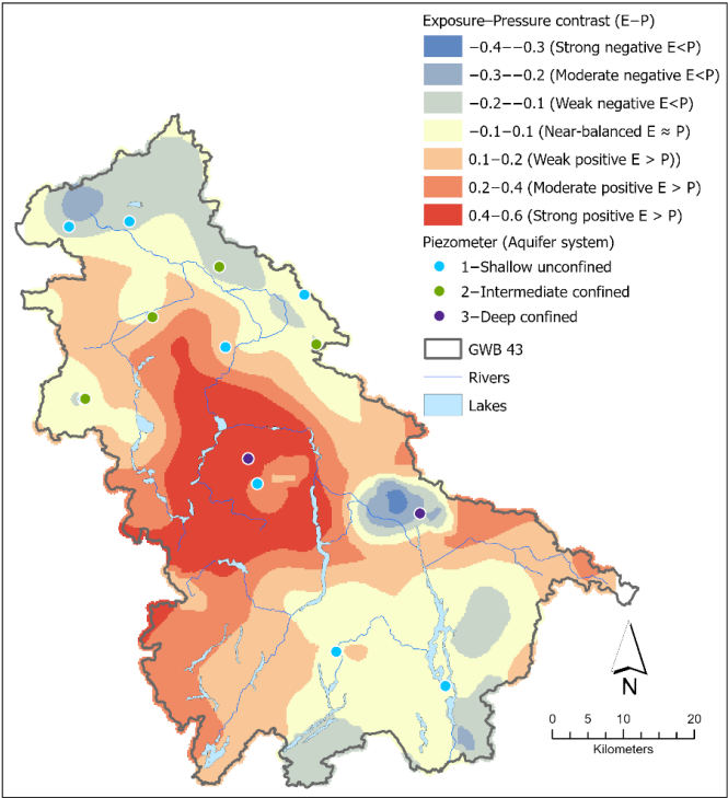
Figure 8. Spatial contrast between normalised Exposure (E) and Pressure (P) in GWB 43. Positive values are consistent with areas where E exceeds P, negative values are consistent with areas where P exceeds E, and values between –0.1 and 0.1 represent a balanced contrast. The E–P classes provide a descriptive comparison of the relative mapped component magnitudes and should not be interpreted as causal attribution.
