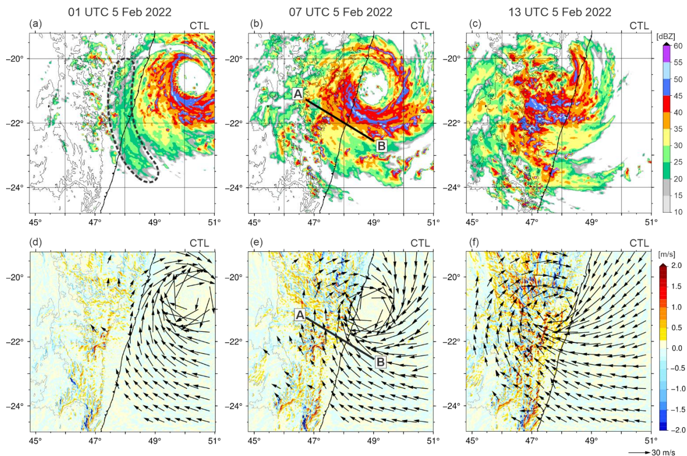
515 Figure 12. Horizontal distributions of CTL-simulated (a–c) reflectivity at 3 km above sea level and (d–f) vertical velocity at 20 m above sea level at 01, 07, and 13 UTC on 5 February 2022. The southeastern coastline of Madagascar is indicated by a thick solid line, and topographic contours at 500 m intervals are shown by thin solid lines in all panels. Horizontal wind vectors exceeding 10 \text{m s}^{-1} are shown. The location of the vertical cross section along A–B used in Fig. 14 is marked by a black solid line in panels (b) and (e). The spiral rainband along the coastline of Madagascar is delineated by black dashed contour in panel (a).
