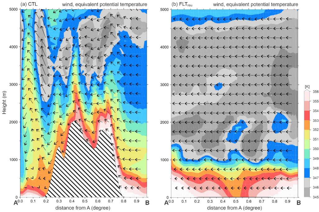
435 Figure 11. Vertical cross-sections of wind ( u - w vectors) and equivalent potential temperature ( \theta_e , shaded) along the A–B line, simulated by (a) CTL and (b) FLT_{reu} at 00 UTC on 3 February. The location of the A–B line is shown by the green solid line in Figs. 9e and 10e for the CTL and FLT_{reu} simulations, respectively. The hatched area in (a) represents the topography.
