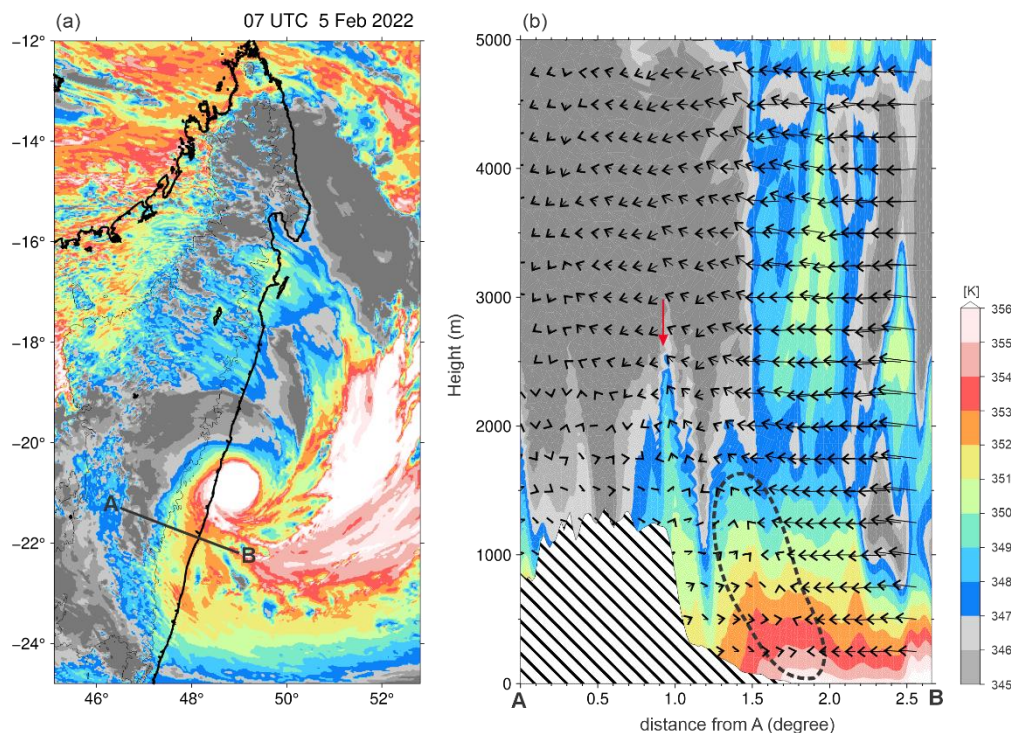
560 Figure 14. Horizontal and vertical distributions of CTL-simulated equivalent potential temperature ( \theta_e ) over the Madagascar region at 07 UTC on 5 February 2022. Panel (a) shows the horizontal map with the A-B line indicating the location of the vertical cross section, which is presented in panel (b). A downward red arrow indicates the localized warm and moist layer at low altitude above the mountain ridge.
