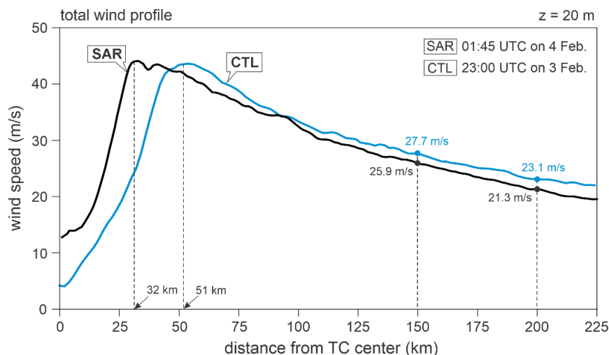
265 Figure 5. Near-surface wind profiles at 20 m height for TC Batsirai. Observations from SAR at 01:45 UTC on 4 February 2022 are shown as a black solid line, while the CTL simulation at 23 UTC on 3 February 2022 is shown in blue.
