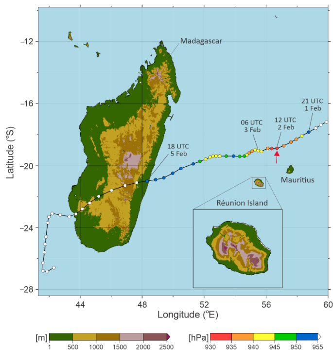
95 Figure 1. Topography of the SWIO region and the observed trajectory of TC Batsirai (2022) from International Best Track Archive for Climate Stewardship (IBTrACS) best-track data. Three-hourly minimum sea level pressure (MSLP) values are indicated by colored circles along the black solid line. The location and timing of the cyclone's minimum MSLP (12 UTC on 2 February 2022) are highlighted with a red arrow.
