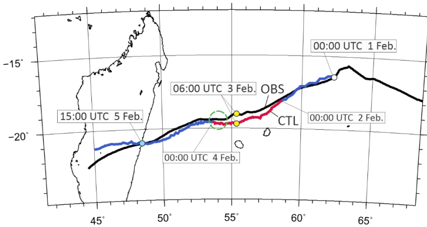
220 Figure 3. Model domain and observed and simulated tracks of TC Batsirai (2022). The observed IBTrACS track is shown by the black line, while the CTL-simulated track is shown in blue. The highlighted segment (00 UTC 2 February to 00 UTC 4 February) indicates the period of noticeable track discrepancy between CTL and IBTrACS. The white dot marks the initial CTL simulation time (00 UTC 1 February), yellow dots indicate the closest approach of Batsirai to Réunion Island, and the blue dot shows the landfall of observed TC on the eastern coast of Madagascar. The approximate position of TC centre captured by the SAR measurement at 225 01:45 UTC is marked by the green dashed circle.
