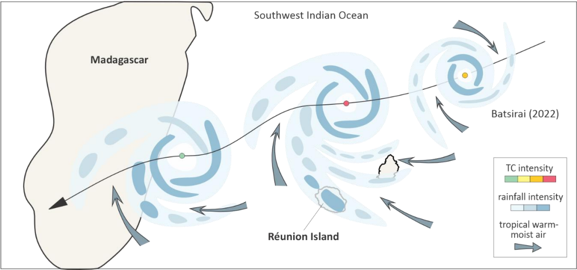
585 Figure 15. Schematic illustration of tropical cyclone Batsirai (2022). Rainfall intensity is indicated by a blue color scale, with darker shades representing stronger precipitation. Dark blue arrows show the warm, moist low-level flows associated with the TC, while the black arrow represents the TC trajectory.
