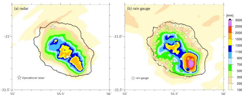
Figure 2. Three-day accumulated precipitation over Réunion Island from 00 UTC on 2 February to 00 UTC on 5 February 2022.
