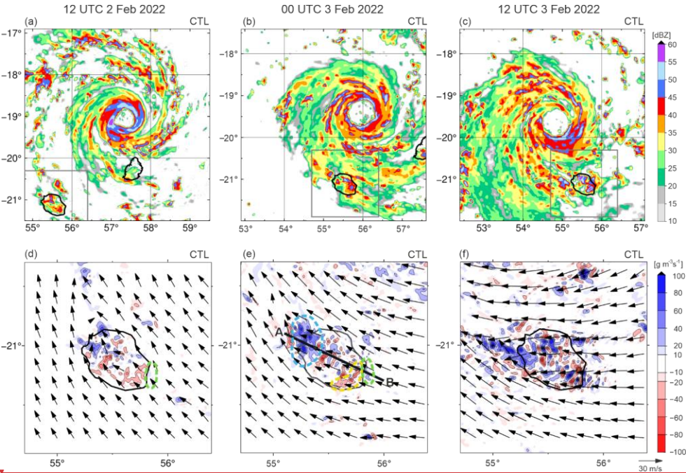
Figure 9. Horizontal distributions of CTL-simulated reflectivity at 3 km above sea level in panels (a)–(c) and low-level moisture flux convergence below 3 km in panels (d)–(f) at 12 UTC on 2 February, 00 and 12 UTC on 3 February 2022. The inner boxes in panels (a)–(c) indicate the domains shown in panels (d)–(f). The black solid line in panel (e) marks the location of the vertical cross-section
