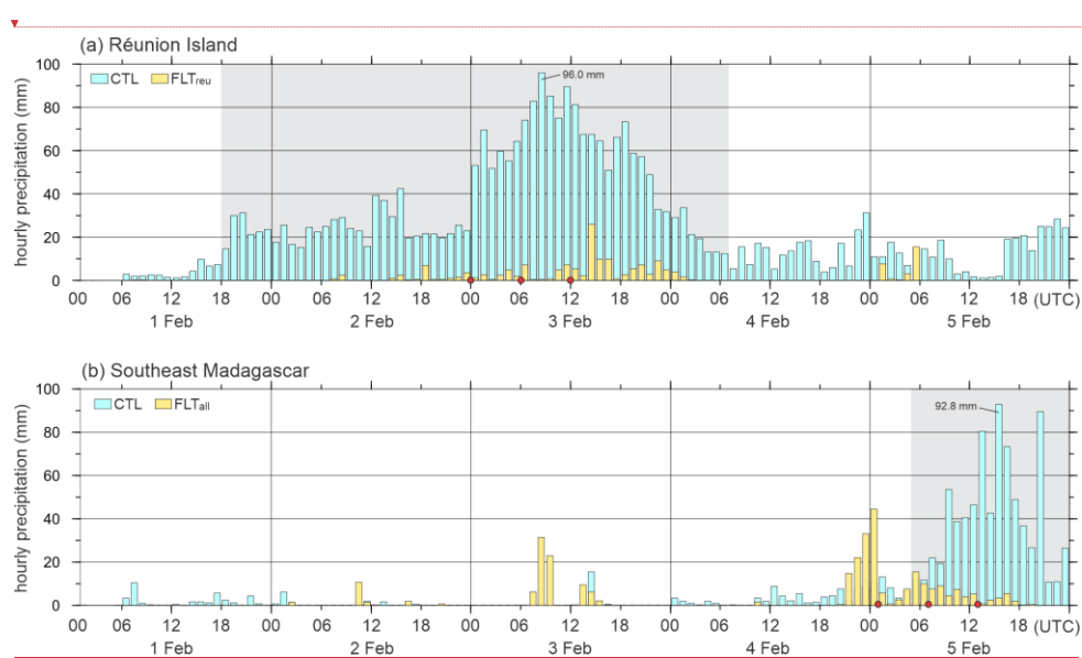
400 Figure 8. Temporal evolution of the simulated maximum precipitation within the analysis domains: (a) the Réunion Island region, from the CTL (light blue bars) and FLT_{reu} (yellow bars) experiments, and (b) the eastern Madagascar region, from the CTL (light blue bars) and FLT_{all} (yellow bars) experiments. The horizontal extent of the analysis domains is shown by the boxes in Fig. 7. Red circles along the x-axis indicate the selected times presented in Figs. 9, 10, and 12. The grey-shaded areas highlight period during which precipitation \geq 10 \text{ mm h}^{-1} persists in CTL experiment. Results of the first 6 hours of the spin-up period were excluded from the analysis.
