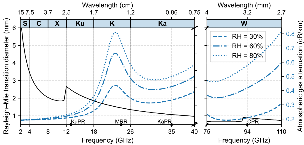
Figure E1. Frequency dependence of the Rayleigh-Mie Rayleigh-Mie transition diameter and atmospheric gas attenuation (oxygen and water vapour vapor ) across microwave radar bands. The bottom x-axis shows frequency (GHz) and the top axes show the corresponding wavelengths (cm and mm), with S, C, X, Ku, K, Ka, and W bands indicated. The operating frequencies of TRMM and GPM KuPR, MRR, GPM KaPR, and CloudSat and EarthCare EarthCARE CPR radars are annotated. The black solid curve (left y-axis) represents the drop diameter at which scattering transitions from the Rayleigh to the Mie regime. The transition is defined as the diameter at which the pyTmatrix-simulated pytmatrix-simulated normalized radar backscattering cross section \frac{\sigma_H^b(D)}{\pi(D/2)^2} - \frac{\sigma_H^b(D)}{\pi(D/2)^2} deviates by more than 10% from the Rayleigh approximation. The blue dashed, dash-dotted, and dotted curves (right y-axis) show atmospheric gas attenuation ( \text{dB km}^{-1} ) for relative humidity (RH) levels of 30%, 60%, and 80%, respectively. Gaseous attenuation increases with both frequency and humidity, exhibits a pronounced peak near the 22-24 22-24 GHz water vapor absorption band, and becomes very strong in the oxygen absorption region within the V band ( 40-75 40-75 GHz; not shown). Strong gaseous attenuation also occurs at W band frequencies.
