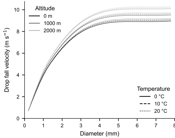
Figure B1. Rain-drop fall velocity as a function of drop diameter, altitude, and temperature estimated using the Beard terminal fall velocity-fall-velocity model.
