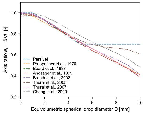
Figure A1. Comparison of the drop axis ratio as a function of drop diameter for parametrizations parameterizations implemented in disdrodb.
