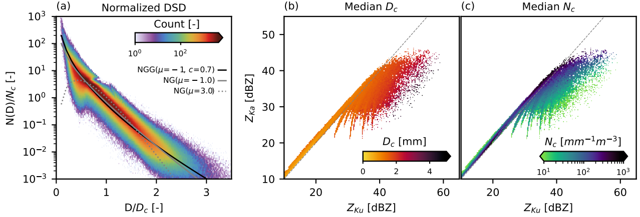
Figure 9. Double-moment normalization analysis and radar relationships derived from 15 years of disdrometer measurements at Whitworth Meteorological Observatory. (a) Observed double-moment normalized DSDs expressed as N(D)/N_c versus D/D_c , using moments i = 3 and j = 4 . Colors indicate the frequency of occurrence (counts). The solid gray and black curves show fitted normalized gamma (NG) and normalized generalized gamma (NGG) models, while the gray dashed line shows the NG parametric model (with \mu = -3 ) \mu = 3 currently adopted in GPM DPR retrievals. (b) Relationship between Ku-band reflectivity Z_{Ku} and Ka-band reflectivity Z_{Ka} , with color shading indicating the observed median general characteristic diameter D_c . D_c grows monotonically with increasing reflectivities. (c) Relationship between Ku-band reflectivity Z_{Ku} and Ka-band reflectivity Z_{Ka} , with color shading indicating the observed median general characteristic intercept parameter N_c . Retrieval of N_c becomes particularly challenging for Z_{Ku} < 30 dBZ, where large variation variations in N_c produces produce only small changes in Z_{Ka} . This region is associated with negative dual-frequency ratio (DFR) values and corresponds to the area above the 1:1 dashed gray line.
