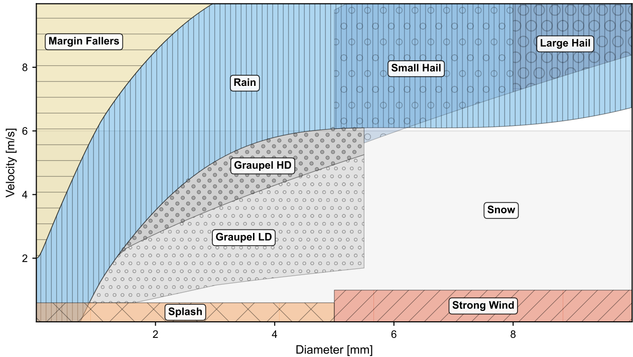
Figure 4. Schematic illustration of particle size-velocity size-velocity spectrum partitioning, inspired by Friedrich et al. (2013) and derived from theoretical fall velocity-particle velocity-particle size relationships (see Appendix B). The hydrometeors hydrometeor masks are automatically adjusted according to the station altitude.
