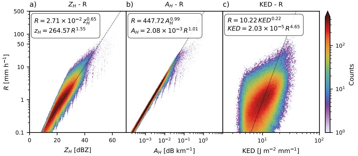
Figure 7. Two-dimensional histograms illustrating power-law relationships between rainfall rate R and selected radar and microphysical variables derived from 15 years of disdrometer measurements at Whitworth Meteorological Observatory. Colors indicate the frequency of occurrence (counts), while black dashed lines represent the fitted power-law relationships shown in each panel. Power-law relationships are fitted by default using the robust RANSAC algorithm (Fischler and Bolles, 1981) applied to the median values within each bin; weighted nonlinear least squares is also available as an alternative. Inverse power-law relationships are obtained by algebraic inversion of the fitted models. (a) C-band horizontal reflectivity factor Z_{H,C} versus R . The z_H in the power-law expressions denotes reflectivity in linear units, and the regression is performed on z_H . (b) C-band horizontal specific attenuation A_{H,C} versus R . (c) Kinetic energy density (KED) versus R . Similar diagnostic plots, including additional radar variables at multiple frequency bands and kinetic energy relationships, are automatically generated by disdrodb as part of the station summary figures.
