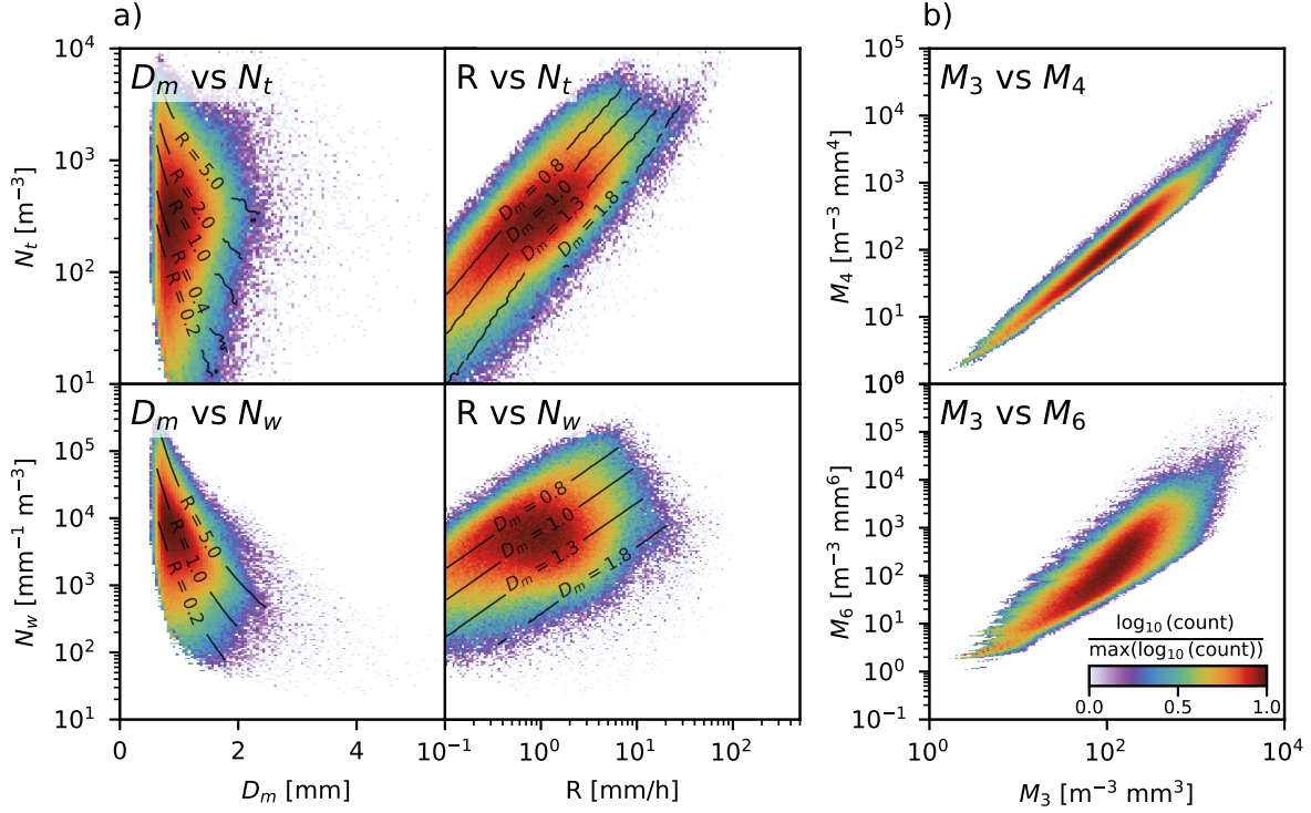
Figure 6. Two-dimensional histograms illustrating the relationships among DSD bulk quantities derived from 15 years of measurements collected by a Thies LPM disdrometer installed at the Whitworth Meteorological Observatory, Manchester University, United Kingdom. Colors represent the normalized logarithmic frequency of occurrence. a) Relationships among D_m , N_t , N_w and R . Black contour lines indicate median iso- R values in the left column and median iso- D_m values in the right column. A decreasing trend of N_w with increasing D_m is observed, while R generally increases with both D_m and N_t . No clear relationship is evident between D_m and N_t , nor between N_w and R . (b) Relationships between the third moment M_3 and higher-order moments M_4 (top) and M_6 (bottom), commonly used in double-moment DSD normalization approaches (see Appendix D). Similar diagnostic plots exploring additional DSD bulk relationships are automatically generated by disdrodb as part of the station summary figures.
