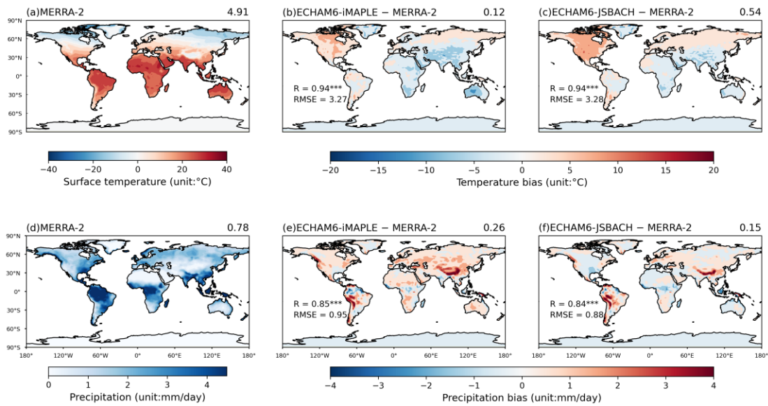
921 Figure 6. Spatial distributions of (a) surface temperature (T, °C) and (d) precipitation 922 (PREC, mm/day) from MERRA-2 reanalyses, biases of (b, e) ECHAM6-iMAPLE and 923 (c, f) ECHAM6-JSBACH relative to MERRA-2. Both model simulations and MERRA- 924 2 reanalyses are averaged for the period of 2005-2014. The spatial R and RMSE 925 between simulations and observations are shown in the lower left corner of simulation 926 panels. The area-weighted mean (or mean biases) T and PREC are indicated at the top 927 of each panel.
