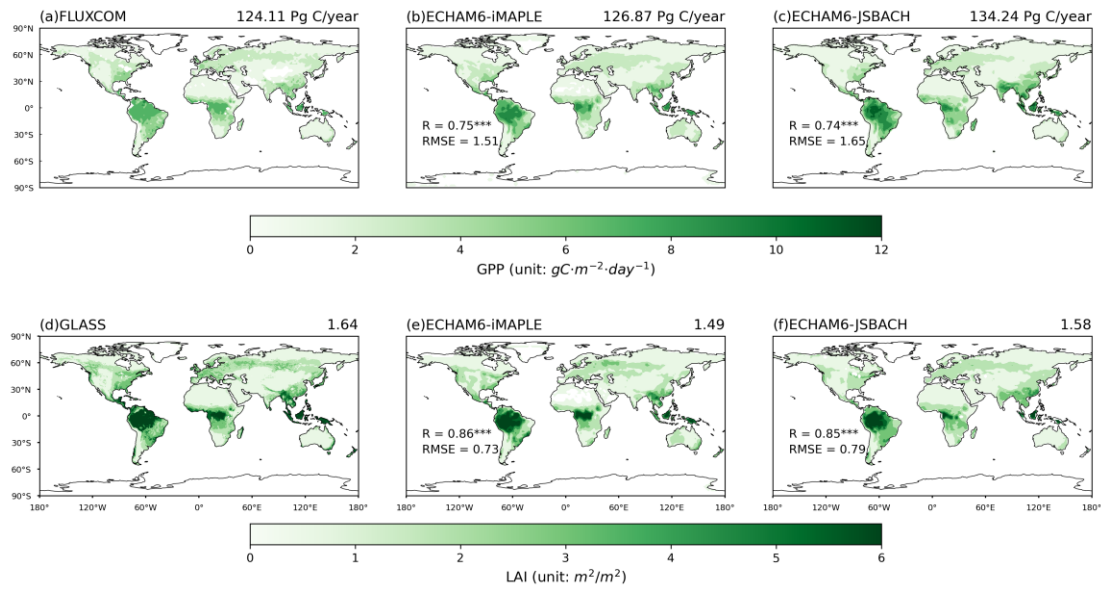
Figure 2. Spatial distributions of (a) gross primary productivity (GPP, g\ C\ m^{-2}\ day^{-1} ) from FLUXCOM and (d) leaf area index (LAI, m^2/m^2 ) from GLASS, compared with simulations from (b, e) ECHAM6-iMAPLE and (c, f) ECHAM6-JSBACH. Both model simulations and benchmark/observational datasets are averaged for the period of 2005-2014. The spatial correlation coefficient ( R ) and root mean square error (RMSE) between simulations and the corresponding observations are shown in the lower left corner of the simulation panels.
