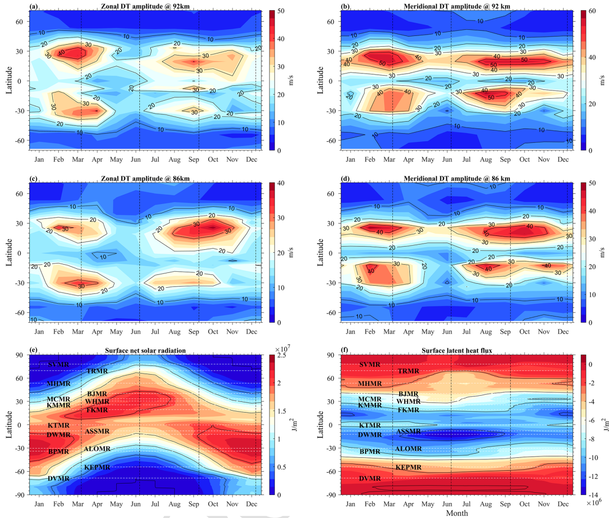
Figure 7. (a–d) Latitude–seasonal variations in the zonal and meridional diurnal tidal amplitudes at 92 and 86 km derived from the fifteen meteor radars. (e–f) Surface net solar radiation and surface latent heat flux derived from the ERA5 reanalysis produced by the European Centre for Medium-Range Weather Forecasts (ECMWF). Note that the colorbar scales differ among panels.
