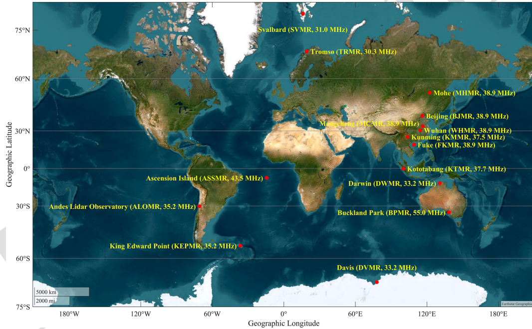
Figure 1. The locations of the Davis Station (DVMR, 68.6° S, 77.9° E), King Edward Point Station (KEPMR, 54° S, 36° W), Buckland Park (BPMR, 34.6° S, 138.5° E), Andes Lidar Observatory (ALOMR, 30.3° S, 70.7° W), Darwin (DWMR, 12.3° S, 130.5° E), Ascension Island (ASSMR, 7.9° S, 14.4° W), Kototabang (KTMR, 0.2° S, 100.3° E), Fuke (FKMR, 19.5° N, 109.1° E), Kunming (KMMR, 25.6° N, 103.8° E), Wuhan (WHMR, 30.6° N, 114.4° E), Mengcheng (MCMR, 33.4° N, 116.5° E), Beijing (BJMR, 40.3° N, 116.2° E), Mohe (MHMR, 53.5° N, 122.3° E), Tromsø (TRMR, 69.6° N, 19.2° E), and Svalbard (SVMR, 78.2° N, 16° E).
