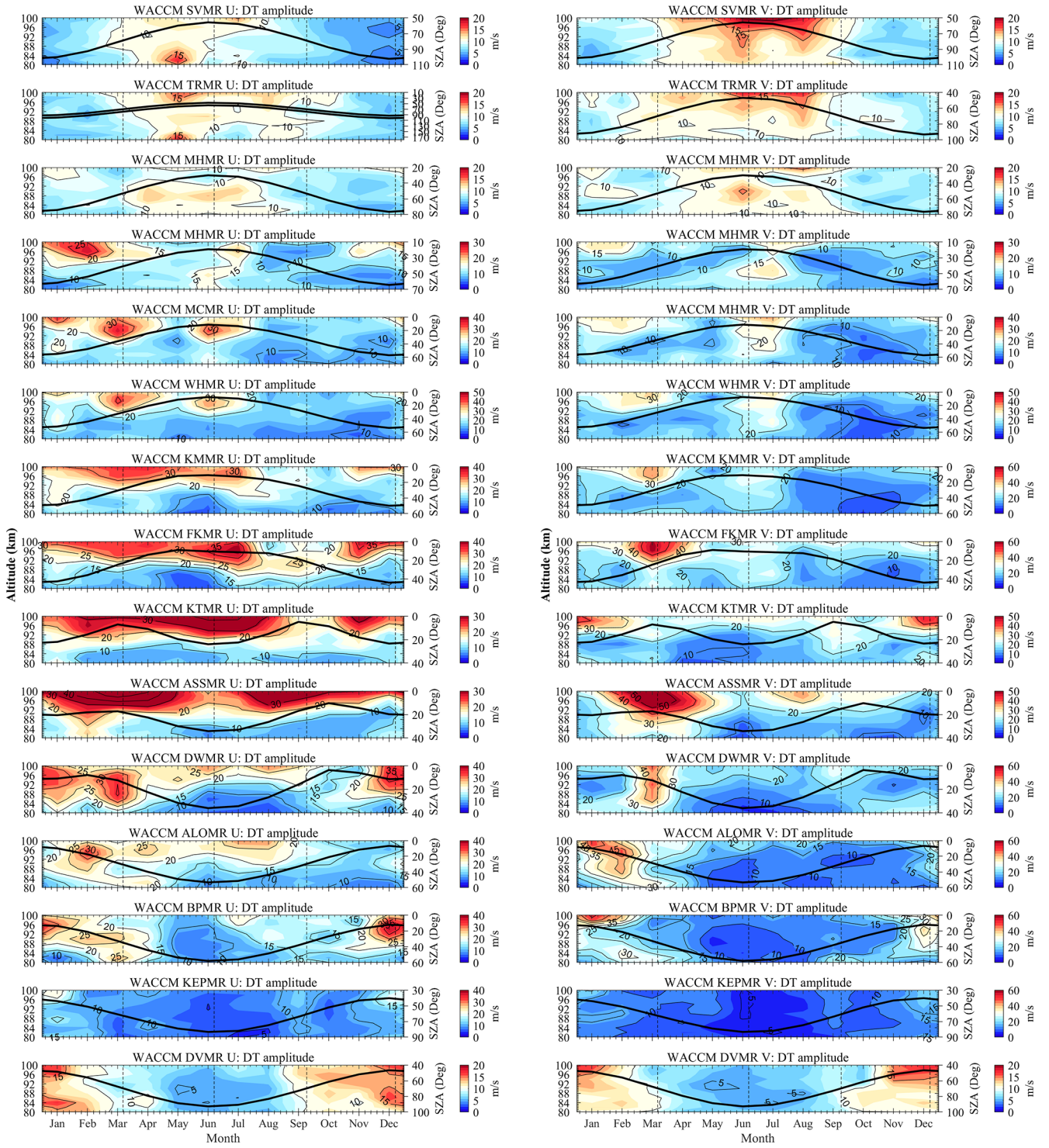
Figure 5. Same as Fig. 2, but for the monthly mean amplitudes of composite zonal (left column) and meridional (right column) diurnal tidal (DT) components obtained from the SD-WACCM.
