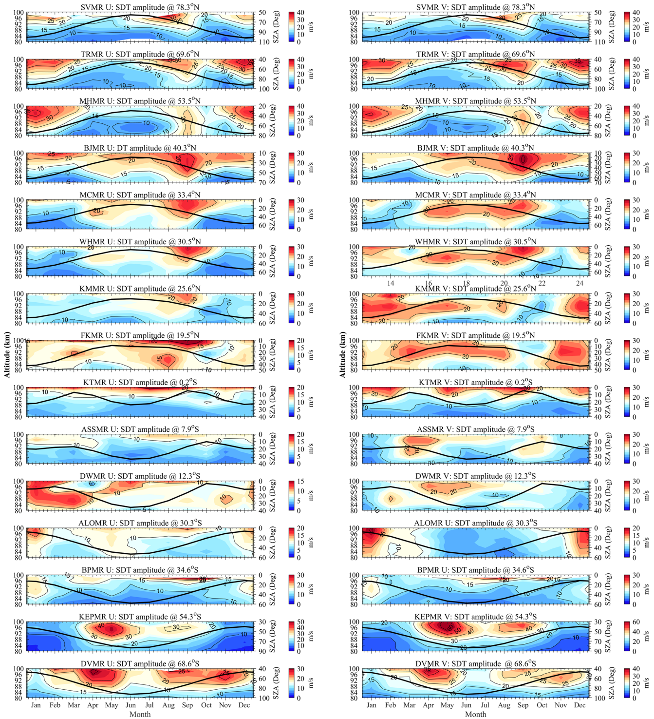
Figure A4. Monthly mean amplitudes of the composite zonal ( U ; left columns) and meridional ( V ; right columns) semidiurnal tidal (SDT) components derived from fifteen meteor radars. Note that the colorbar scales differ among panels. The black solid lines denote the solar zenith angle at local noon (12:00 LT), shown on the right axes. The vertical black dashed lines indicate the spring and autumn equinoxes and the summer and winter solstices.
