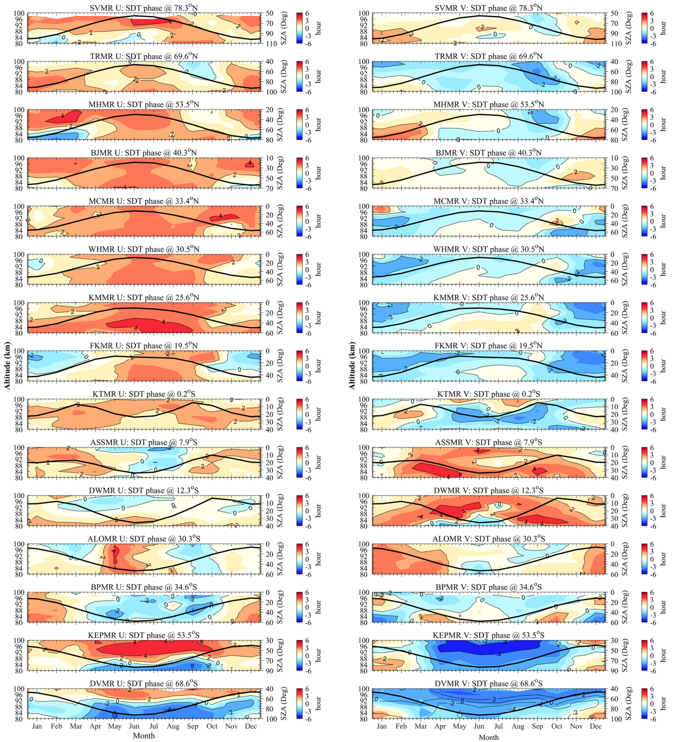
Figure A5. Same as Fig. A4, but for the monthly mean phases of composite zonal (left column) and meridional (right column) semidiurnal tidal (SDT) components derived from fifteen meteor radars.
