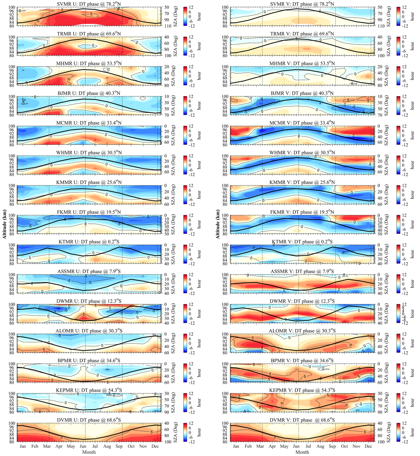
Figure 3. Same as Fig. 2, but for the monthly mean phases of composite zonal (left column) and meridional (right column) diurnal tidal (DT) components.
