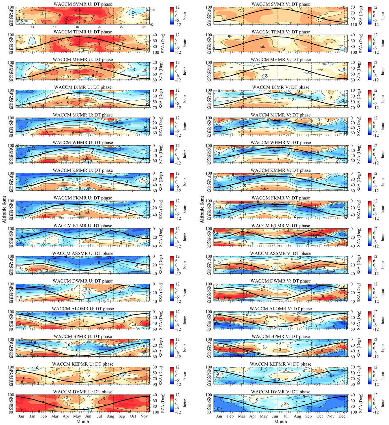
Figure 6. Same as Fig. 3, but for the monthly mean phases of composite zonal (left column) and meridional (right column) diurnal tidal (DT) components obtained from the SD-WACCM.
