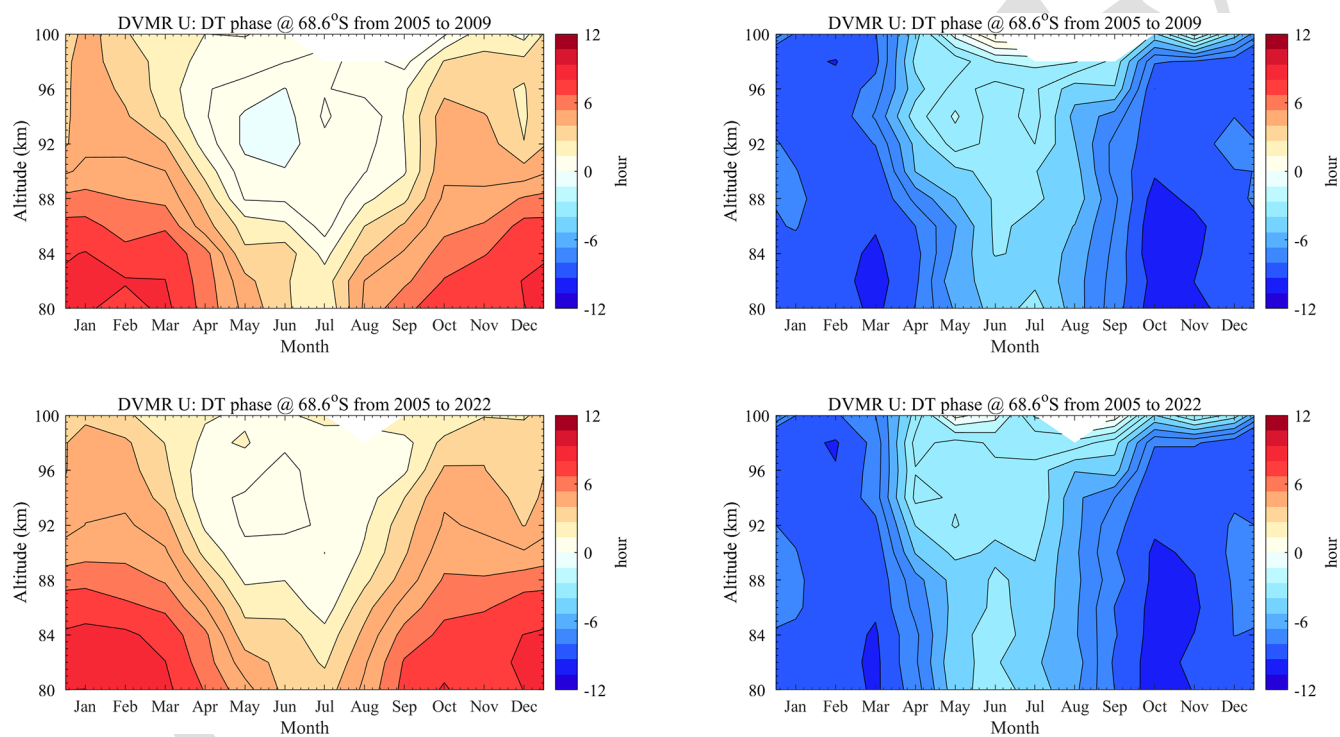
Figure A3. Same as Fig. A2, but for the meridional amplitude and phase.
