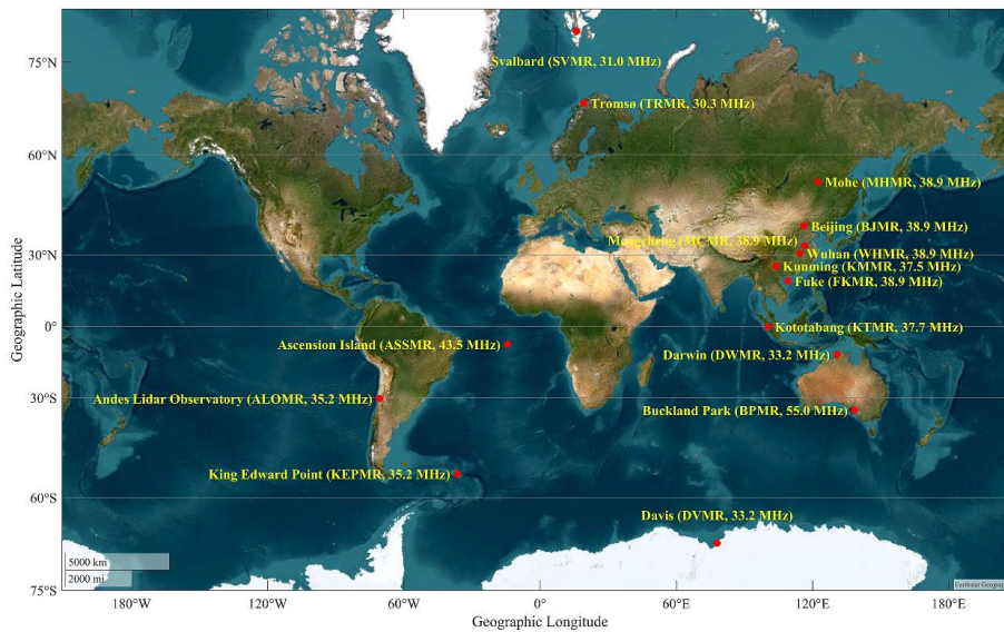
Figure 1. The locations of the Davis Station (DVMR, 68.6°S, 77.9°E), King Edward Point Station (KEPMR, 54° S, 36° W), Buckland Park (BPMR, 34.6°S, 138.5°E),
