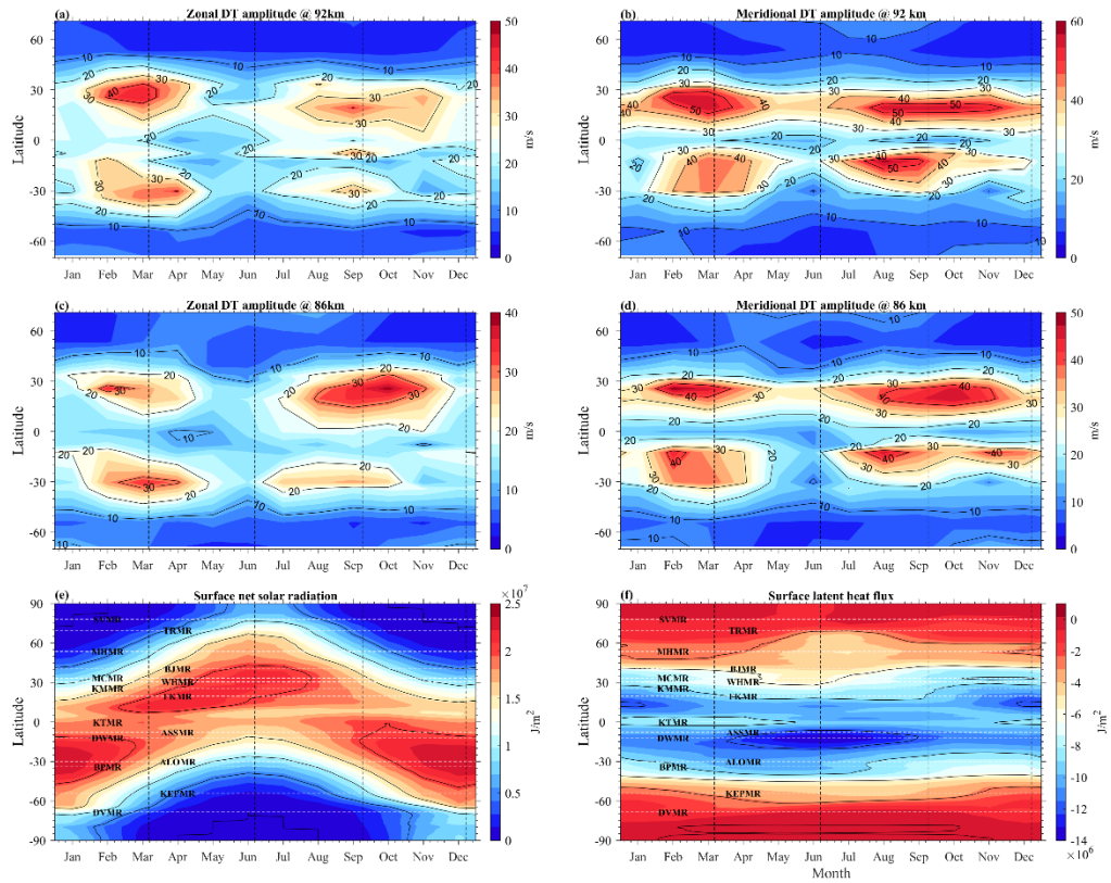
Figure 67. (a–d) Latitude–seasonal variations in the zonal and meridional diurnal tidal amplitudes at 92 and 86 km were obtained derived from the fifteen meteor radars. (e) and (f) Surface net solar radiation and Surfacesurface latent heat flux derived from the ERA5 reanalysis produced by the European Centre for Medium-Range Weather Forecasts (ECMWF-). Note that the values of colorbar are different scales differ among panels.
