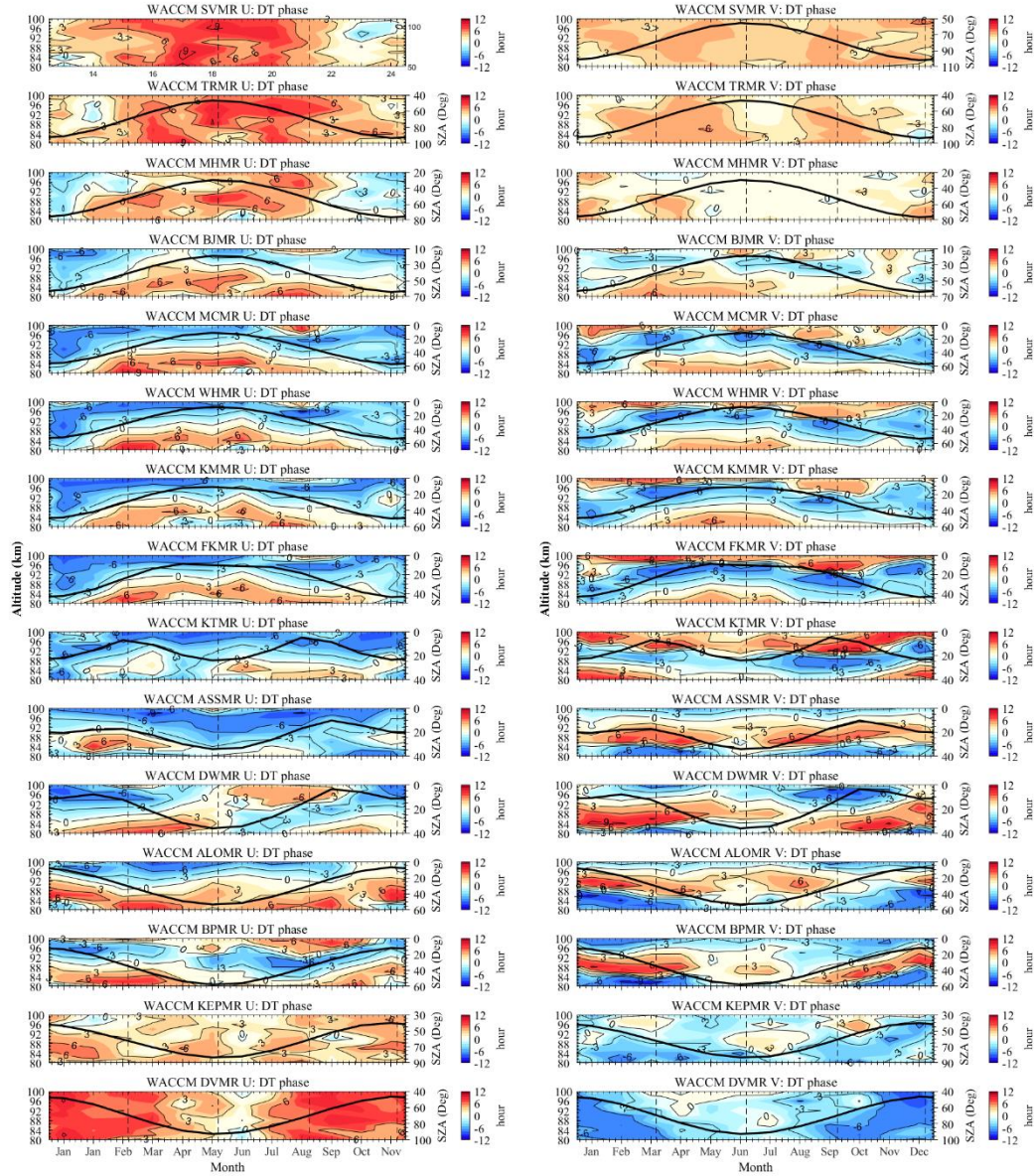
Figure 56. Same as Figure 3, but for the monthly mean phases of composite zonal (left column) and meridional (right column) diurnal tidal (DT) components obtained from the SD-WACCM.
