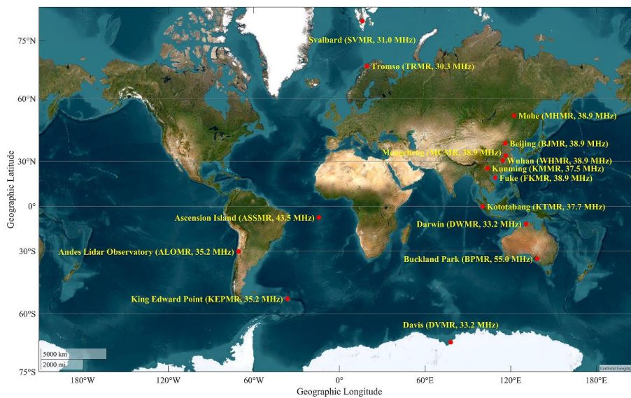
Figure 1. The locations of the Davis Station (DVMR, 68.6°S, 77.9°E), King Edward
