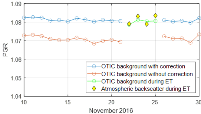
Figure 4: Daily mean OTIC PGR without (red) and with (blue) MSC using Eq. (56). The onboard PGR calibration using the PD was conducted over 22–25 November 2016 (green). Yellow diamonds show the corresponding daily mean PGRs derived from atmospheric backscatter signals within 8.2–20.2 km in the OTIC columns during the ET with the PD inserted.
