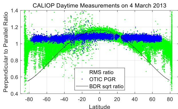
Figure 3: One day of CALIOP observations acquired on 4 March 2013 , comprising a total of 14 daytime granules, one of which is the granule shown in Fig. 2. The green dots represent the RMS ratio, the blue dots denote the OTIC PGR, and the solid dark curve shows the square root of the scaled molecular-scattering BDR depolarization ratio at the surface. The theoretical BDR curve follows the upper (in the tropics) and lower (high latitudes) envelopes of the RMS ratios where molecular scattering dominates.
