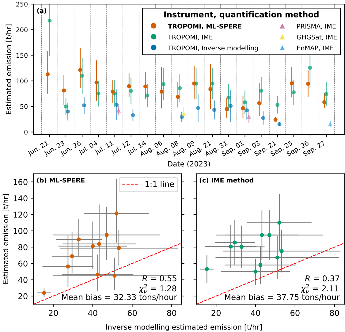
Figure 5. a Time series of daily estimated methane emission rates for the Karaturun East oilfield blowout. TROPOMI inverse modeling estimates and high-resolution satellite IME estimates are taken from Guanter et al. (2024). ML-SPERE data points are median values of the estimated posterior distribution of estimated emissions. Errorbars shown are \pm 1\sigma , with the exception of error bars for ML-SPERE estimates, which extend from the 16th to the 84th percentile of the posterior distribution of emission estimates (all statistics are given in Table A3) We choose to represent error bars for ML-SPERE with percentiles to show the skewed shape of the posterior distribution of the estimate (e.g., see Fig. A6a). b ML-SPERE estimates of the daily emission rate compared to the TROPOMI inverse modeling estimate for that same day. c IME estimates of the daily emission rate compared to the TROPOMI inverse modeling estimate for that same day.
