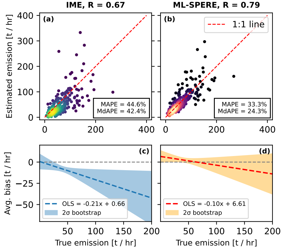
Figure A4. Estimated emission rates for simulated HYSPLIT plumes via (a) the IME method and (b) ML-SPERE as a function of true plume emission rates, filtered to only include scenes from the test set where the emission source location is contained within the estimated plume mask. The colormaps represent the relative density of the visualised data. We visualise bootstrapped ordinary least squares (OLS) regression lines for emission rate estimates from both the IME method (in c) and ML-SPERE (in d). The 1:1 line is subtracted in c and d to show average bias.
