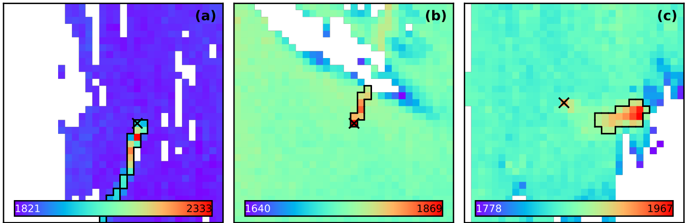
Figure A3. A few examples of test set plumes and their derived plume masks outlined in black. Emission source locations are shown with a black x. In a , the plume is easily delineated. In b , the head of the plume is captured, but missing data prevents the rest of the plume from being included in the mask. In c , background variability results in only some of the plume being successfully delineated, and the source pixel is not included in the mask. Colorbar values are methane concentrations in ppbv.
