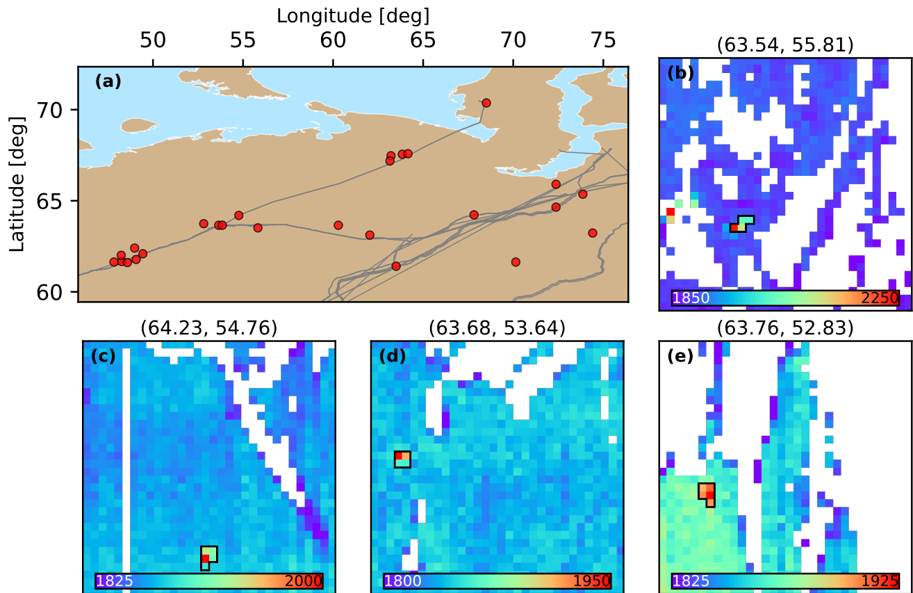
Figure A10. a Locations for the plumes in northern Russia for which ML-SPERE estimates exhibit the largest log-ratios when compared to the IME method, shown in red dots. Pipelines from the Global Energy Monitor are shown with grey lines. Examples of methane observations are shown in panels b-e , and colorbar values show methane concentrations in ppbv. Latitude-longitude coordinates of the most upwind pixel within the plume masks are shown in the titles of panels b-e .
