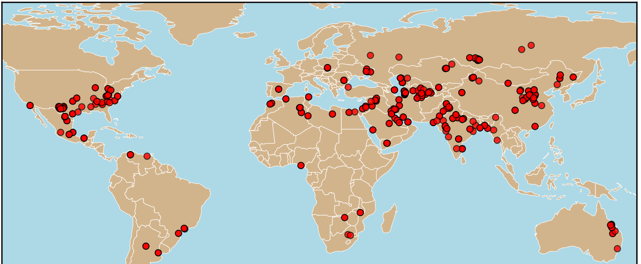
Figure A2. 438 test set plumes simulated at 224 unique global locations with HYSPLIT.
