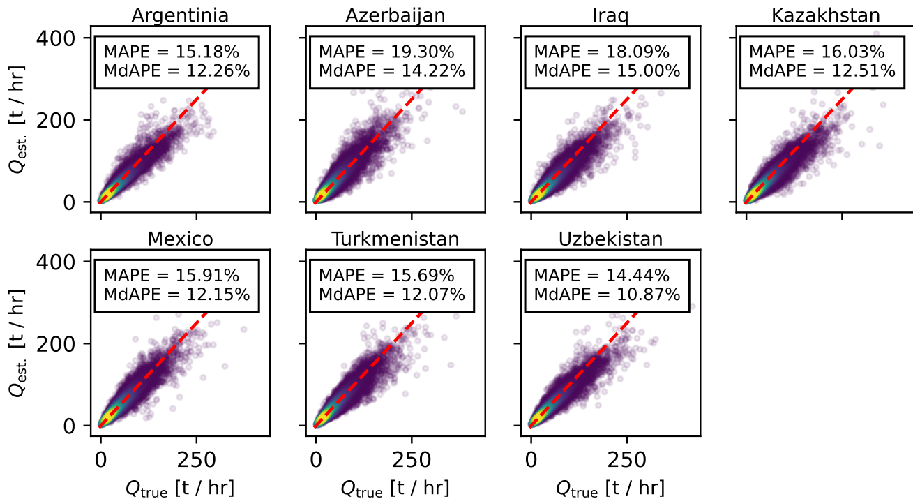
Figure A7. Visualizations of ML-SPERE estimated emission rates Q_{\text{est.}} vs true emission rates Q_{\text{true}} for each of the K-fold test sets. Values for MAPE and MdAPE are shown in each panel, and the red dashed lines show the 1:1 line. The colormaps represent the relative density of the visualised data.
