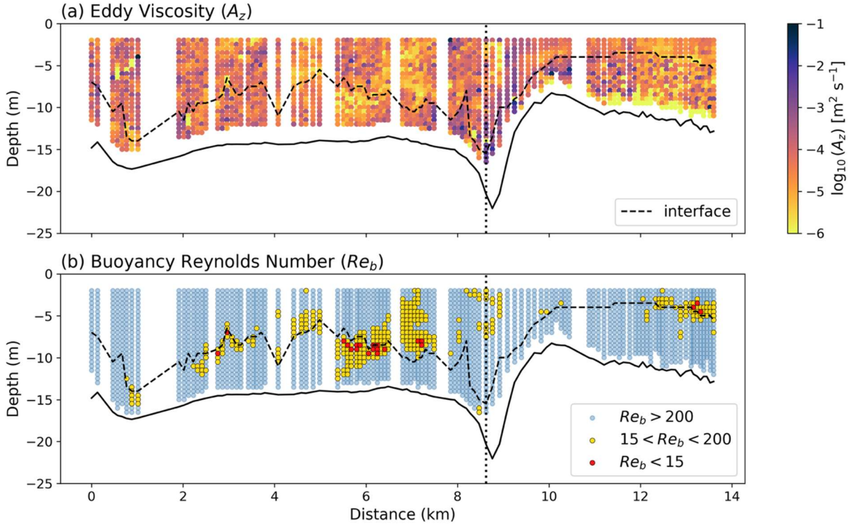
535 Figure 10. Spatial distributions of (a) the vertical eddy viscosity ( A_z , \text{m}^2 \text{s}^{-1} ), and (b) the buoyancy Reynolds number ( Re_b ). The dashed line indicates the interface position between layers. The vertical dotted line marks the position of the mouth (inlet). Distance (km) is measured from the first upstream profile within the channel.
