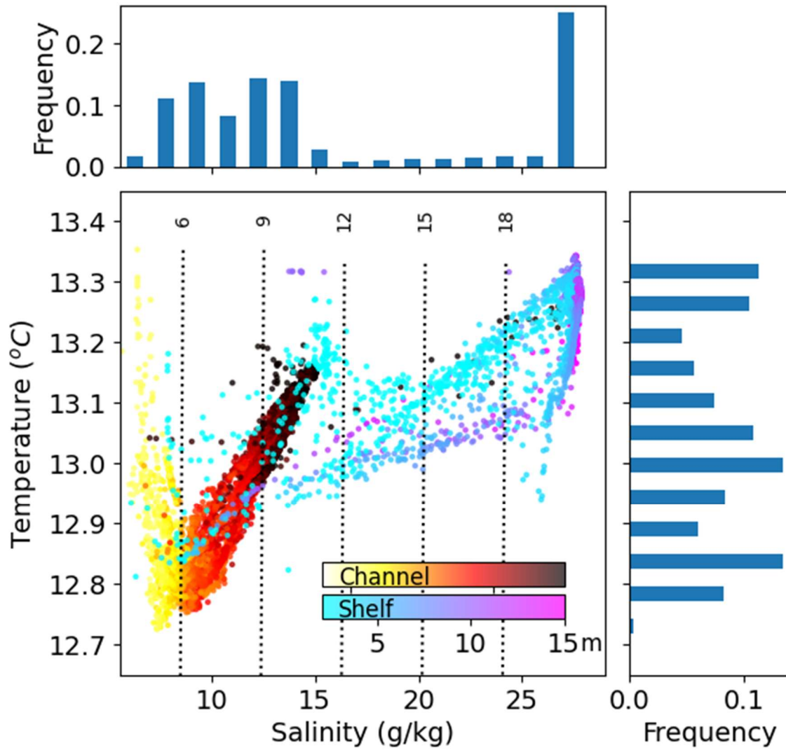
Figure 5. Temperature–Salinity (T–S) diagram and frequency histograms of salinity (top) and temperature (right) for the Drift segment. The central panel shows temperature (°C) versus salinity (g kg -1 ), with dotted vertical lines indicating density anomaly ( \sigma_\theta ) values. The colour bar distinguishes data from the Channel (warm tones) and the Shelf (cold tones), with shading representing the sampling depth (m).
