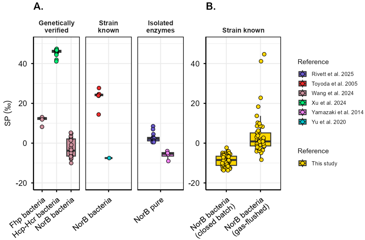
Figure 5. Site preference (SP) of N_2O produced by three classes of N_2O -forming systems. A) Literature-derived SP values grouped by system type: left, intact denitrifiers with genetically verified N_2O -forming enzymes, where both strain identity and the active enzyme system (NorB, Hcp–Hcr, or Fhp) were confirmed (Xu et al., 2024; Wang et al., 2024); center, intact denitrifiers, strains are known but additional N_2O -forming pathways cannot be excluded (Toyoda et al., 2005; Yu et al., 2020); and right, isolated enzyme assays, in which purified NorB was studied directly, yielding enzyme-specific SP values (Yamazaki et al., 2014; Rivett et al., 2025). B) SP values obtained in this study for intact denitrifiers with known strain background, shown separately for closed-batch and gas-flushed incubation modes. Boxplots show the distribution of SP values within each category; horizontal bars indicate mean \pm standard deviation. Gas-flushed incubations represent time-resolved SP measurements, whereas closed-batch incubations reflect SP integrated over the accumulated N_2O pool.
