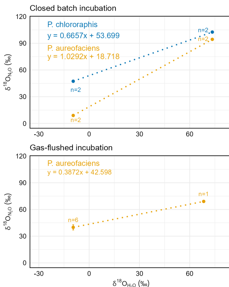
3 4 Figure 8. \delta^{18}\text{O-N}_2\text{O} as a function of \delta^{18}\text{O-H}_2\text{O} for both endpoint (closed batch) and gas-flushed incubations of P. aureo- 5 faciens (NirK) and P. chlororaphis (NirS). The regression slope from incubations in natural-abundance ( \delta^{18}\text{O-H}_2\text{O} \approx - 6 9.5 ‰) and ^{18}\text{O} -enriched water ( \delta^{18}\text{O-H}_2\text{O} \approx +68.3 ‰ or +73.5 ‰) reflects the extent of oxygen-atom exchange be- 7 tween nitrite and water during stepwise \text{N}_2\text{O} formation. The intercept represents the \delta^{18}\text{O-N}_2\text{O} value expected for incu- 8 bation in water with \delta^{18}\text{O-H}_2\text{O} = 0 ‰, and thus reflects the combined effects of the nitrite–water equilibrium isotope 9 effect and the branching isotope effect for the reaction of \text{NO}_2^- \rightarrow \text{N}_2\text{O} , plus any contribution from nitrate-derived oxy- 10 gen that is not removed by nitrite–water exchange. The slope for P. aureofaciens in gas-flushed incubation ( 0.38 ) indicates 11 partial exchange ( 38 %), whereas endpoint incubations for P. aureofaciens and P. chlororaphis suggest near-complete 12 ( \approx 100 %) and partial exchange ( \approx 66 %), respectively.
