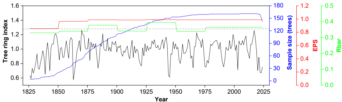
Fig. 3 Standard TRW chronology and sample size for Schrenk spruce in the eastern Tianshan Mountains (chronology: black line; sample size: blue line; running Rbar: green line; running EPS: red line; grey line is the threshold of EPS 0.85).
