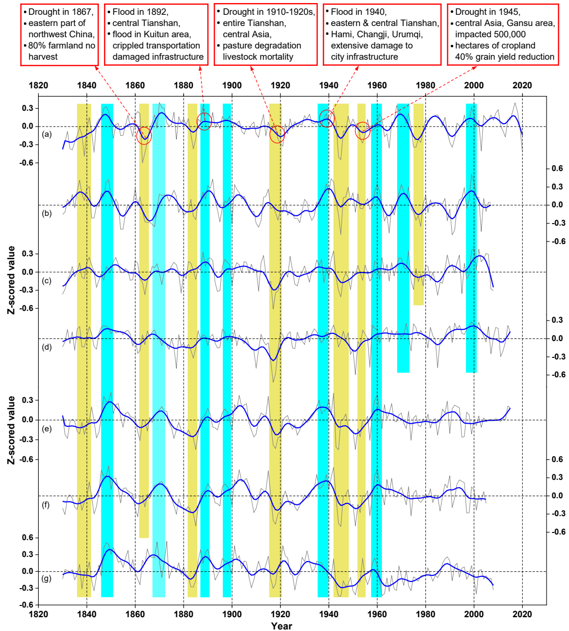
Fig. 9 Comparison of multiple hydroclimatic reconstructions across the Tianshan Mountains from different studies: (a) precipitation reconstruction from this study; (b) precipitation reconstruction for the eastern Tianshan Mountains (Zhang et al., 2015); (c) PDSI drought reconstruction for the inner Tianshan Mountains (Zhang et al., 2017); (d) SPEI drought reconstruction for the central Tianshan Mountains (Ma et al., 2025); (e) PDSI drought reconstruction for the Tianshan Mountains (Wang et al., 2021); (f) SPEI drought reconstruction for the central Tianshan Mountains (Jiang et al., 2017); and (g) SPEI drought reconstruction for the central Tianshan Mountains (Xu et al., 2014). The historical archives of climate events are shown in the red boxes on the top.
