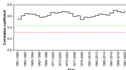
Fig. 6 The moving correlation between the TRW chronology and July – June precipitation over the period 1961–2020. The horizontal red and dashed green lines represent the 0.05 and 0.01 significance levels, respectively.
