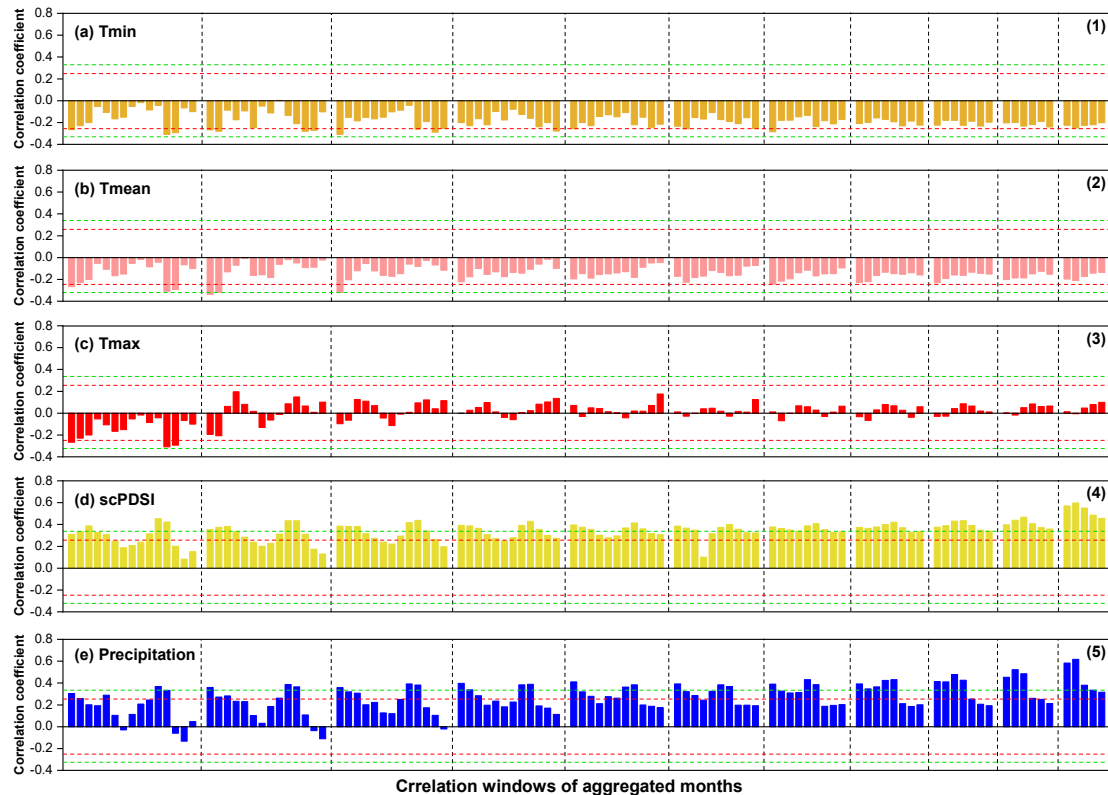
Fig. S1 Correlations between the tree-ring width chronology and aggregated monthly climate variables (temperature, precipitation, and scPDSI) were examined over windows of 2 to 12
