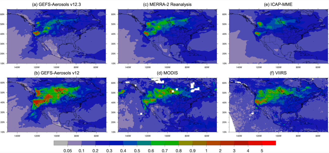
171 Figure 2. Monthly mean Day-1 AOD forecasts for August 2021 over North America from (a) GEFS-Aerosols v12.3, (b) GEFS- 172 Aerosols v12 compared with (c) MERRA-2 reanalysis; (d) MODIS; (e) ICAP multi-model ensemble; and (f) VIIRS observation. 173 All panels show AOD at 550 nm.
