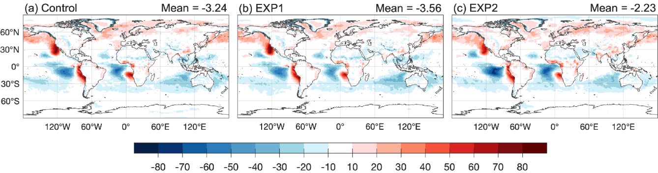
260 Figure 10. Six-year averaged (2012–2017) TOA net radiative flux bias compared with CERES for August in UFS-Chem for the 261 (a) Control, (b) EXP1, and (c) EXP2 experiments.
