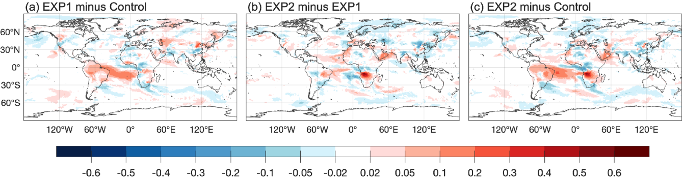
Figure A2. Differences in Total AOD for August 2016 in UFS-Chem. (a) Effect of aerosol radiative feedback (EXP1 minus Control). (b) Effect of aerosol indirect feedback (EXP2 minus EXP1). (c) Combined effect of aerosol radiative and indirect feedback (EXP2 minus Control).
