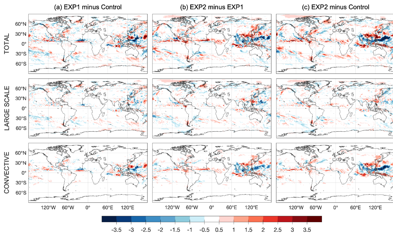
296 Figure 13. Six-year averaged (2012–2017) differences in total precipitation (top row; \text{mm day}^{-1} ), large-scale precipitation (middle 297 row; \text{mm day}^{-1} ) and convective precipitation (bottom row; \text{mm day}^{-1} ) for August in UFS-Chem. (a) Effect of aerosol radiative 298 feedback (EXP1 minus Control). (b) Effect of aerosol indirect feedback (EXP2 minus EXP1). (c) Combined effect of aerosol 299 radiative and indirect feedback (EXP2 minus Control).
