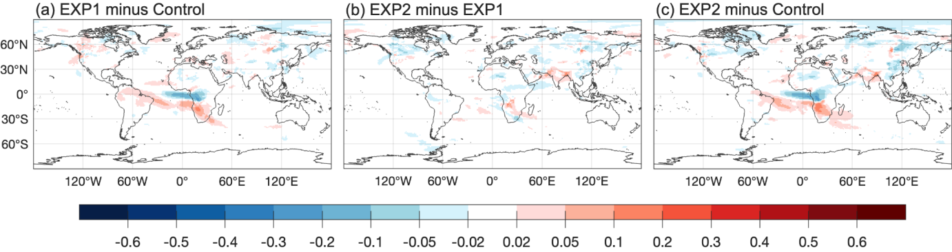
Figure A3. Six-year averaged (2012–2017) differences in Total AOD for August in UFS-Chem. (a) Effect of aerosol radiative feedback (EXP1 minus Control). (b) Effect of aerosol indirect feedback (EXP2 minus EXP1). (c) Combined effect of aerosol radiative and indirect feedback (EXP2 minus Control).
