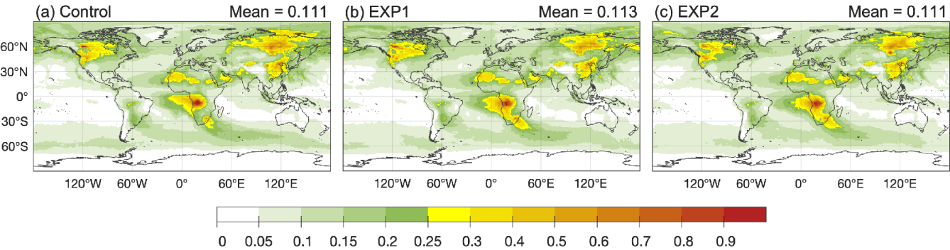
250 Figure 9. The same as in Figure 8, but for AOD RMSE.
