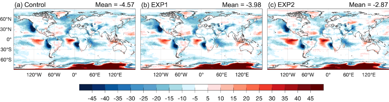
272 Figure 11. Six-year averaged (2012–2017) cloud fraction bias (%) compared with CERES for August in UFS-Chem for the (a) 273 Control, (b) EXP1, and (c) EXP2 experiments.
