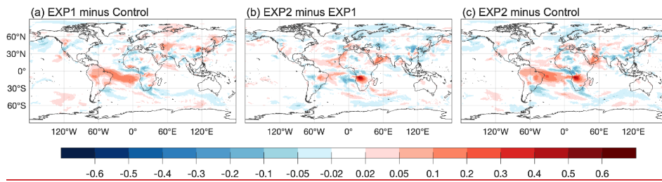
Figure A2. Differences in Total AOD for August 2016 in UFS-Chem. (a) Effect of aerosol radiative feedback (EXP1 minus Control). (b) Effect of aerosol indirect feedback (EXP2 minus EXP1). (c) Combined effect of aerosol radiative and indirect feedback (EXP2 minus Control).
