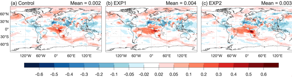
Figure 6. AOD biases relative to MERRA-2 reanalysis for August 2016 in UFS-Chem. (a) Control: aerosol radiative feedback from prescribed MERRA-2 climatological aerosol fields; (b) EXP1: aerosol radiative feedback from inline-predicted aerosols; (c) EXP2: aerosol radiative and indirect feedback from inline-predicted aerosols.
