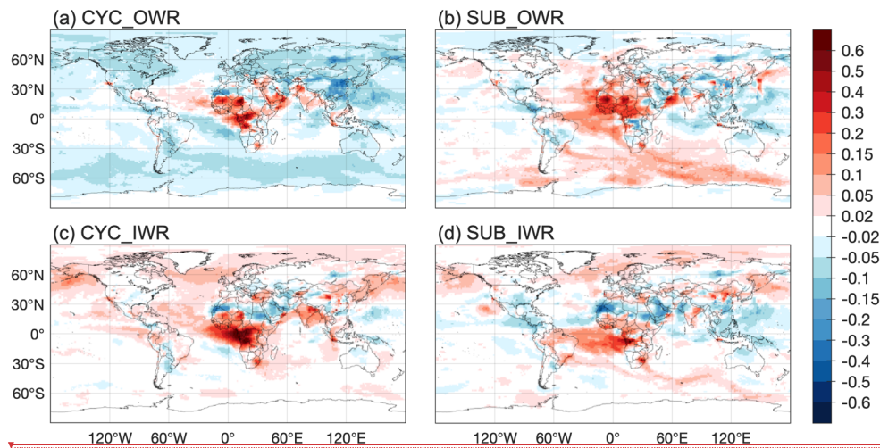
Figure 4. AOD biases with respect to MERRA-2 for the following experiments in August 2016: (a) CYC_OWR, a 24 h cycling run with offline large-scale wet removal; (b) SUB_OWR, a fully coupled subseasonal run with offline large-scale wet removal; (c) CYC_IWR, a 24 h cycling run with inline large-scale wet removal; and (d) SUB_IWR, a fully coupled subseasonal run with inline large-scale wet removal.
