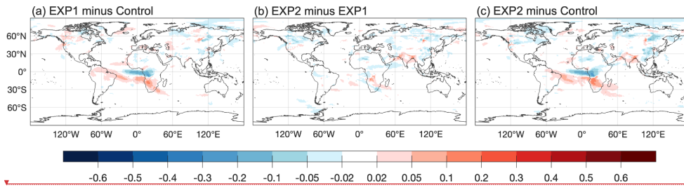
Figure A3. Six-year averaged (2012–2017) differences in Total AOD for August in UFS-Chem. (a) Effect of aerosol radiative feedback (EXP1 minus Control). (b) Effect of aerosol indirect feedback (EXP2 minus EXP1). (c) Combined effect of aerosol radiative and indirect feedback (EXP2 minus Control).
