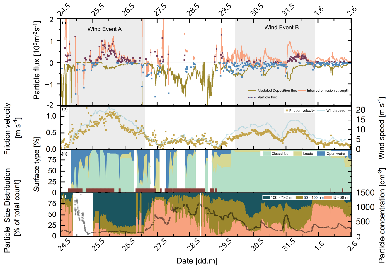
Figure 10. (a) Particle fluxes (red squares indicate net particle emission, and the blue squares indicate net particle deposition), modeled deposition flux (dark beige), and inferred emission strength (salmon-colored) from 24 May to 2 June evaluated in 20-minute intervals (in 10^6 \text{ m}^{-2} \text{ s}^{-1} ). Panel (b) shows the friction velocity ( u_* , beige, in \text{m s}^{-1} ) and wind speed (light blue, in \text{m s}^{-1} ). The grey shading in (a, b) shows the time periods when the threshold for blowing snow is exceeded. Panel (c) shows the hourly distribution of the three surface types: closed ice (turquoise), leads (beige), and open water (blue). Periods with ship speeds \geq 1 \text{ kn} are indicated in red. (d) Particle size fractions from 15 to 792 nm in three accumulated groups (left y-axis, in % of total particle number concentration) measured with a DMPS on the fourth deck of Oden and total particle number concentration ( \text{cm}^{-3} ), measured with an MCPC at the foremast (black symbols; right y-axis).
