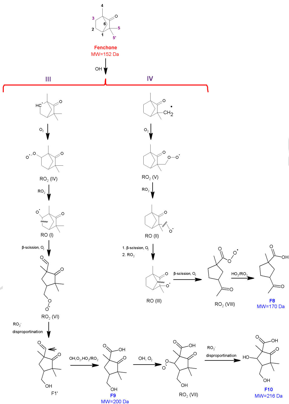
Scheme 2. Proposed mechanism for the OH reaction with fenchone. Terpenoic acids detected with LC-ToF/MS are highlighted in bold blue font. TS1
