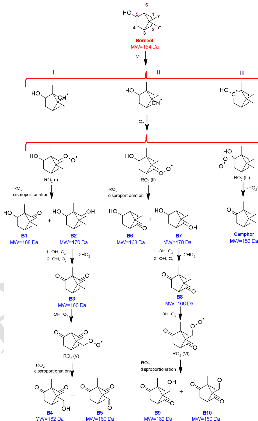
Scheme 3. Proposed mechanism of borneol (BNL) + OH reaction (R2). The detected products are highlighted in bold blue font. The formation of all possible isomers is not included for clarity. The mechanism of Reaction (R2) is continued in Schemes 4 and 5 – formation of TACs.
