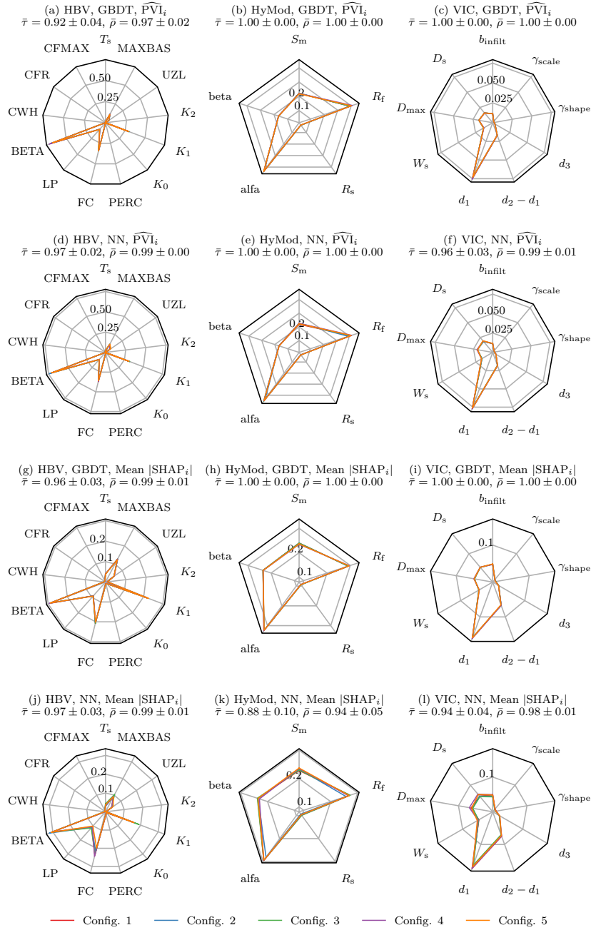
Figure 2. Sanity check of feature importance estimates for GBDT and NN metamodels across five overfitting configurations (see Table 2). Panels (a–c) show \widehat{PVI}_i and panels (g–i) show mean |\text{SHAP}_i| for the GBDT metamodel applied to HBV, HyMod, and VIC, respectively, while panels (d–f) and (j–l) show the corresponding results for the NN metamodel. Each coloured line represents a different model configuration. Panel titles report the mean \pm standard deviation of pairwise Kendall \tau and Spearman \rho correlation between the importance vectors of the five configurations. The strong overlap of importance curves across configurations, supported by high \bar{\tau} and \bar{\rho} estimates, indicates that the feature importance estimates are robust to overfitting.
