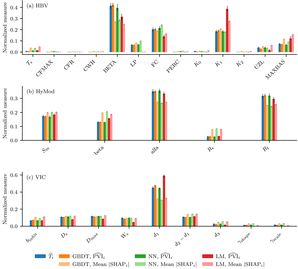
Figure 4. Parameter rankings for (a) HBV, (b) HyMod, and (c) VIC. Bars show normalized \hat{T}_i from variance-based GSA, normalized \widehat{PVI}_i estimates, and normalized mean |SHAP_i| with \hat{T}_i obtained from GBDT, NN, and LM metamodels. Sensitivity measures were normalized by dividing each by the sum of all sensitivities, as in the convergence test. Thin black lines indicate 95% confidence intervals.
