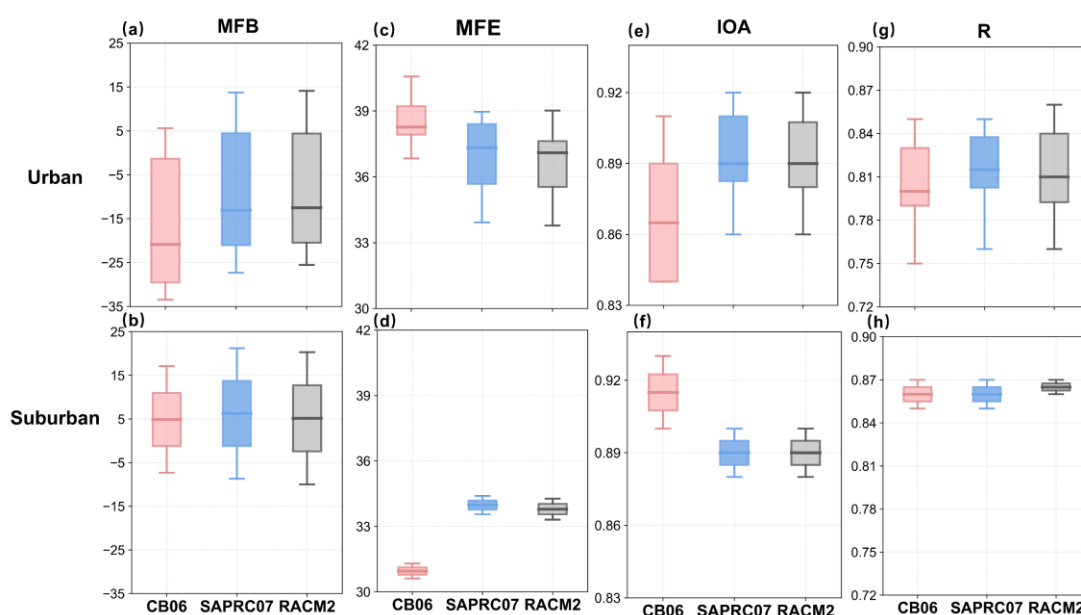
Figure 5 Statistical analysis of hourly O 3 simulated by three photochemical mechanisms (CB06, SAPRC07 and RACM2) s at urban sites and suburban sites across Chengdu region during August 9-August 18, 2019.
