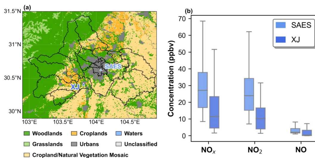
Figure 4 (a) Land use types in Chengdu and surrounding areas, along with the locations of the SAES site (light blue triangle) and XJ site (dark blue triangle). (b) Distribution of NO x (NO x = NO + NO 2 ), NO 2 and NO concentrations (ppbv) at the Sichuan Academy of Environmental Sciences (SAES) site and Xinjin (XJ) site during this pollution episode. The box plots present the 10th, 25th, 50th, 75th, and 90th percentiles of the statistical metrics individually.
