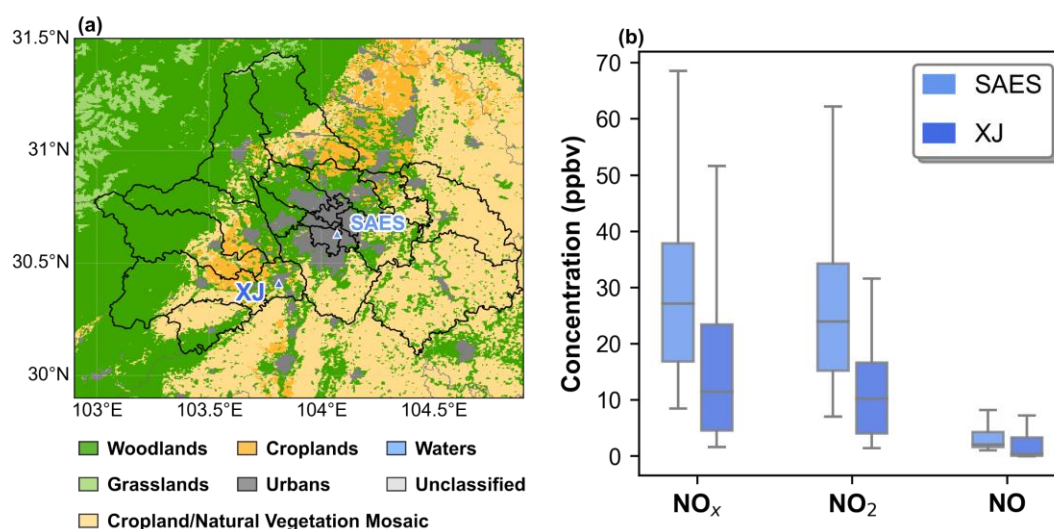
Figure 1 (a) Land use types in Chengdu and surrounding areas, along with the locations of the SAES site (light blue triangle) and XJ site (dark blue triangle). (b) Distribution of NO x (NO x = NO + NO 2 ), NO 2 and NO concentrations (ppbv) at the Sichuan Academy of Environmental Sciences (SAES) site and Xinjin (XJ) site during this pollution episode. The box plots present the 10th, 25th, 50th, 75th, and 90th percentiles of the statistical metrics individually.
