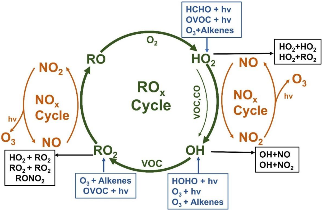
Figure S1 Schematic of simplified ozone formation mechanism and the coupling of the NO x and RO x radical cycle. The primary source reactions and the termination reactions of RO x radicals were shown in blue and black, respectively.
