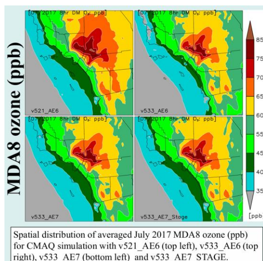
Response Figure 1. Spatial distribution of averaged July 2017 MDA8 ozone (ppb) for CMAQ with different aerosol module versions. Adapted from Kulkarni, S. (2021).
