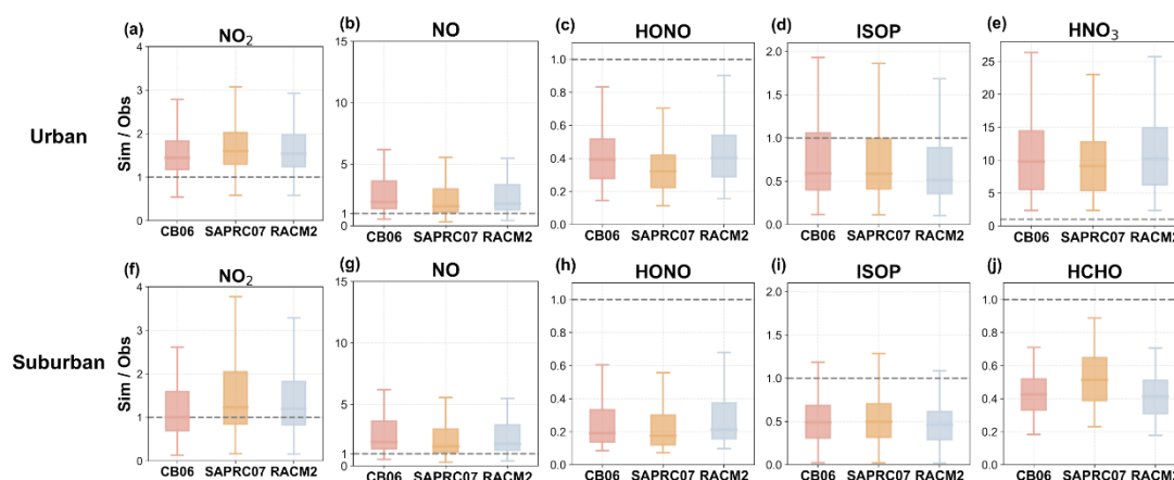
Figure 3 Comparison of three photochemical mechanisms on key photochemical species at urban site and suburban site. The box plots present the 10th, 25th, 50th, 75th, and 90th percentiles of the ratio of simulation value vs observation value (08:00-18:00 local time) individually.
