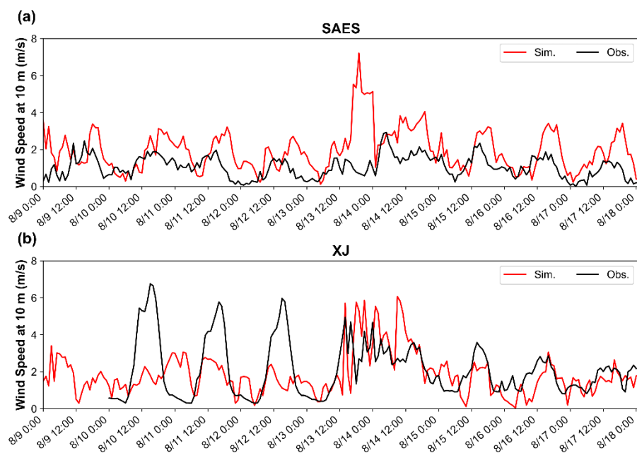
Figure S5 Time series of wind speed (m/s) at 10 m simulation (red lines) and observation (black lines) at SEAS (a) and XJ (b) sites.
