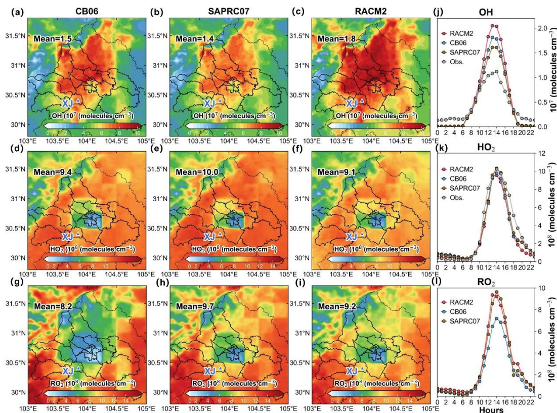
Figure 5 Regional distributions of OH, HO 2 and RO 2 radical concentration at 14:00 local time and diurnal variation at XJ site of OH, HO 2 and RO 2 concentration simulated by three photochemical mechanisms during August 9-August 18, 2019. The location of XJ site is marked with a dark blue triangle.
