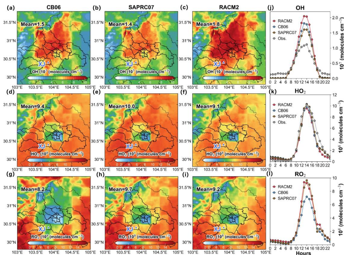
Figure 5 Regional distributions of OH, HO 2 and RO 2 concentration at 14:00 local time and diurnal variation at XJ site of OH, HO 2 and RO 2 concentration simulated by three photochemical mechanisms during August 9-August 18, 2019. The location of XJ site is marked with a dark blue triangle.
