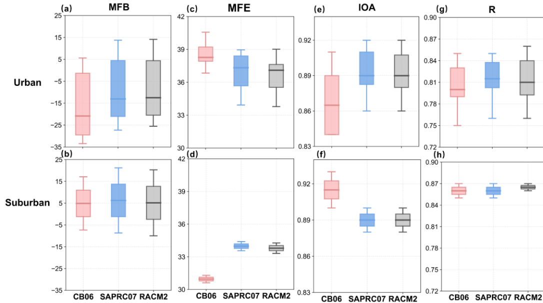
Figure 2 Statistical analysis of hourly O_3 simulated by three photochemical mechanisms (CB06, SAPRC07 and RACM2) s at urban sites and suburban sites across Chengdu region during August 9-August 18, 2019.
