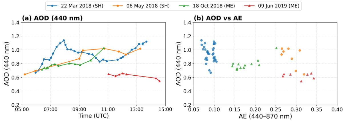
Figure S7: (a) Temporal evolution of AOD at 440 nm for four selected dust events (22 March 2018, 06 May 2018, 18 October 2018, and 09 June 2019). (b) Corresponding relationship between AOD_{440} and AE_{440-870} for the same events. 22 March 2018 (Saharan; blue circles), 06 May 2018 (Saharan; orange circles), 18 October 2018 (Middle Eastern; green triangles), and 09 June 2019 (Middle Eastern; red triangles).
