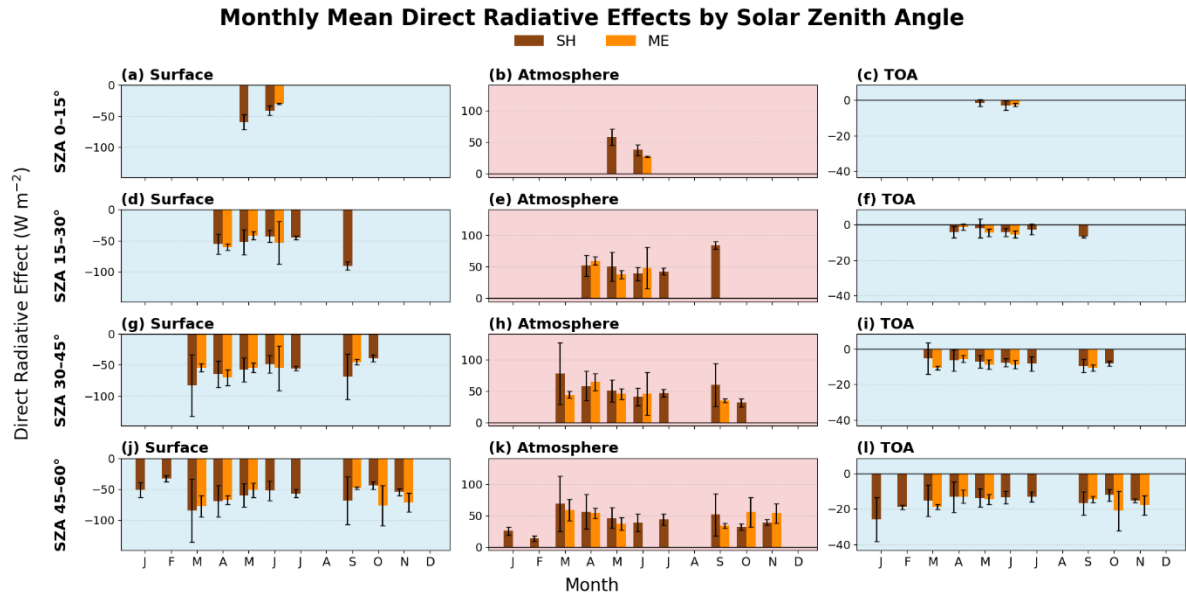
Figure S4: Monthly mean shortwave direct radiative effects (DRE; \text{W m}^{-2} ) over AMX during 2015–2022 under clear-sky conditions, classified into four solar zenith angle (SZA) intervals: 0–15°, 15–30°, 30–45°, and 45–60°. Results are shown for the surface (left column), atmosphere (middle column), and top of the atmosphere (TOA; right column). Saharan dust events are shown in brown and Middle Eastern dust events in orange. Bars represent monthly mean DRE values within each SZA interval, and error bars denote \pm 1 standard deviation, indicating the variability among the instantaneous observations included in each monthly mean. Background shading denotes cooling effects in blue and atmospheric heating in red.
