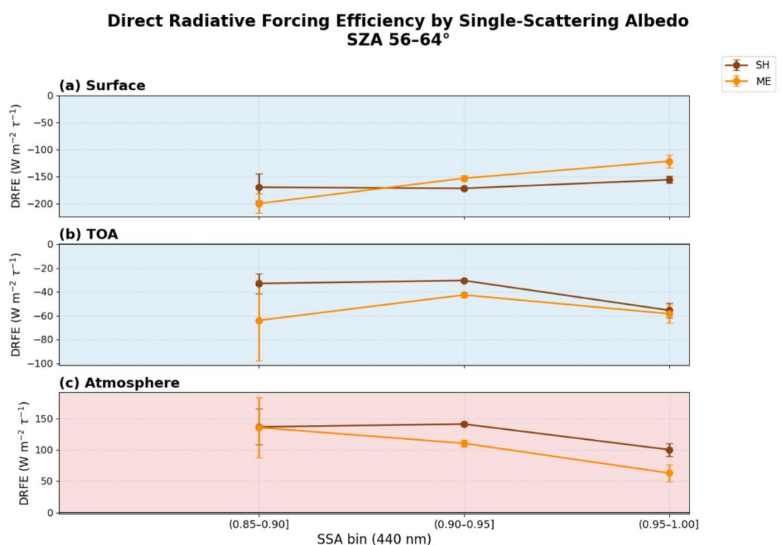
Figure S5: The DRFE (in \text{W m}^{-2} \tau^{-1} ) as a function of SSA at 440 nm for (a) surface, (b) TOA, and (c) atmosphere, for Saharan (brown) and Middle Eastern (orange) dust. Symbols represent mean values within SSA bins and error bars denote \pm 1\sigma . Background colors denote cooling (blue) and warming (red) effects.
