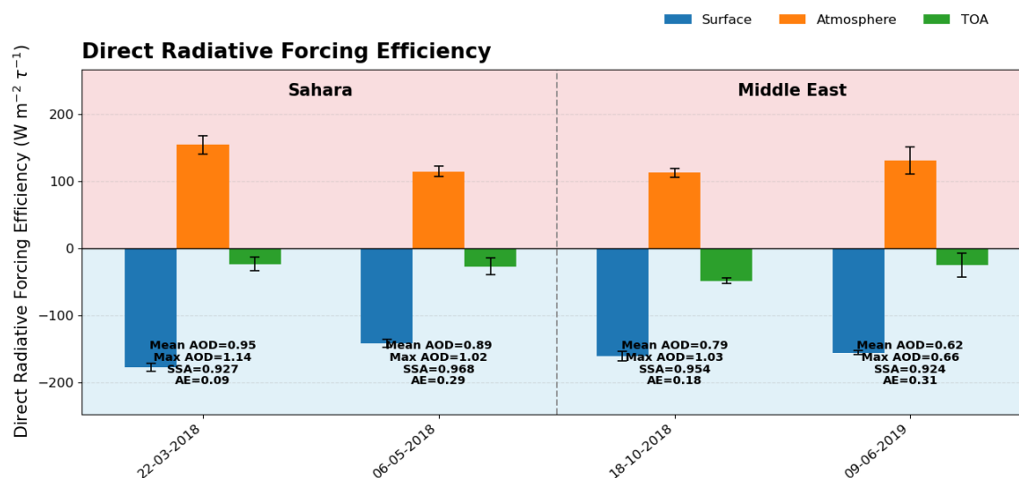
Figure S6: DRFE at the surface, within the atmosphere, and at the TOA for the selected four dust events.
