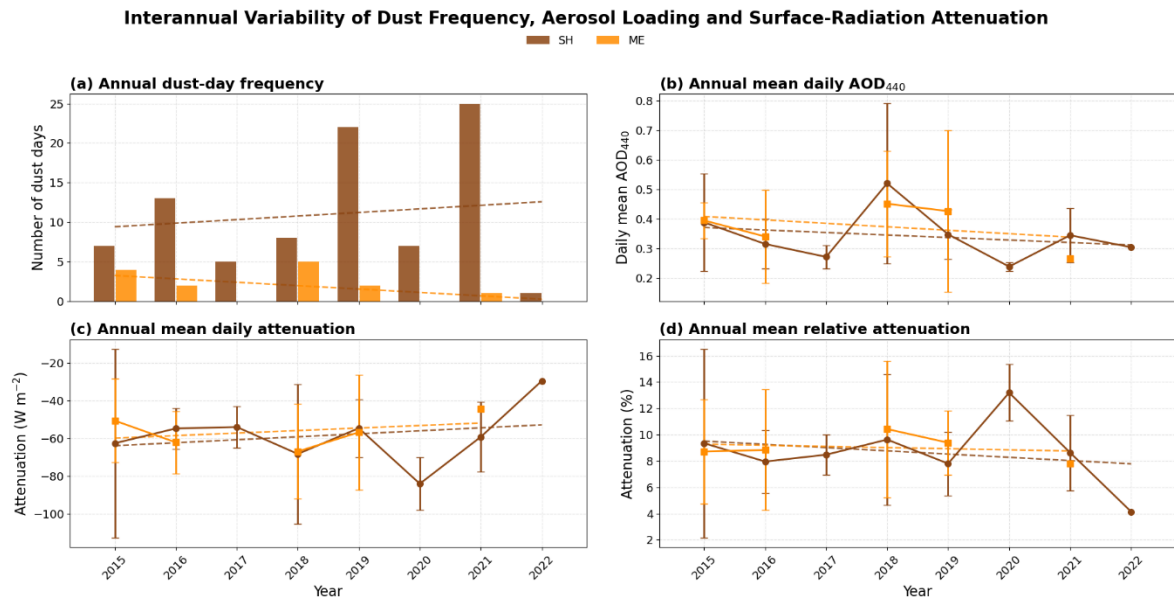
Figure S8: Interannual variability of (a) annual dust-day frequency, (b) annual mean daily AOD_{440} , (c) annual mean daily surface attenuation (DRE), and (d) annual mean relative attenuation (%) for Saharan (SH) and Middle Eastern (ME) dust over the study period (2015–2022). Error bars represent \pm 1 standard deviation. Dashed lines indicate linear trends.
