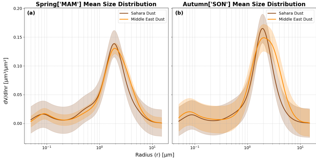
Figure S3: Mean volume size distributions for MAM (a) and SON (b) dust events, comparing Saharan (SH; brown) and Middle Eastern (ME; orange) dust layers during the study period 2015–2022. The shaded area denotes \pm 1 standard deviation.
