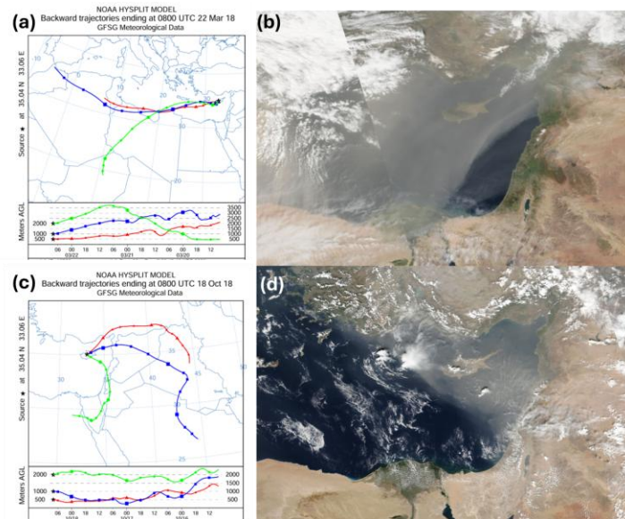
Figure 3: (a–b) Saharan dust event on 22 March 2018 and (c–d) Middle Eastern dust event on 18 October 2018 over Cyprus. Panels (a) and (c) show 72-hour backward air mass trajectories calculated using the NOAA Hybrid Single-Particle Lagrangian Integrated Trajectory (HYSPLIT) model with reanalysis meteorological data. Trajectories are presented for three arrival heights, indicated by red, green, and blue lines, revealing distinct source regions for each event. Panels (b) and (d) display corresponding MODIS satellite imagery (GIBS/Worldview), illustrating the spatial extent and transport of dust over the region during the two episodes.
