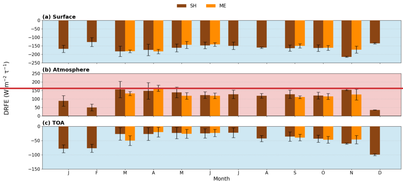
Figure 10: Monthly mean dust DRFE (in \text{W m}^{-2} \tau^{-1} ) over AMX (2015–2022) under clear-sky conditions for (a) surface, (b) within the atmosphere, and (c) TOA. Saharan dust events are shown in brown and Middle Eastern dust events in orange. Bars represent
