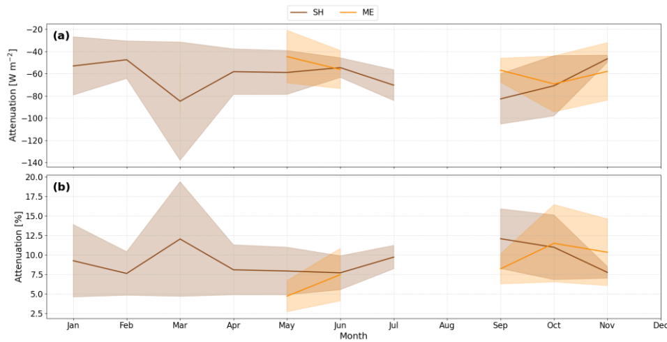
Figure 125: Seasonal variation in aerosol-induced attenuation of global horizontal irradiance (GHI) for Saharan (brown) and Middle Eastern (orange) dust events over Cyprus. (a) Monthly mean attenuation in absolute terms ( \text{W m}^{-2} ). (b) (%) Monthly mean attenuation. Shaded areas represent \pm 1 standard deviation, indicating interannual variability.
