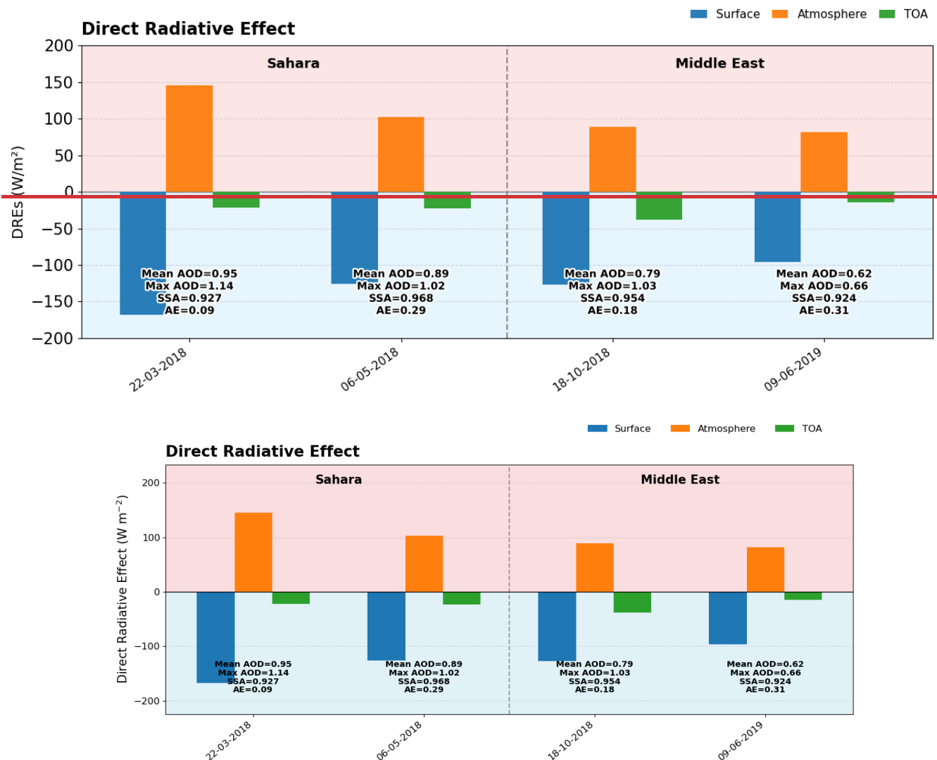
Figure 12: Daily mean DREs at the surface, within the atmosphere, and at the TOA for four selected dust events (22 March 2018, 06 May 2018, 18 October 2018, and 09 June 2019). Negative values indicate cooling (surface and TOA), while positive values represent atmospheric heating. Shaded regions highlight cooling (blue) and heating (red) regimes. Annotations provide mean and maximum AOD at 440 nm, along with SSA and Ångström exponent (AE) values for each case.
