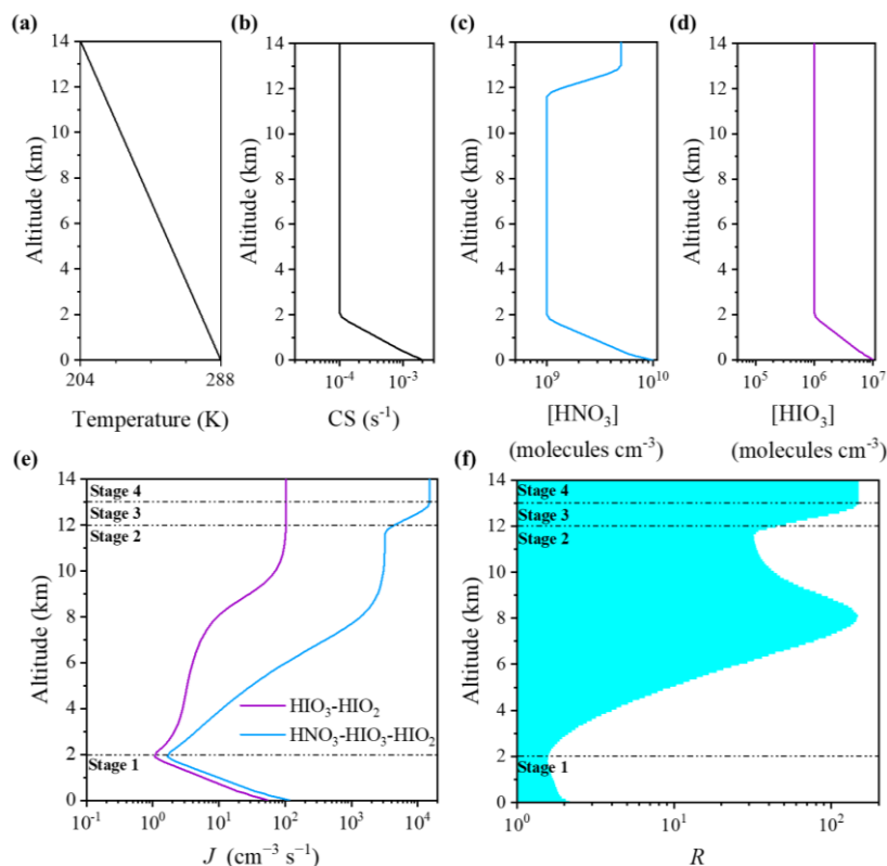
Figure 4. Altitude-dependent simulation inputs and the corresponding cluster formation rates ( J , cm -3 s -1 ). (a) Temperature; (b) CS; (c) \text{HNO}_3 concentration; and (d) \text{HIO}_3 concentration as functions of altitude. (e) J versus altitude for the \text{HIO}_3\text{-HIO}_2 (purple) and \text{HNO}_3\text{-HIO}_3\text{-HIO}_2 (blue) mechanisms. (f) R versus altitude.
