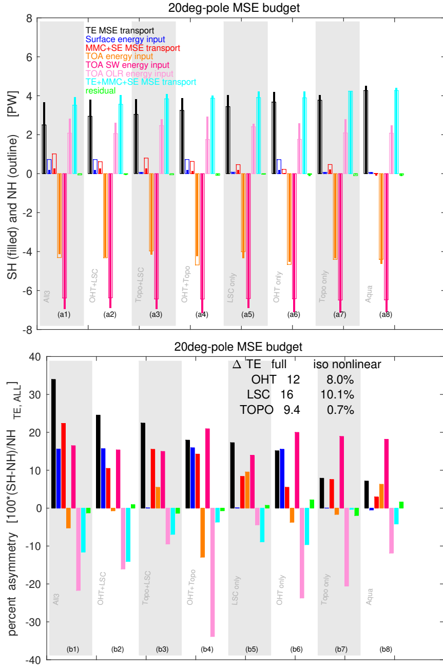
Figure 9. Moist static energy budget averaged from 20° to the pole (equation 2). In panel (a), we show each term for the SH (narrow filled bar) and NH (wide outline-only bar) separately, and in panel (b) the percent difference with the transient term in the NH taken in the denominator (e.g., the OLR percent difference is \frac{OLR_{SH} - OLR_{NH}}{TE_{NH}} ). For simplicity in our plots we lump together \Delta MMC with \Delta SE . Panel b also summarizes the NH vs. SH asymmetry in sub-monthly MSE flux in response to each surface inhomogeneity for both the isolated and full nonlinear responses. A similar figure but for the White et al. (2021) configuration is shown in Supplemental Figure S5.
