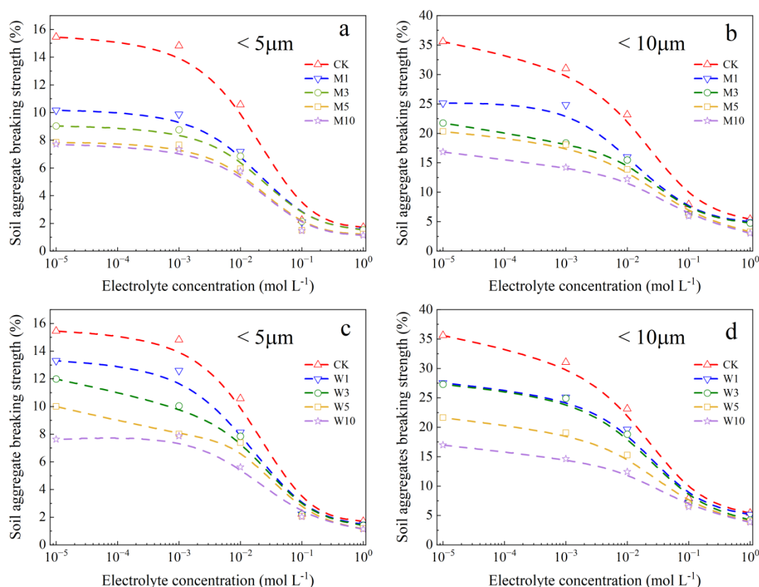
Fig. 8. Soil aggregate breaking strength (< 5 \mu m, < 10 \mu m) at different electrolyte
