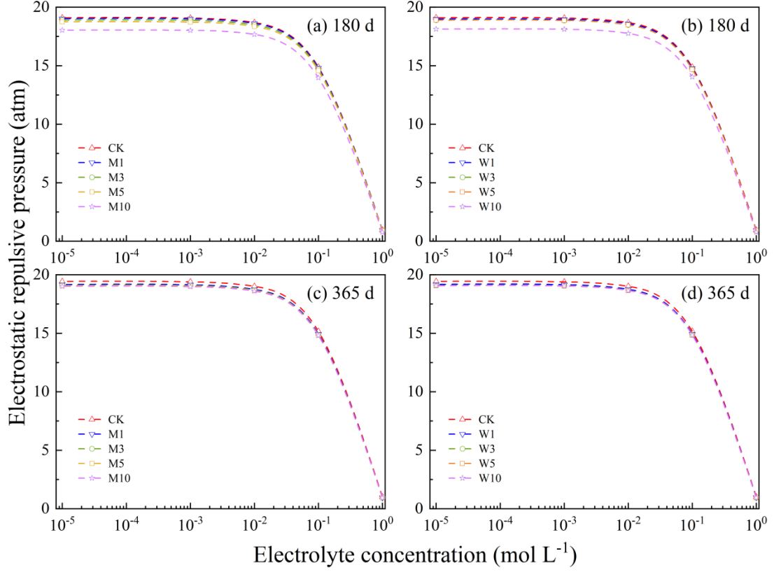
Fig. 5. Electrostatic repulsive pressure between soil particles at an interparticle distance of 2 nm under different electrolyte concentrations after 180 and 365 days.
