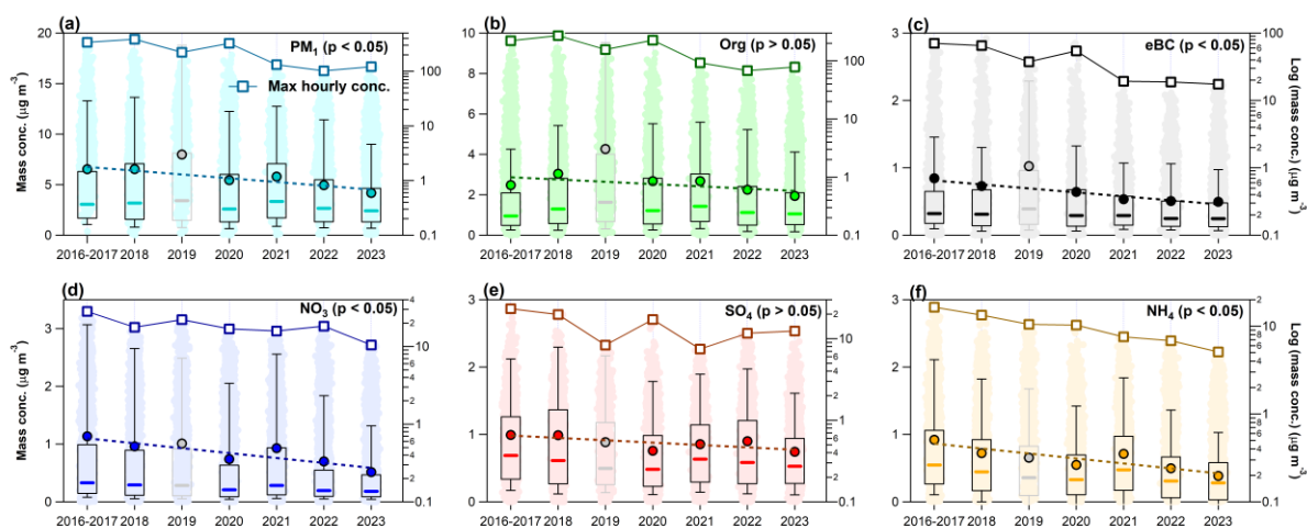
Figure 3. Box plots of annual average mass concentrations for (a) total PM 1 and major components: (b) OA, (c) eBC, (d) NO 3 , (e) SO 4 , and (f) NH 4 , based on long-term observations in Dublin (2016-2023). Light-colored dots in each annual bin represent all hourly data points from that year. Box plots show the mean (circle), median (horizontal line), 25 th -75 th percentiles (box), and 10 th -90 th percentiles (whiskers). Lines with square markers show annual hourly maximum concentrations (right axis, log-scale for clarity). Please note that 2019 is excluded from long-term trend analysis and is shown in grey due to biased data coverage (Fig. S3). The dashed line represents the linear fit of annual average concentrations with 2019 excluded, and the statistical significance of the trends is also shown.
