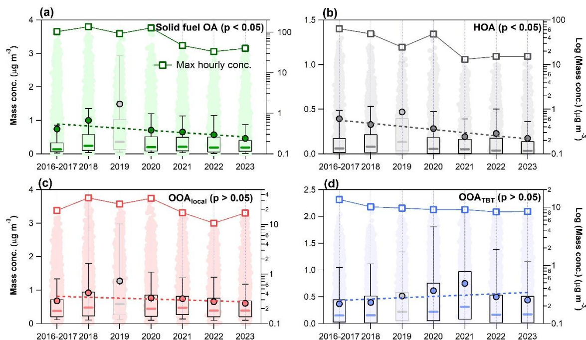
Figure 4. Box plots of annual average mass concentrations for OA factors, including (a) Solid fuel OA, (b) HOA, (c) OOA local and (d) OOA TBT , based on long-term observations in Dublin (2016-2023). Light-colored dots in each annual bin represent all hourly data points from that year. Box plots show the mean (circle), median (horizontal line), 25 th -75 th percentiles (box), and 10 th -90 th percentiles (whiskers). Lines with square markers show annual hourly maximum concentrations (right axis, log-scale for clarity). Please note that 2019 is excluded from long-term trend analysis and is shown in grey due to biased data coverage. The dashed line represents the linear fit of annual average concentrations with 2019 excluded, and the statistical significance of the trends is also shown in Table 1 .
