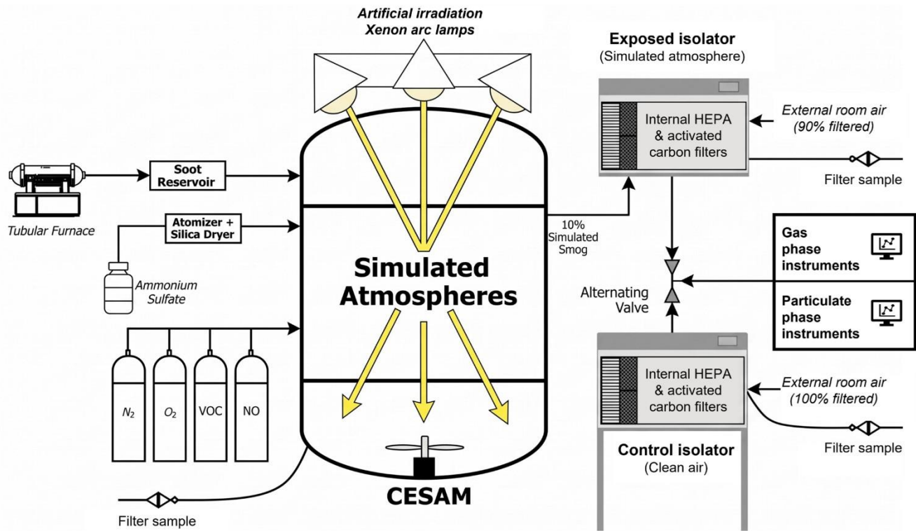
75 Figure 1: Schematic diagram of the PolluRisk experimental platform, illustrating the CESAM atmospheric simulation chamber equipped with a Xenon lamp irradiation system, two isolators for mice exposure (the exposure isolator receiving 90% filtered laboratory air using HEPA and activated carbon filters and 10% simulated air in CESAM, and the reference isolator receiving 100% of filtered room air), and the multi-instrument analytical set for pollutant characterization.
