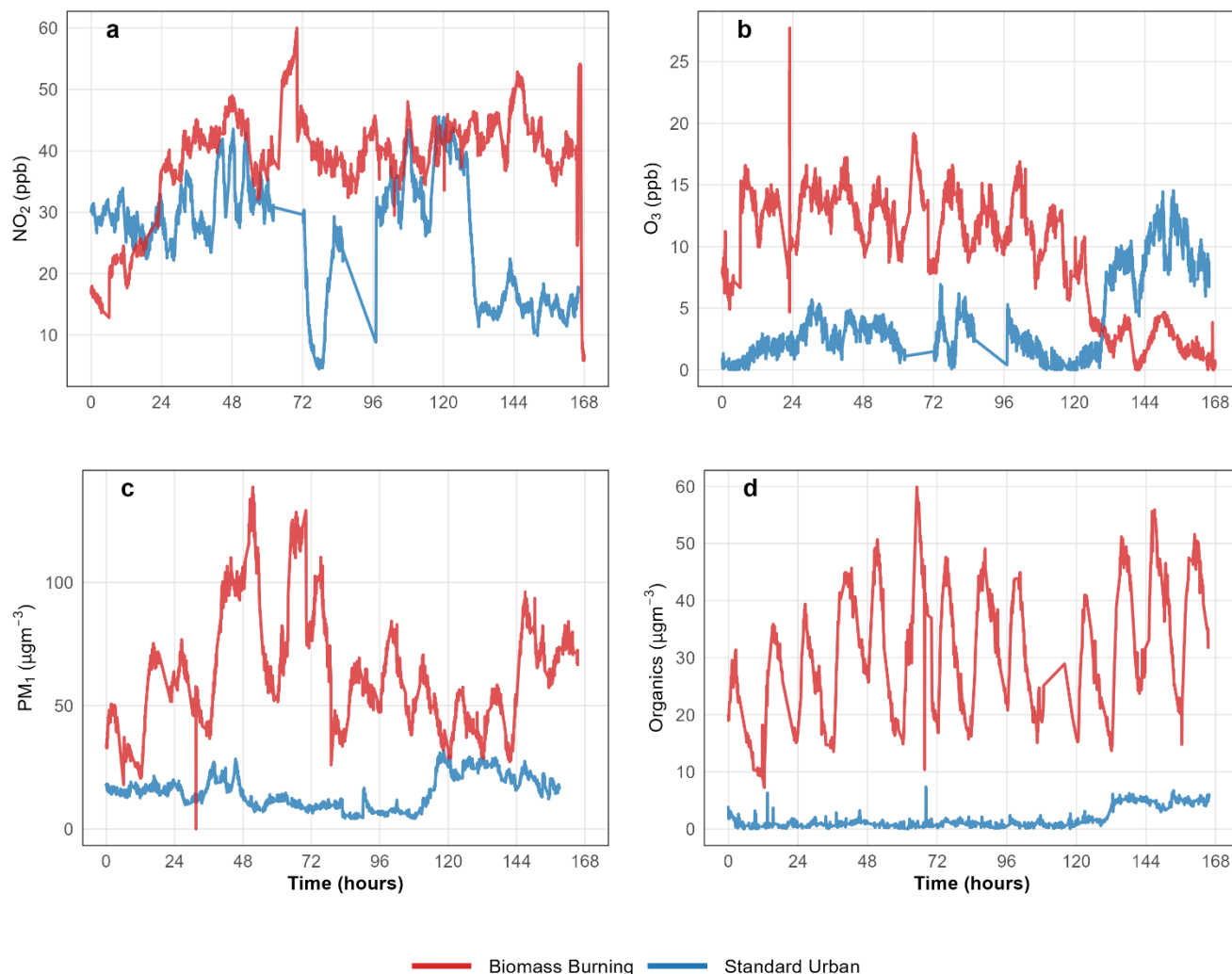
Figure 3: Temporal evolution of key pollutants during standard urban (blue) and biomass burning enhanced (red) exposure experiments: (a) NO 2 , (b) O 3 , (c) PM 1 concentrations, and (d) organic aerosol mass.
