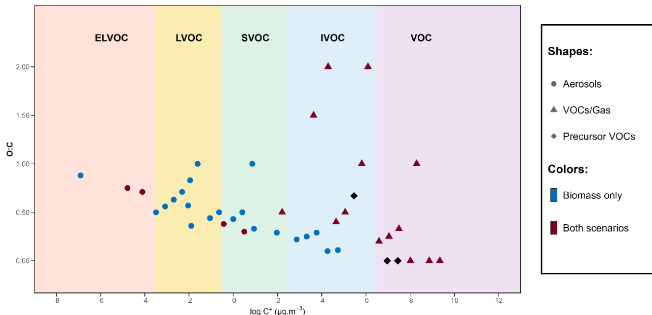
315 Figure 5: Molecular characterization of organic compounds identified in gas and aerosol phases, displayed as oxygen-to-carbon (O/C) ratios versus estimated volatilities (expressed as logarithm of saturation mass concentrations, C^* ). Colour coding indicates compound volatilities, with blue symbols representing compounds detected in biomass burning enhanced scenario only and dark red symbols indicating compounds detected in both atmospheric scenarios. Diamond symbols (◆) indicate precursor VOCs initially injected into CESAM, circles (●) represent compounds detected by UPLC/ESI-IMS-QTOFMS, and triangles (▲) indicate 320 compounds detected by PTR-TOF-MS.
