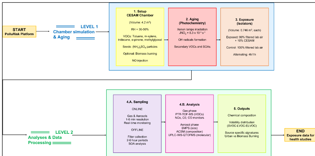
210 Figure 2: Complete experimental workflow. Two-sequence workflow: chamber simulation and aging processes, followed by analytical procedures and data processing. Colour coding: yellow = setup phase, red = photochemical aging, orange = exposure conditions, purple = sampling/analysis, green = final outputs. Flow direction: horizontal arrows indicate sequential progression, vertical arrow shows transition from chamber to analytical levels. END indicates completion of exposure protocol for health studies.
