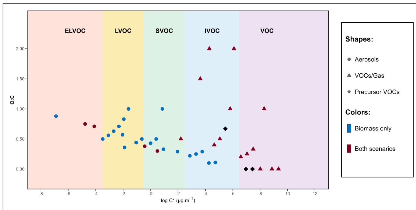
315 Figure 5: Molecular characterization of organic compounds identified in gas and aerosol phases, displayed as oxygen-to-carbon (O/C) ratios versus estimated volatilities (expressed as logarithm of saturation mass concentrations, C^* ). Colour coding indicates compound volatilities, with blue symbols representing compounds detected in biomass burning enhanced scenario only and dark red symbols indicating compounds detected in both atmospheric scenarios. Diamond symbols (◆) indicate precursor VOCs initially injected into CESAM, circles (●) represent compounds detected by UPLC/ESI-IMS-QTOFMS, and triangles (▲) indicate 320 compounds detected by PTR-TOF-MS.
