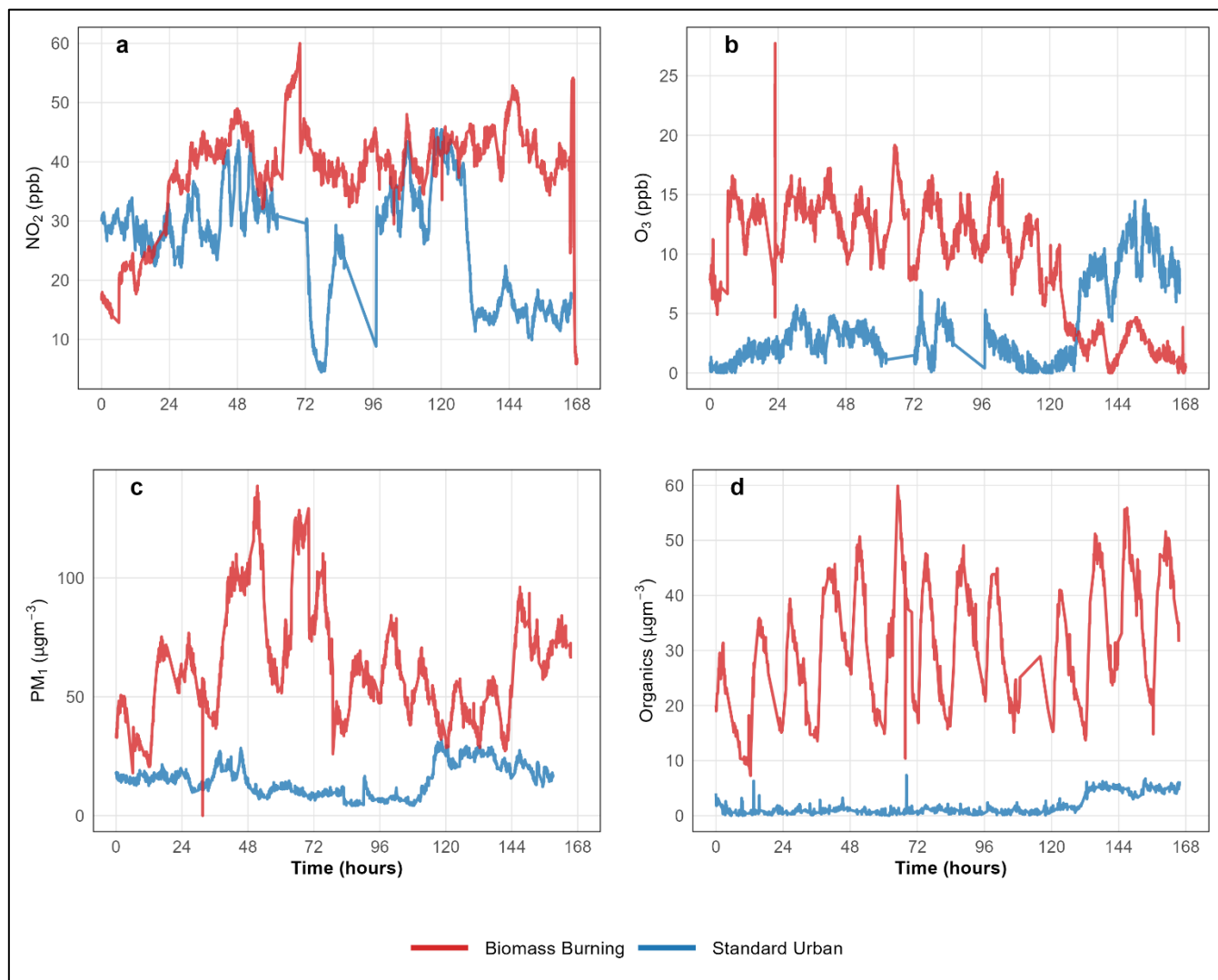
220 Figure 3: Temporal evolution of key pollutants during standard urban (blue) and biomass burning enhanced (red) exposure 225 experiments: (a) NO 2 , (b) O 3 , (c) PM 1 concentrations, and (d) organic aerosol mass.
