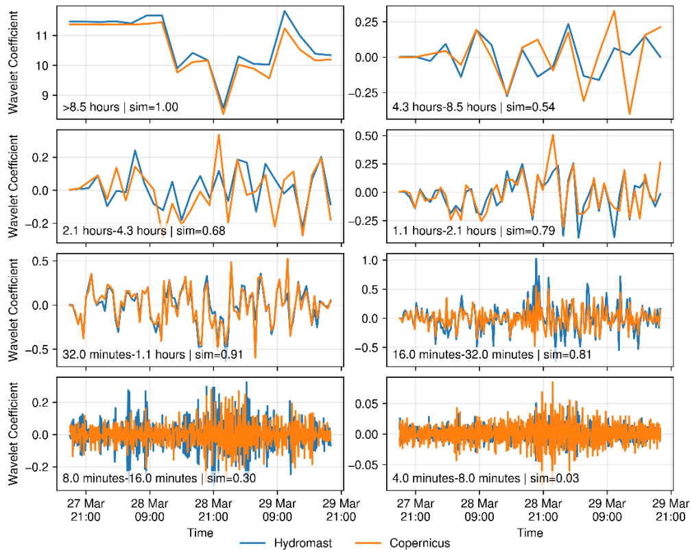
Figure 9. Anatomy of the high-current-speed event from 27 to 29 March, based on 8 frequency bands shown in the sub-figure legends, identified by wavelet analysis. Shown are the results for Stn. 0 (Copernicus) and Stn. 1 (Hydromast), “sim” presents the similarity between the wavelet coefficients in these two stations.
