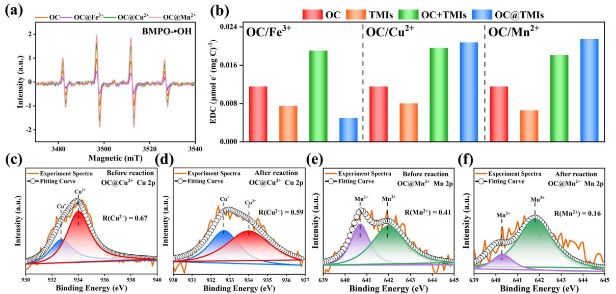
Figure 4. (a) BMPO-•OH adduct EPR spectra of OC, OC@Fe 3+ , OC@Cu 2+ and OC@Mn 2+ under irradiation. (b) Electron donating capacity (EDC) of OC, TMIs, OC+TMIs and OC@TMIs (For OC+TMIs, EDC was the arithmetic sum of that measured for OC and TMIs in separate experiments). High-resolution XPS spectra of Cu 2p for OC@Cu 2+ (c) before and
