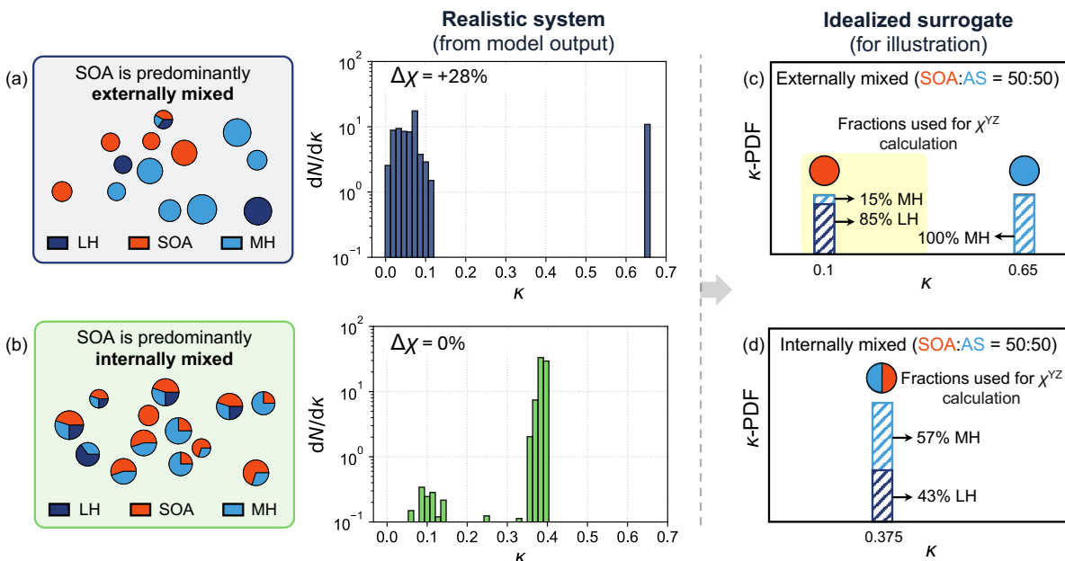
Figure 3. (a and b) The Representative PartMC-derived \kappa -PDFs of from the validation scenario library for two high-SOA (aerosol populations with high secondary organic aerosol (SOA) content aerosol populations at a dry diameter of 150 nm from the validation scenario library, corresponding to predominantly externally mixed (a) and internally mixed (b) particle populations. Note that y-axes are in logarithmic scale. (c and d) Schematic diagrams of simplified-idealized surrogate cases with identical bulk compositions of 50% SOA and 50% ammonium sulfate (AS).
