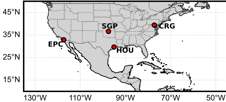
Figure 5. Map of ARM sites with long-term HTDMA measurements: Baltimore, MD (CRG); La Jolla, CA (EPC); Houston, TX (HOU); and Southern Great Plains, OK (SGP).
