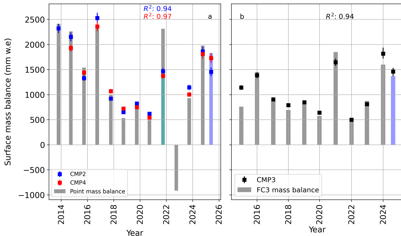
Figure A2. Identification of annual layers by comparing estimated SWE from three CMP gathers across the accumulation area of the Grosser Aletschgletscher with the measured SWE from point mass-balance measurements (Fig. 1). Blue squares represent the identified annual layers from CMP2 (lower part of Ewigschneefeld, a), the red square, CMP4 near the point mass-balance measurement (Jungfraufirn), and the black square, CMP3 (upper part of Ewigschneefeld, b). The y-axis shows the annual surface mass balance in mm w.e, and the x-axis shows the year. The blue vertical bar shows the winter accumulation in 2025, and the cyan vertical bar in 2021 represents the remaining firn layer after the complete removal of the 2022 winter and some part of the 2021 layer (nearly 1000 mm w.e) at the point mass balance measurement location (Stake in Fig 1).
