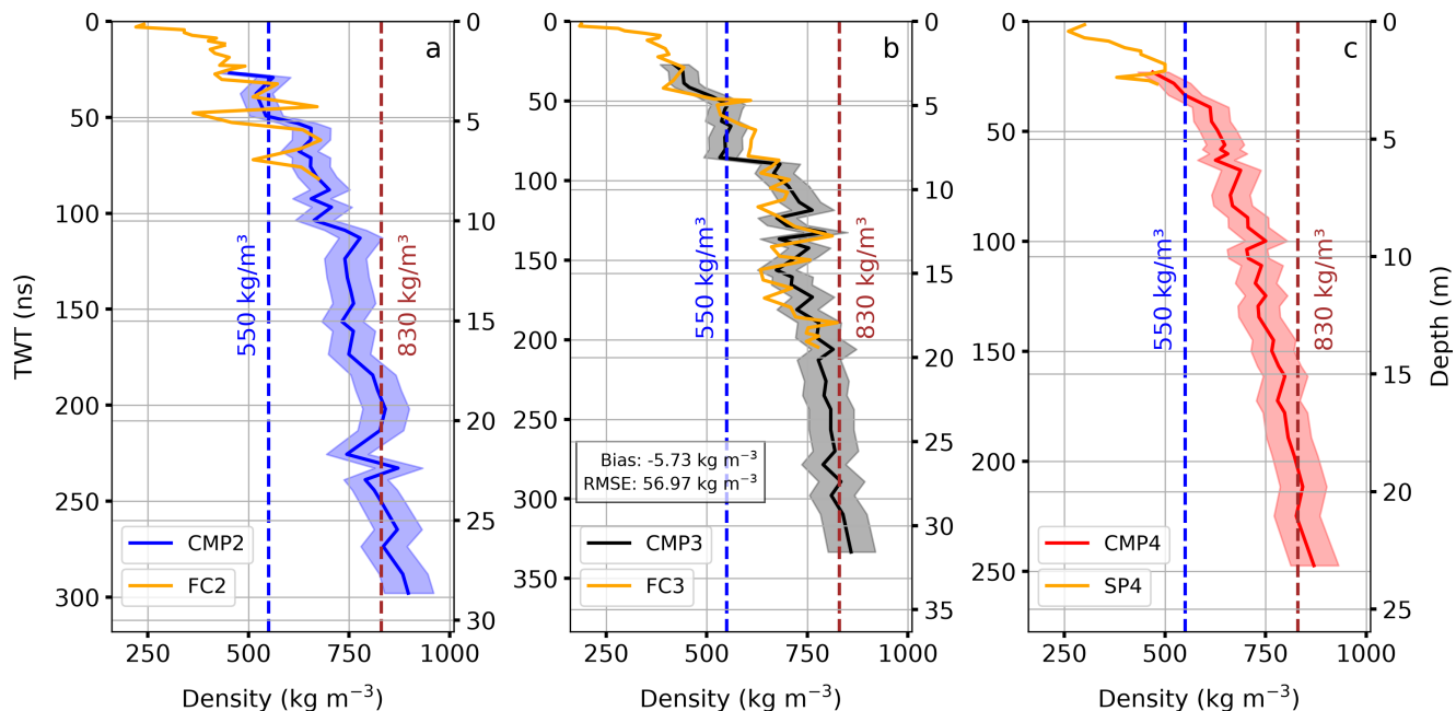
Figure 8. Firn density-depth profiles estimated from the CMP gather acquired in winter 2025 at the accumulation area of the Grosse Aletschgletscher (black crosses in Fig. 1). The figure also shows firn density-depth profiles obtained from firn cores (FC2 and FC3) and a snow pit (SP4) near each corresponding CMP measurement location (orange line in each subplot). The blue line (panel a) shows the CMP-derived (CMP2) firn density-depth profile from the lower part of the Ewigschneefeld, the black line (panel b) is obtained from the upper part of the Ewigschneefeld, and the red line (panel c) shows the density-depth profile near the long-term mass balance measurement location (Jungfraufirn, Fig. 1). The uncertainty range is shown in corresponding shaded colours. The dotted blue and brown lines depict the depth to firn and pore close-off density. The left and right y-axes demonstrate the radar two-way travel time (TWT) in ns and depth in meters corrected for each of the CMP locations after the Dix equation (Eq. 2), respectively.
