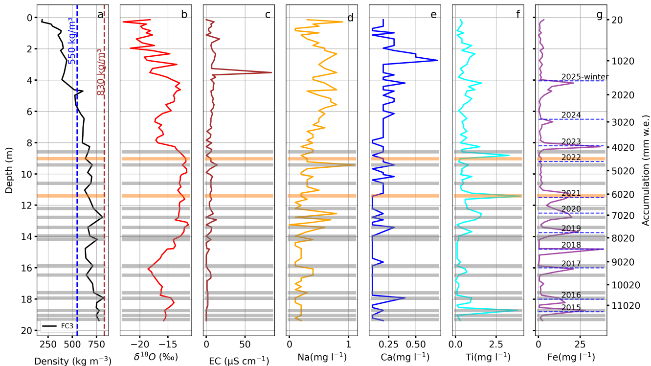
Figure 6. Illustration of depth distribution of different parameters in the firm core (a) density, (b) stable water isotope, (c) electrical conductivity, and the lab analysis of the major ions and chemical impurity concentration ( \text{mg l}^{-1} ) with depth, such as Na (orange, d), Ca (blue, e), Ti (cyan, f), and Fe (purple, g) for FC3 at the upper Ewigschneefeld. The firm and pore close-off densities are indicated by dotted blue and brown vertical lines, respectively (a). Grey horizontal bars represent visually identified ice lenses, whereas orange horizontal bars depict visible Sahara dust events. The highlighted dashed blue lines (g) indicate the identified annual layers. The right y-axis shows the bulk accumulation estimated from the firm core data. The thickness of all ice lenses and the visible Sahara dust layer is not to scale.
