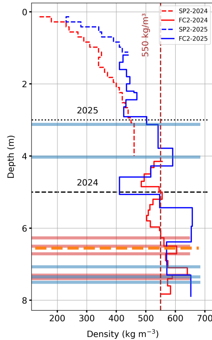
Figure 7. Comparison of firm density-depth derived from the 2024 and 2025 winter glaciological measurements (shallow firm cores, FC2 in Fig. 1) at the lower part of Ewigschneefeld. The dashed red and blue vertical lines refer to the density profiles from the snow pit, whereas the solid red and blue lines illustrate density-depth profiles derived from the firm core starting at the bottom of the respective snow pits. The horizontal lines shown here are identified ice lenses from the snow and firm cores corresponding to the coloured lines. The visible Sahara dust layer is depicted by a horizontal dashed orange line, identified from the firm core collected during the 2025 measurements. The black dashed-and-dotted horizontal layer represents the 2025 and 2024 winter accumulations in meters of depth, respectively. The legend at the top-right corner of the figure shows the years and corresponding glaciological measurements. The depth axis (y-axis) is plotted as a reference surface for the respective 2025 and 2024 shallow firm core results.
